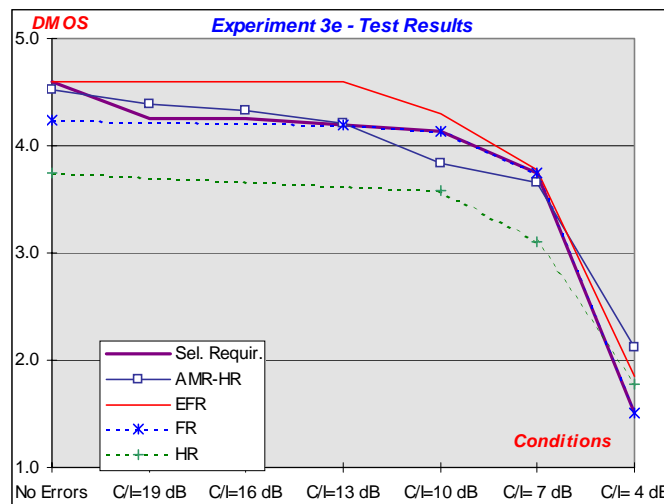
Figure 6.5: AMR performance curves for Experiment 3e (Half rate with Car Noise)
