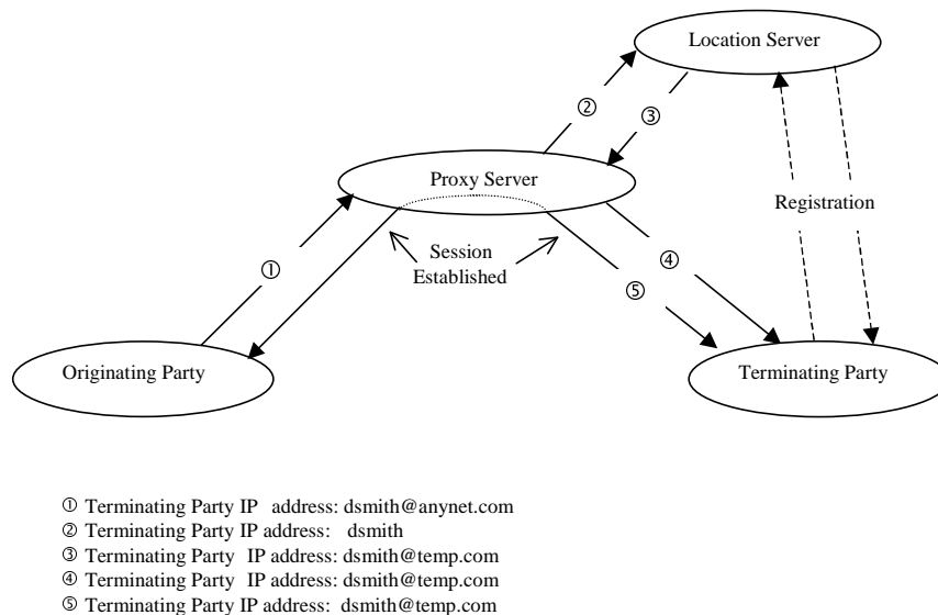
Figure 18: Session Establishment Using a Proxy Server
