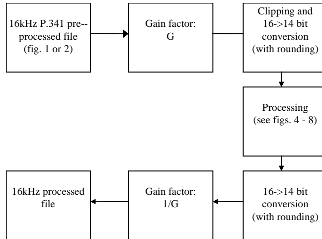
Figure 3: Rounding and scaling for wideband conditions.
