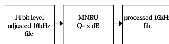
Figure 7: Processing of speech by wideband MNRU.
