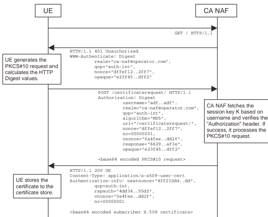
Figure 2: Certificate request using PKCS#10 with HTTP Digest Authentication.
