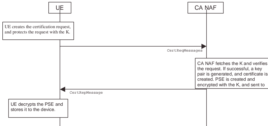
Figure 4: Certificate request using centralized scheme of CMP.
