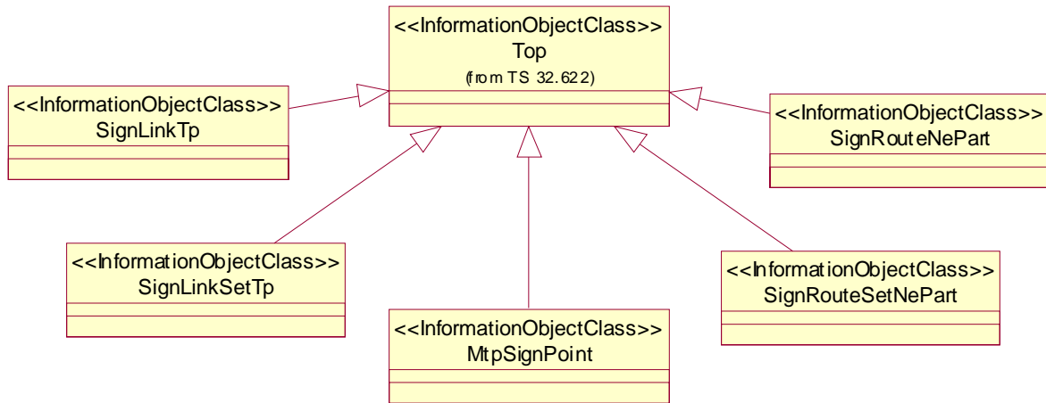
Signalling Transport Network NRM Inheritance Hierarchy
