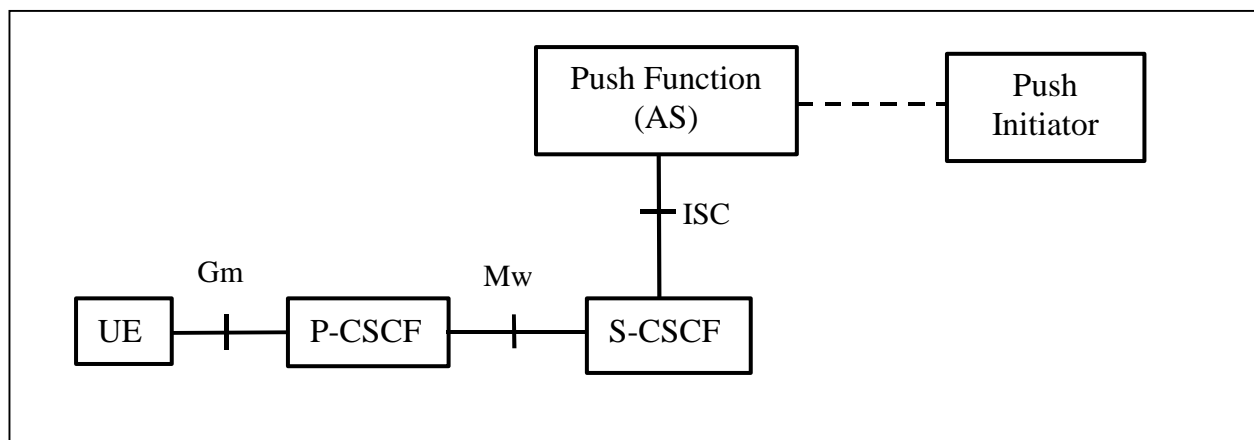
Figure 11: Network Elements and Interfaces supporting Push over IMS.
