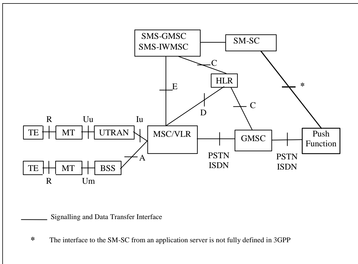
Figure 10. Network Elements and Interfaces supporting Push over the CS Domain (circuit connection and SMS).
