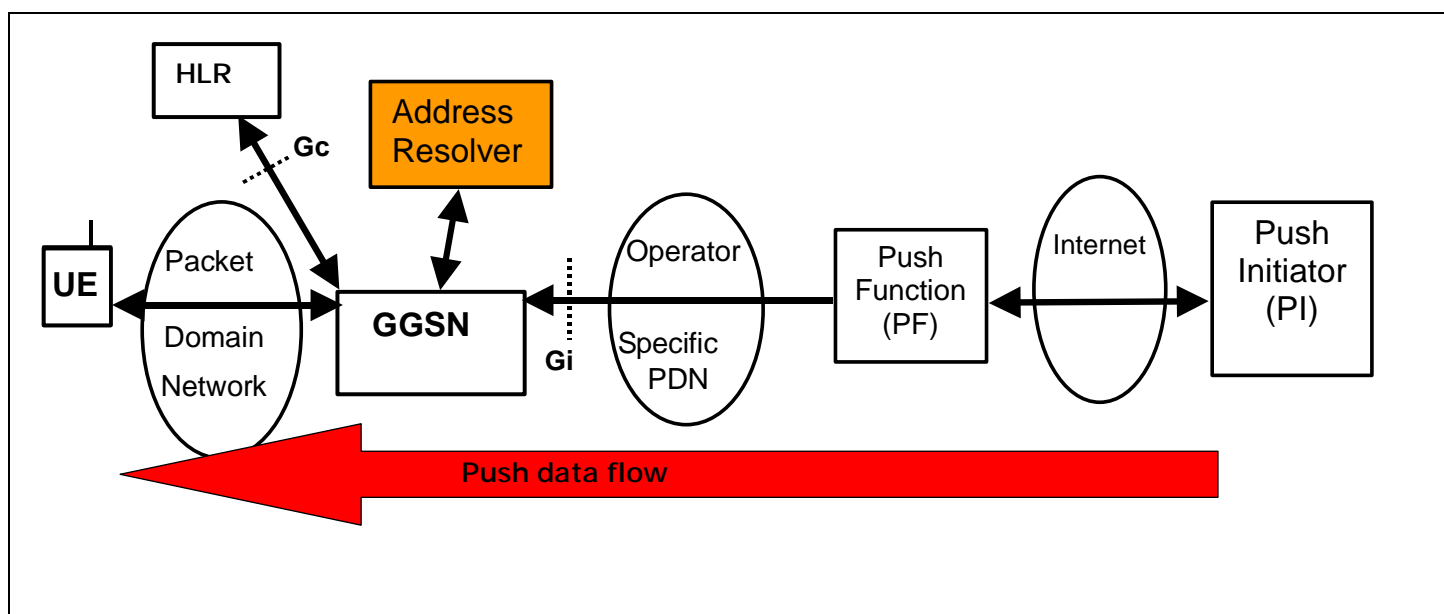
Figure B1. Architecture for NRPCA with Dynamic IP Addressing supporting Push
