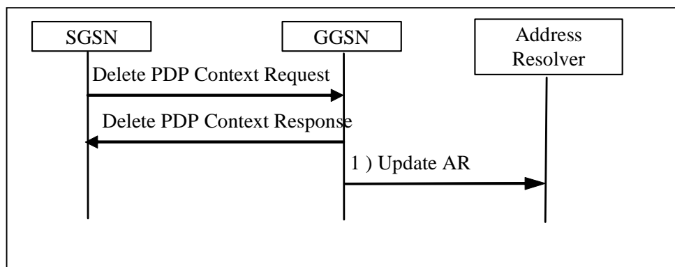
Figure 8: Deactivate of PDP Context and Update Address Resolver (at home GGSN)
