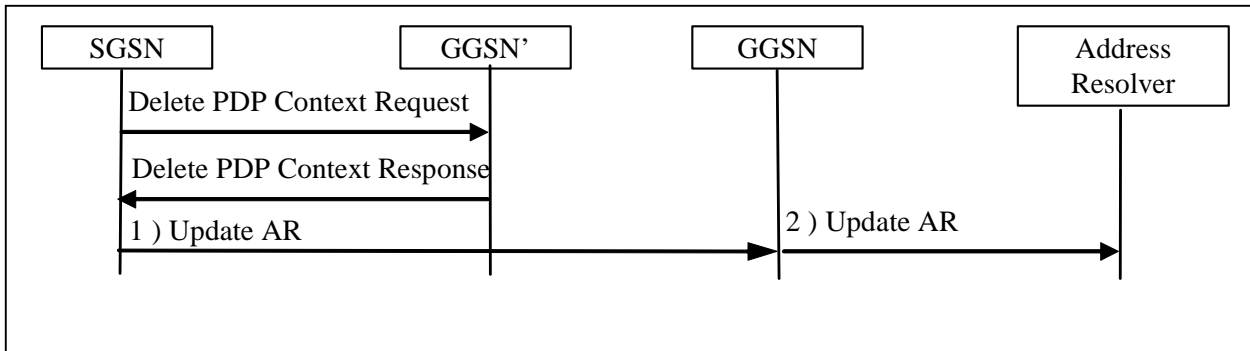
Figure B3: Deactivate of PDP Context and Update Address Resolver (when PDP Context is at the visited GGSN)
