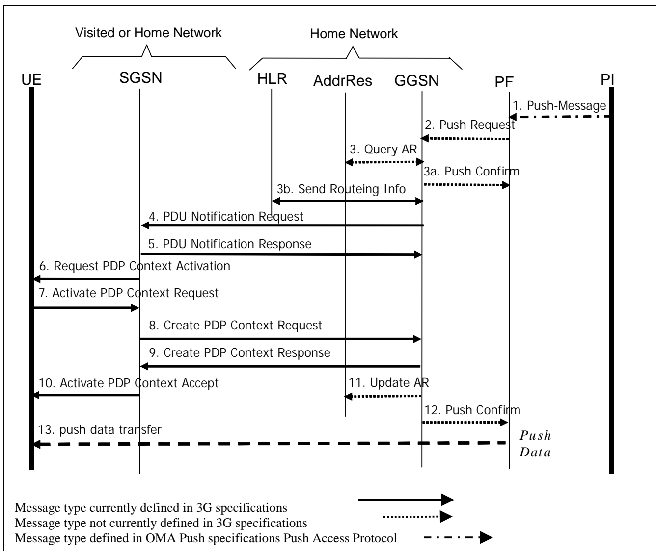
Figure 7. NRPCA using Dynamic IP Address Assignment (one APN per GGSN)
