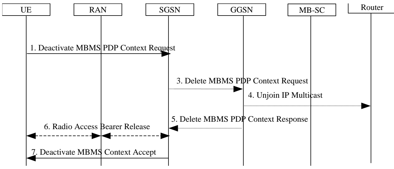
Figure 57: MS Initiated Multicast service deactivation
