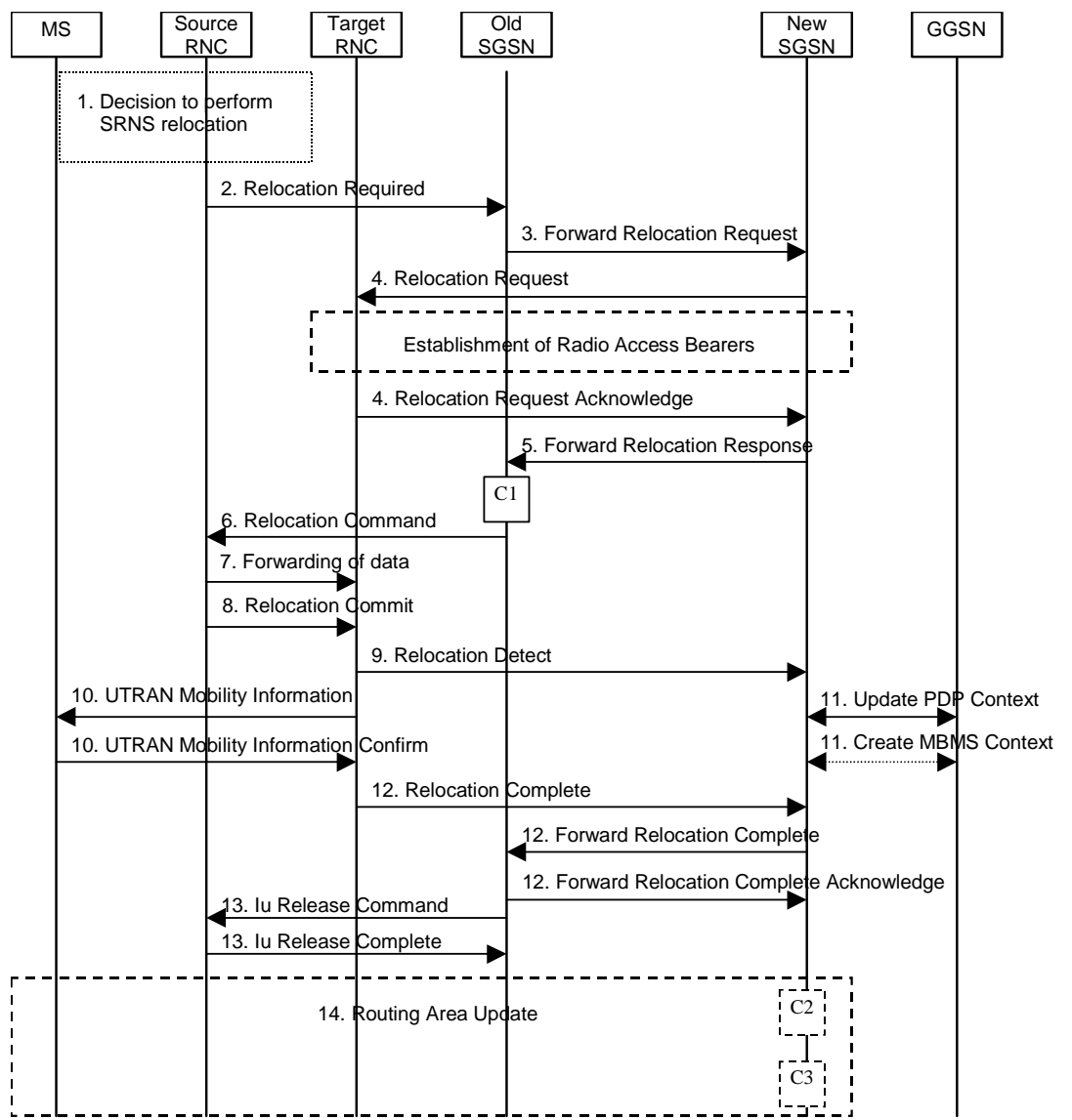
Figure 45: SRNS Relocation Procedure
