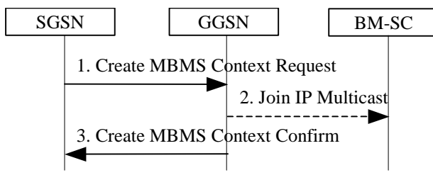
Figure 43: The activation of an MBMS broadcast service
