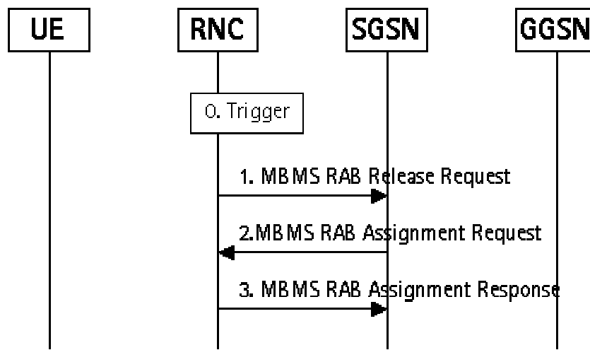
Figure 46 MBMS RAB release
