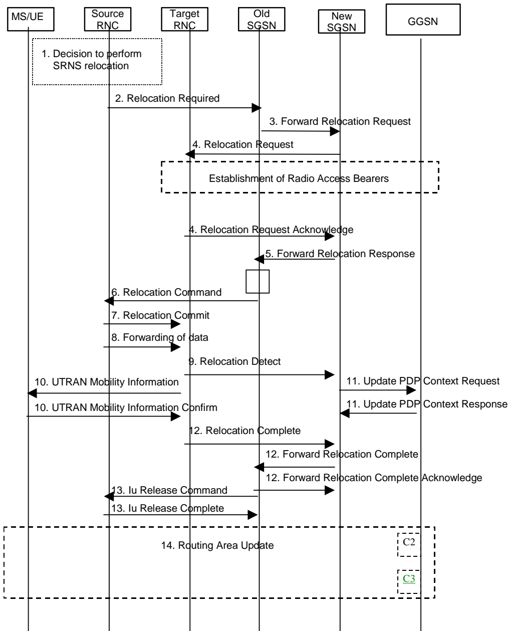
Figure 70: Serving SRNS Relocation Procedure
