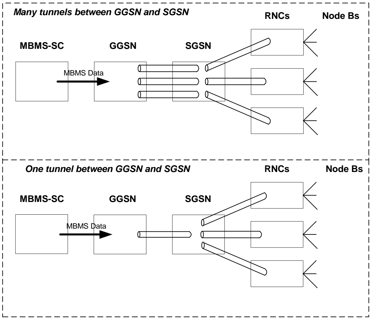
Figure 78. Many tunnels between GGSN and SGSN vs. One tunnel between GGSN and SGSN.
