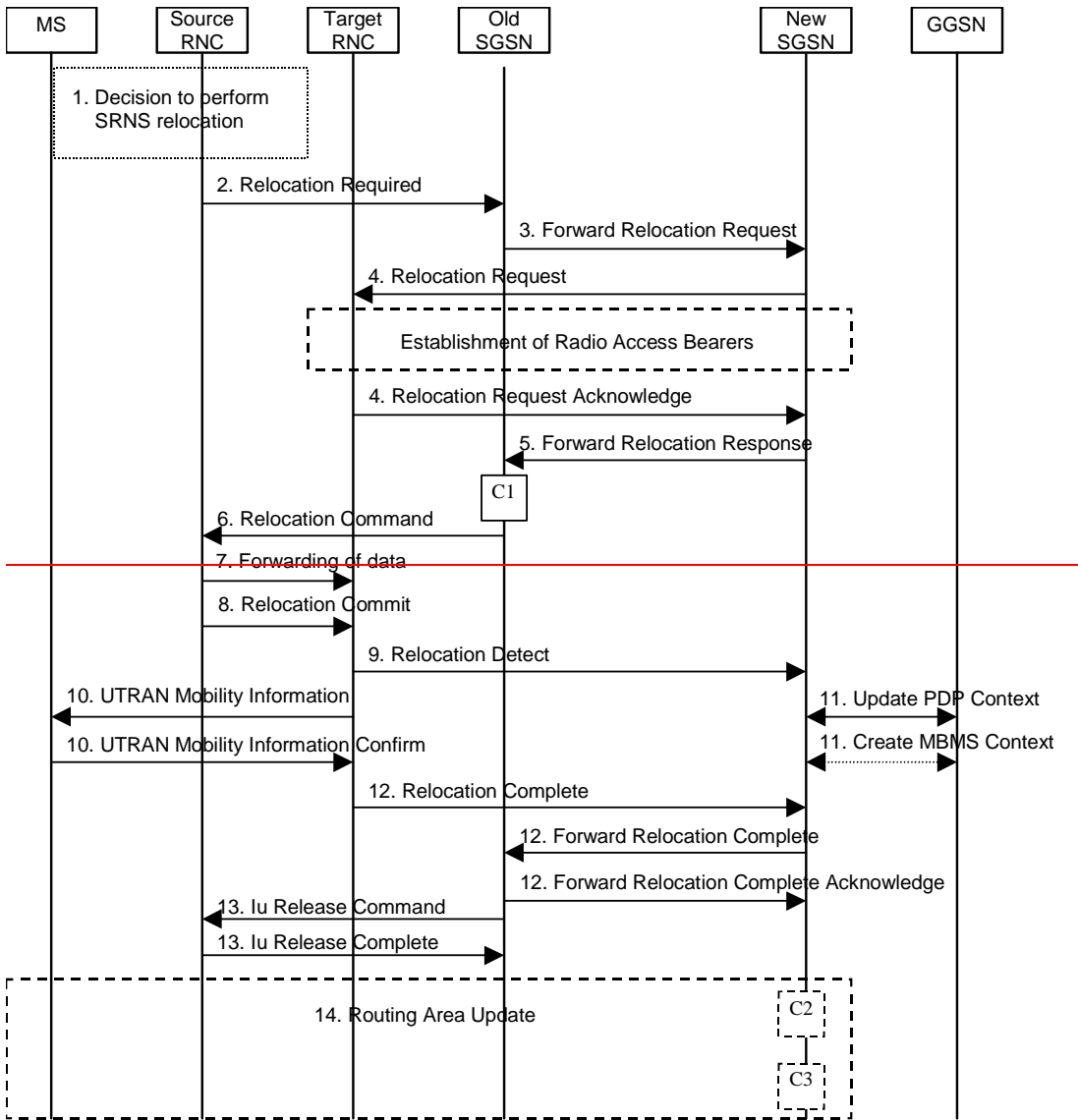
Figure 15.: SRNS Relocation Procedure
