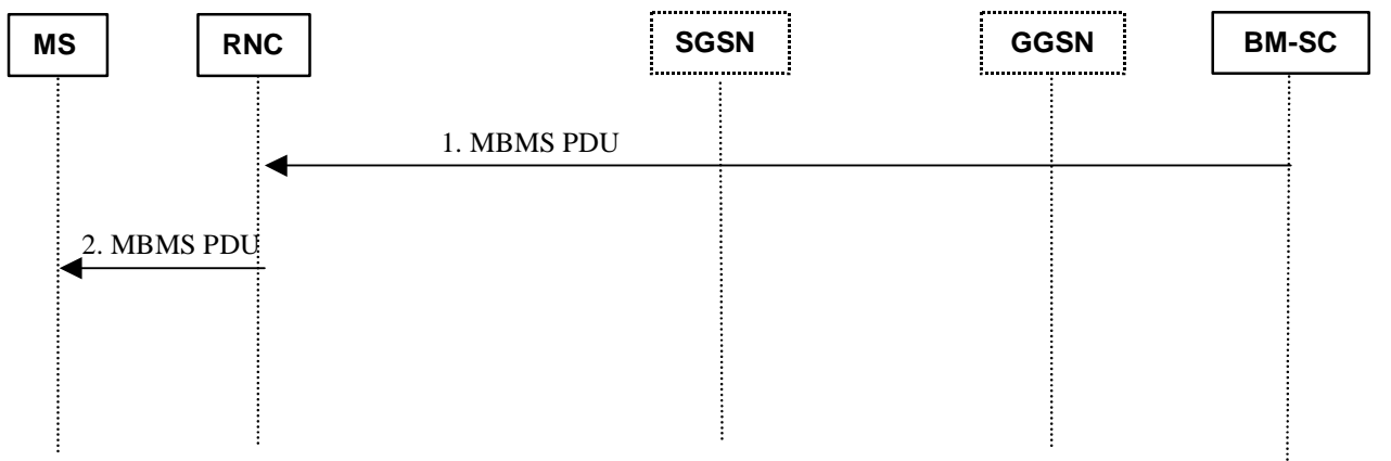
Figure 63: Broadcast service data transfer
