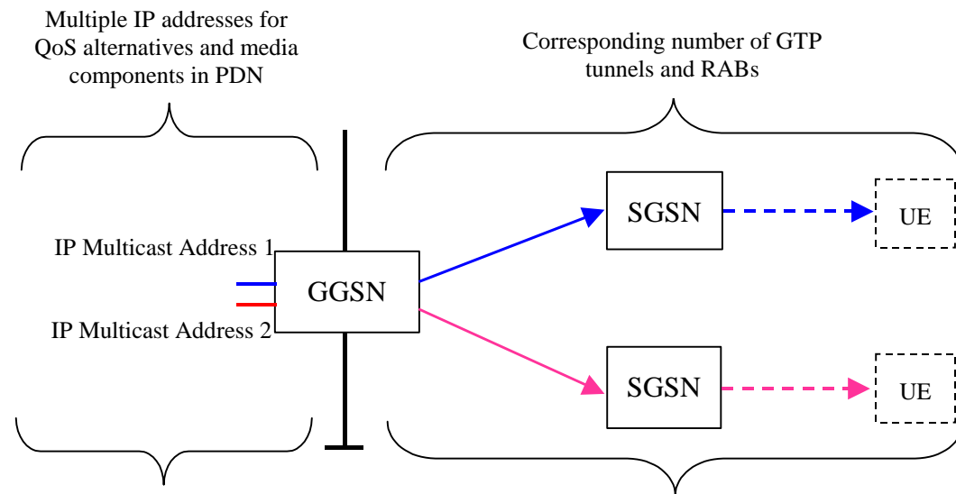
Figure 33: Example of data flow for multiple QoS profiles of an MBMS transmission
