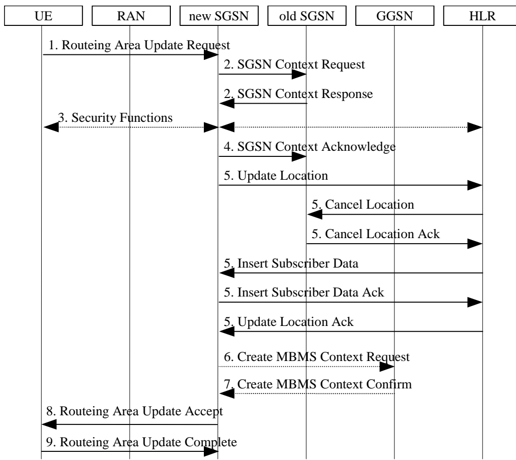
Figure 44: Mobility between SGSNs
