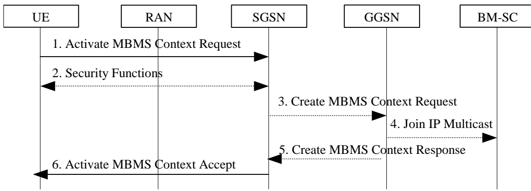
Figure 34. The activation of an MBMS multicast service
