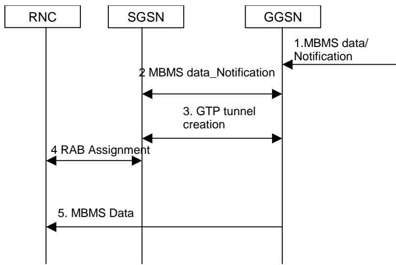
Figure 68: MBMS Bearer Path set-up when Iu-Flex is not configured
