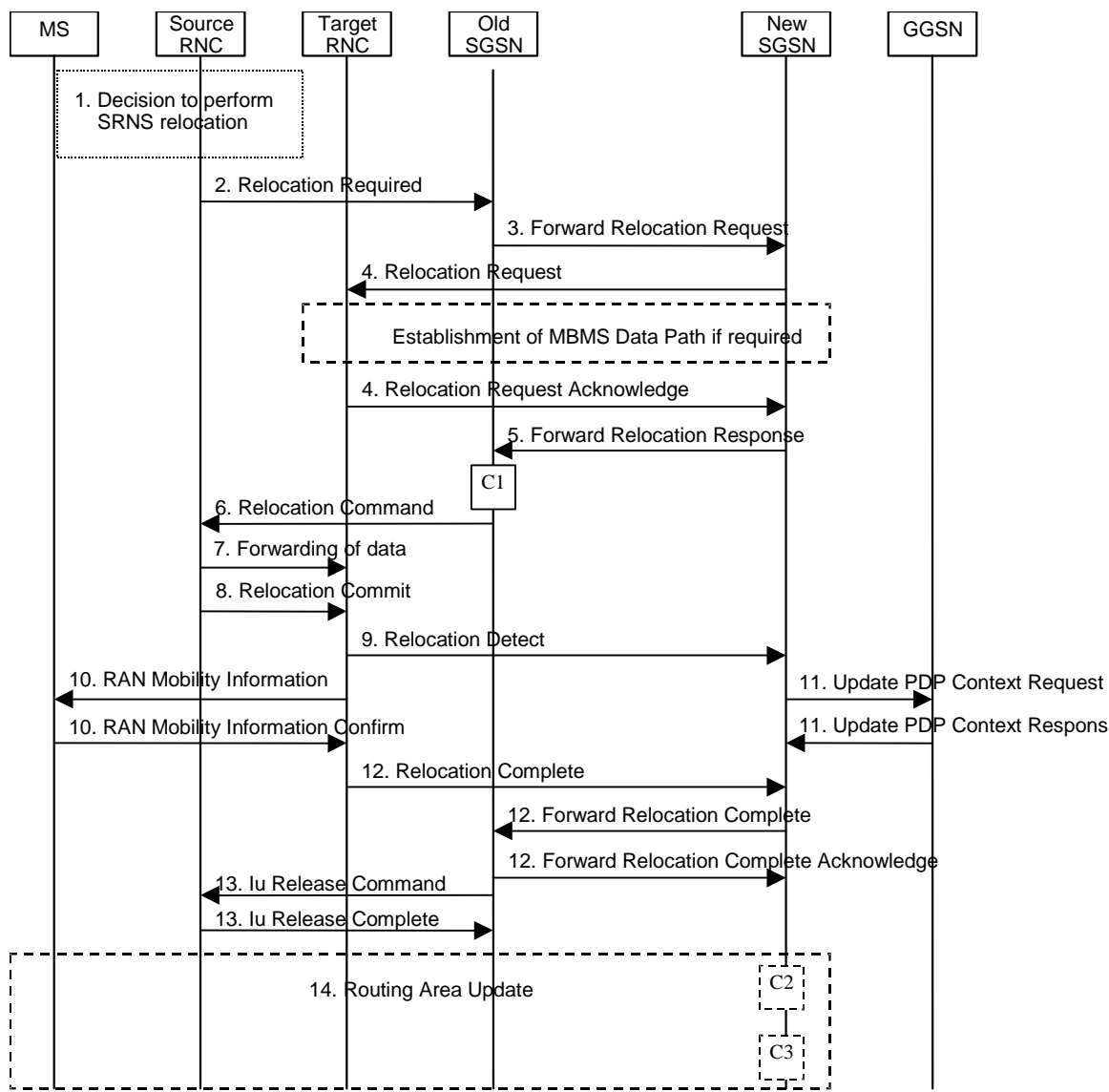
Figure 61: SRNS Relocation Procedure
