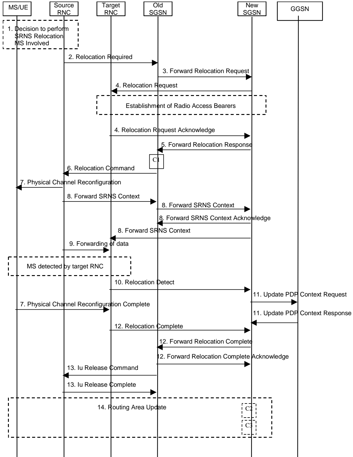
Figure 71: Combined Hard Handover and SRNS Relocation Procedure
