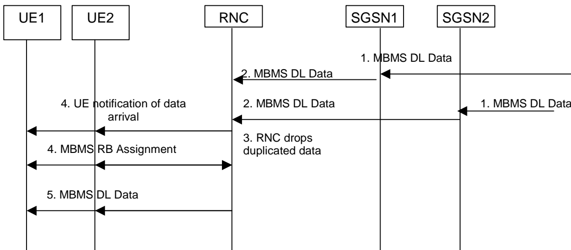
Figure 59: Downlink data transfer in case of Iu Flexibility
