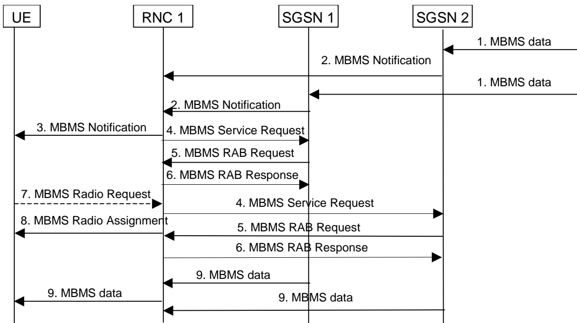
Figure 37: MBMS RAB set-up with IuFlex
