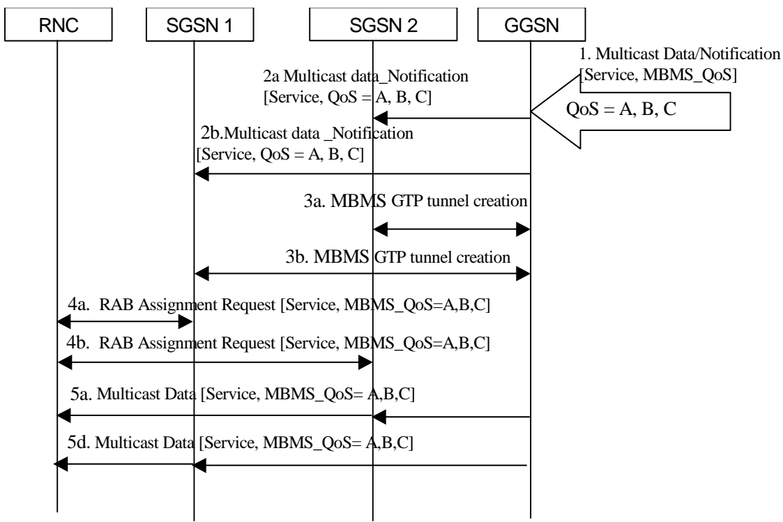
Figure 77: MBMS QoS Aspects of Multicast RAB set-up
