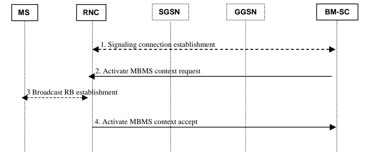
Figure 62: Broadcast service with interface between BM-SC and RNC
