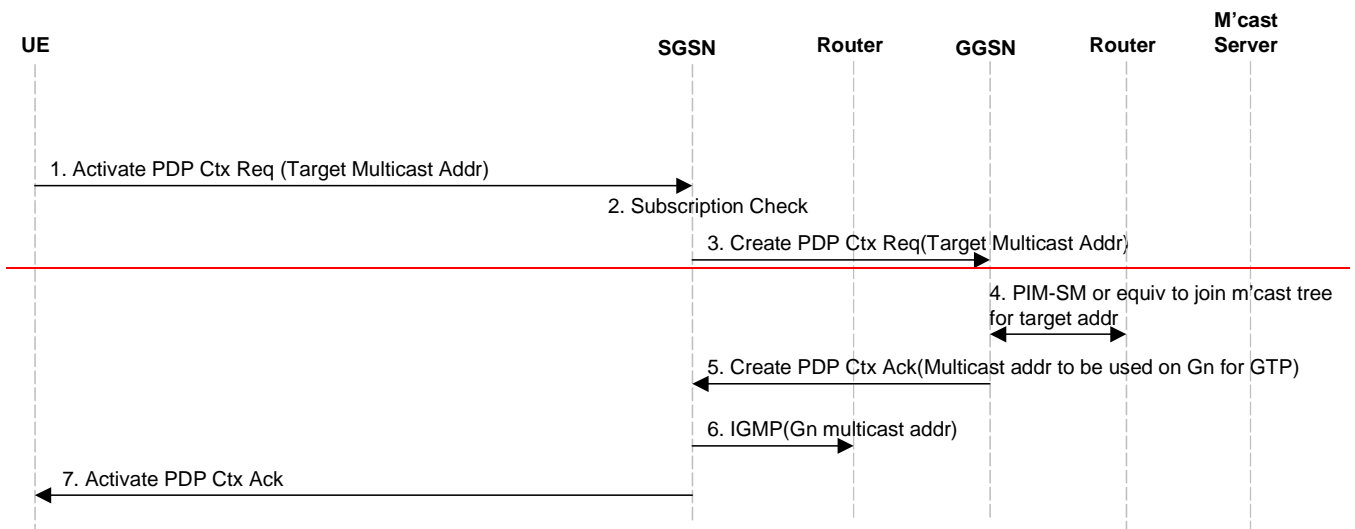
Figure 6— Example activation procedure
