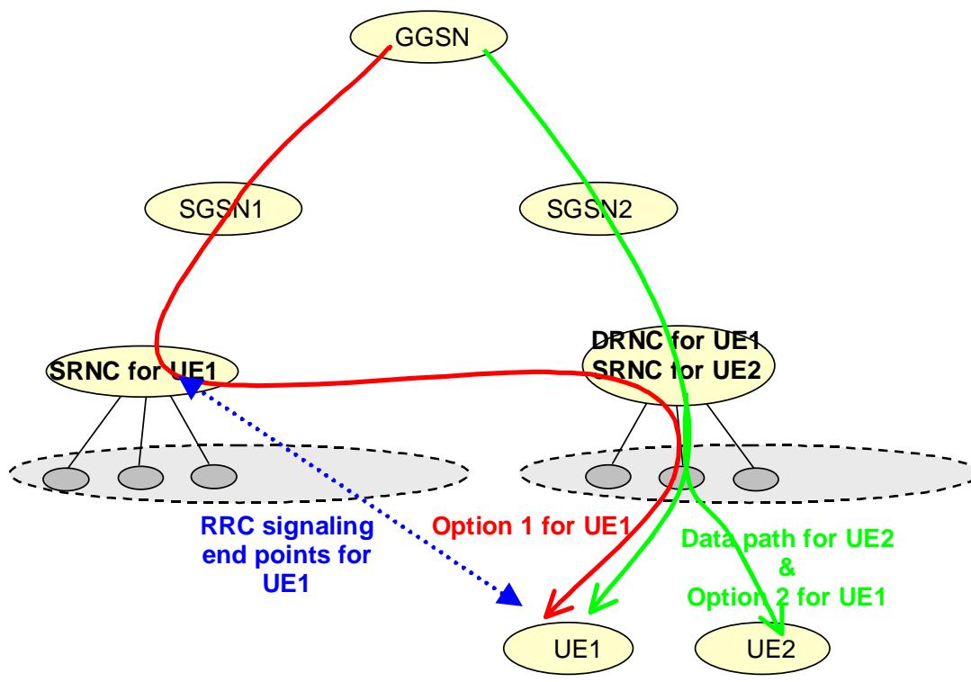
Figure 30: The two possible options for data path for UE1 which is served by DRNC. Option 1 is via the SRNC. Option 2 is via a DRNC; note that the DRNC for UE1 could be serving another UE2 as a SRNC and the same data feeds both UE1 and UE2.
