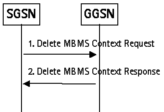
Figure 47: MBMS broadcast service deactivation
