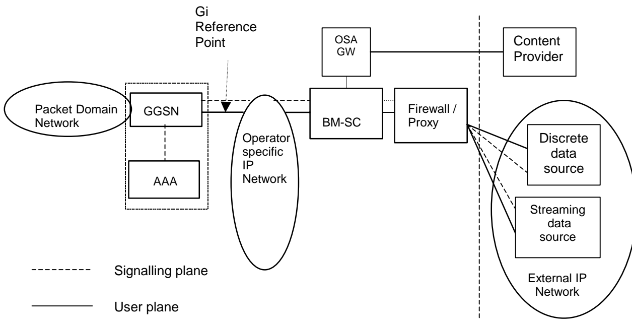
Figure 76: External interfaces
