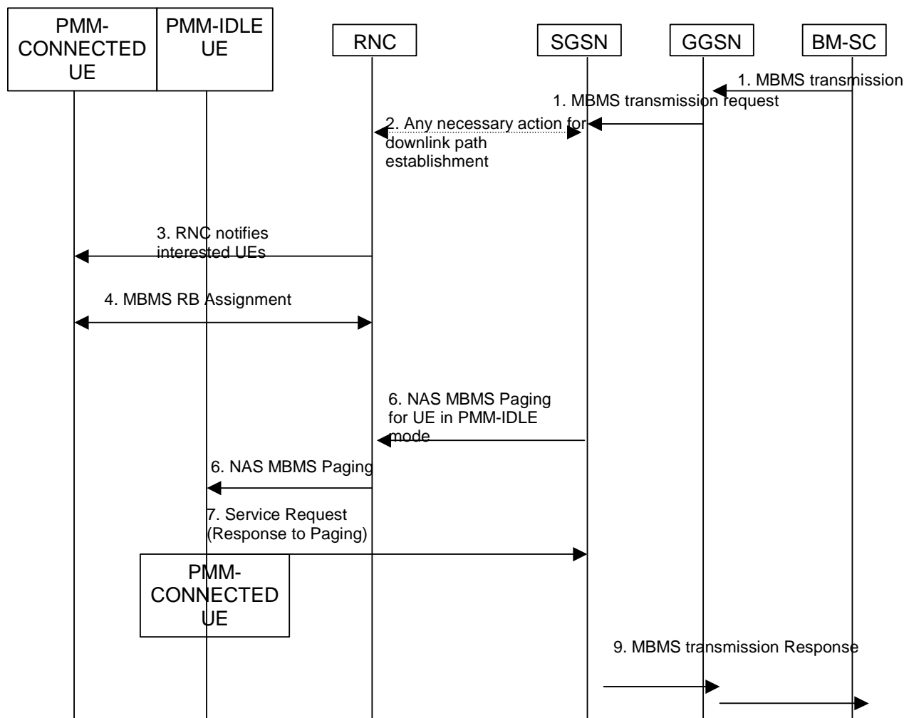
Figure 60: Optional MB-SC notification before MBMS data transfer
