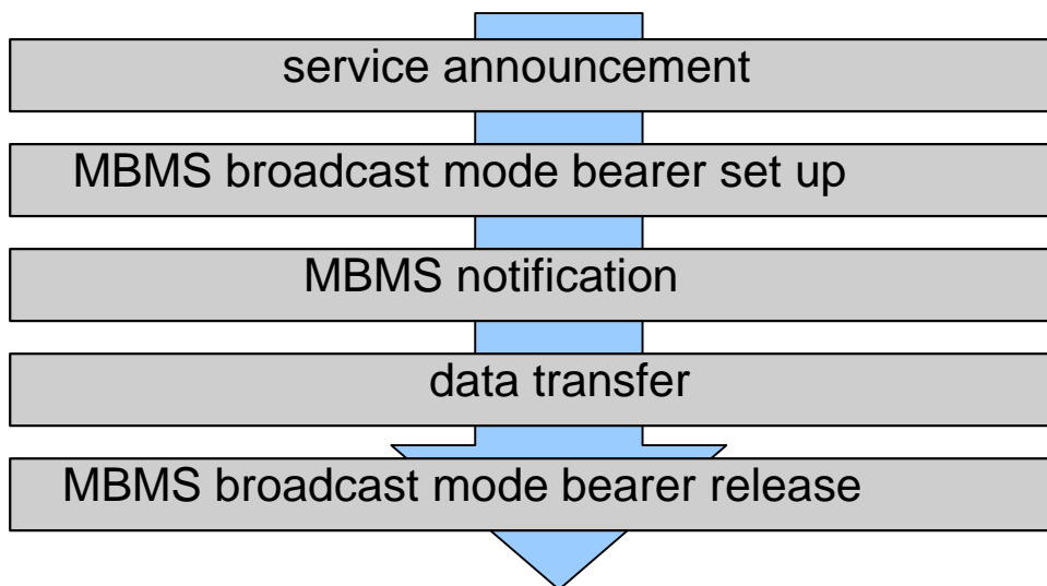
Fig. 25: Phases of MBMS broadcast service provision
