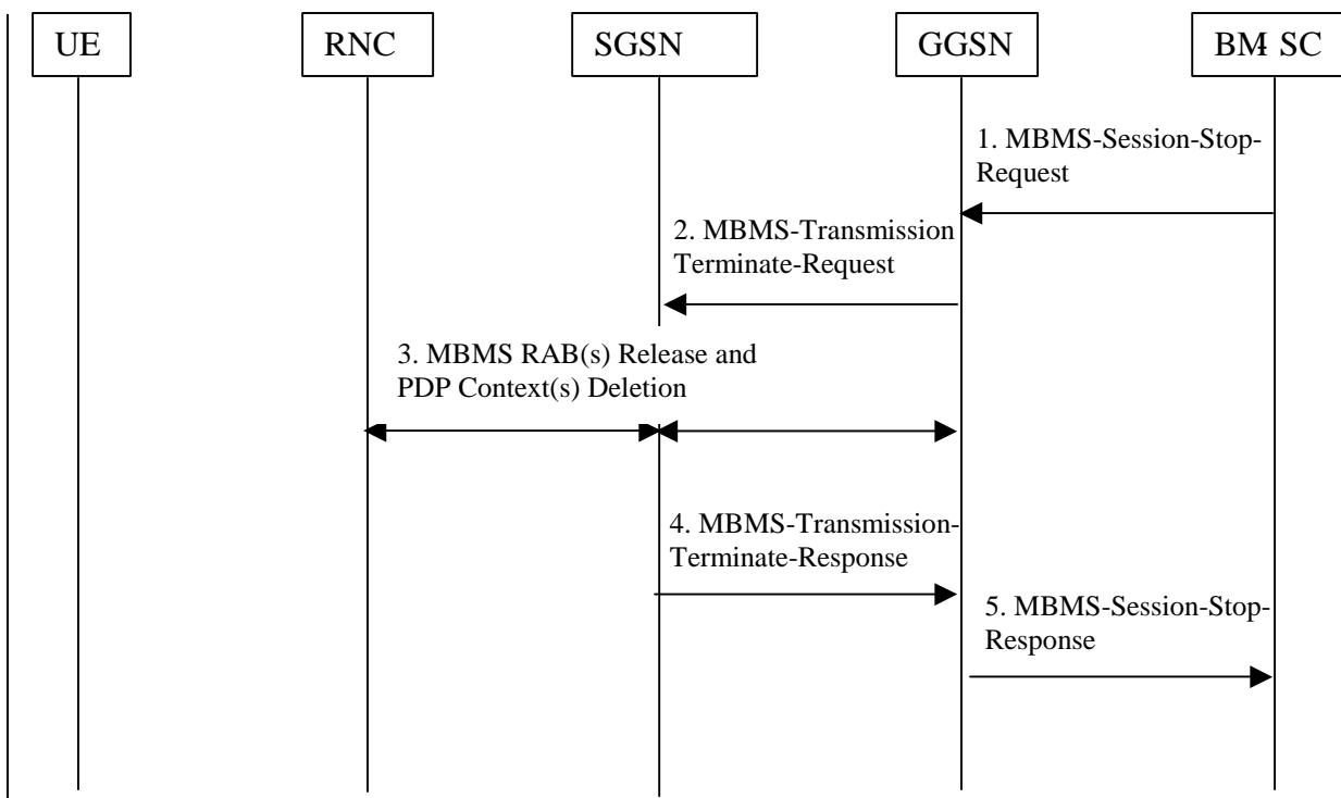
Figure 53. Terminating an MBMS Transmission
