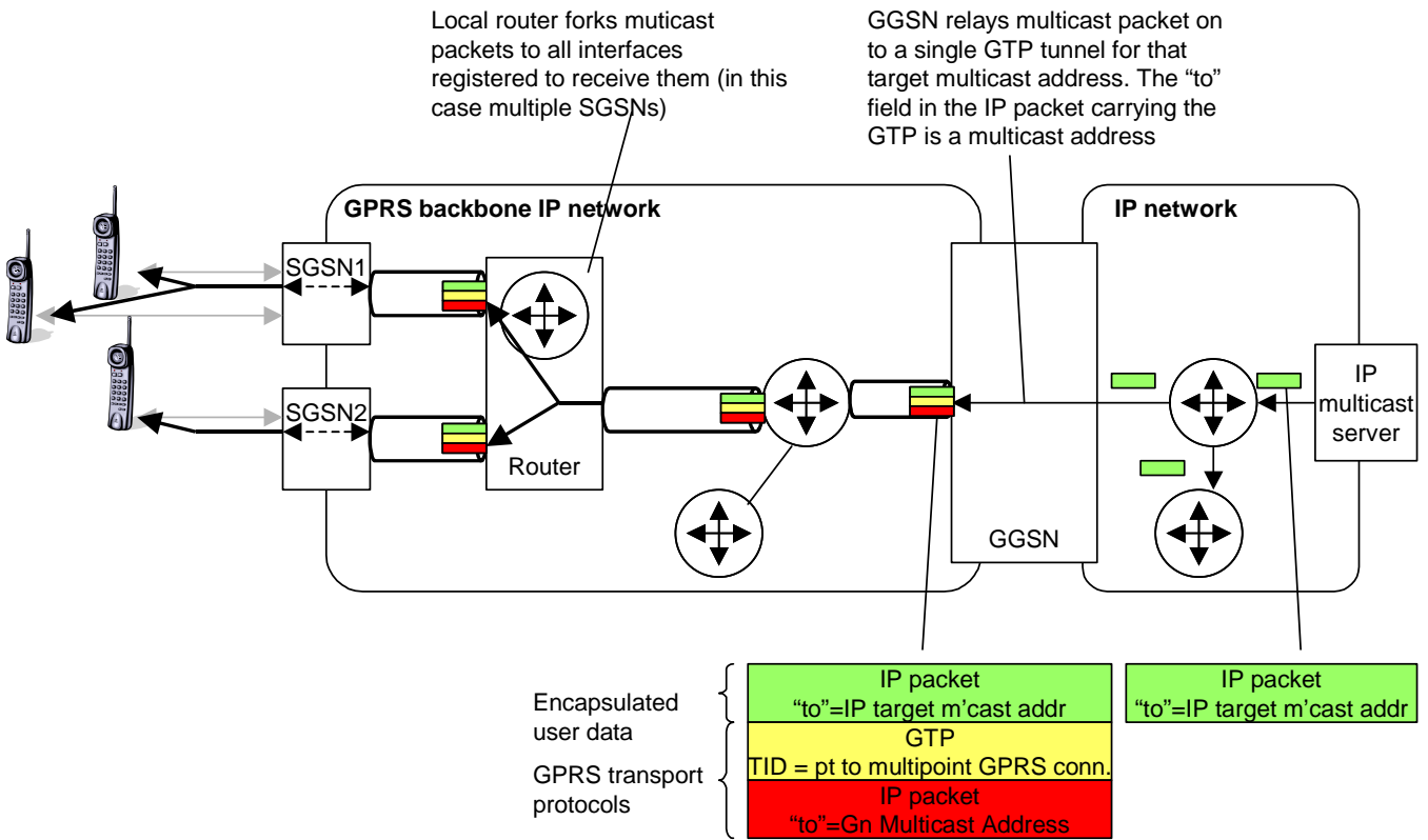
Figure 28: Optimised User Plane connections using IP multicast on the Gn interface
