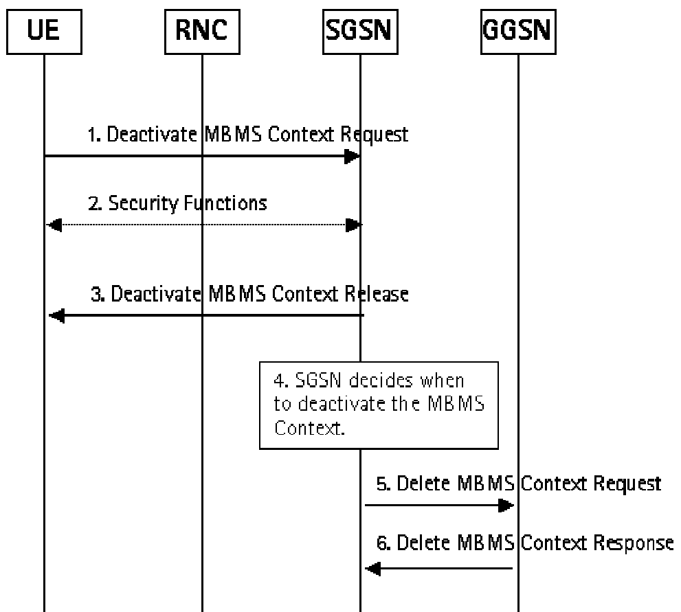
Figure 48: MBMS multicast service deactivation
