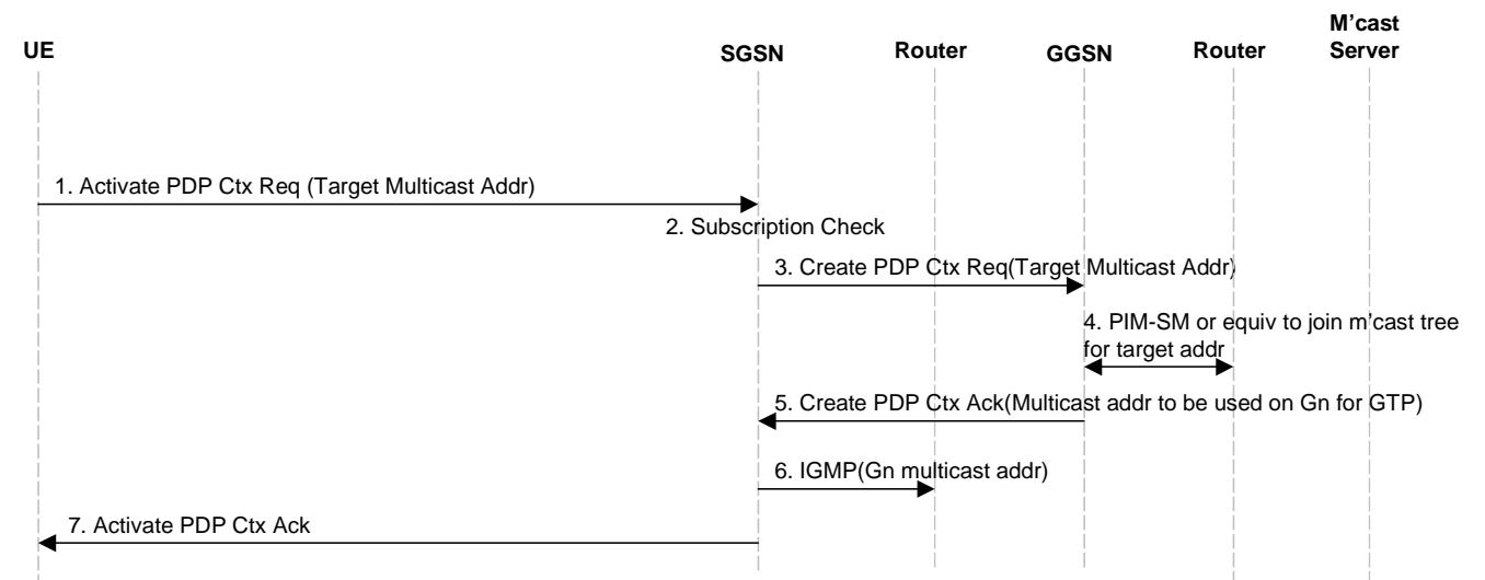
Figure 29 - Example activation procedure
