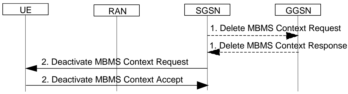
Figure 41: SGSN-initiated MBMS Context Deactivation Procedure
