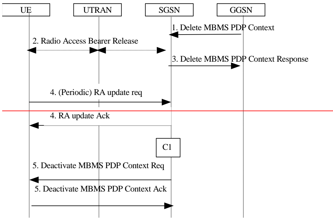
Figure 22. GGSN initiated MBMS PDP context deactivation procedure
