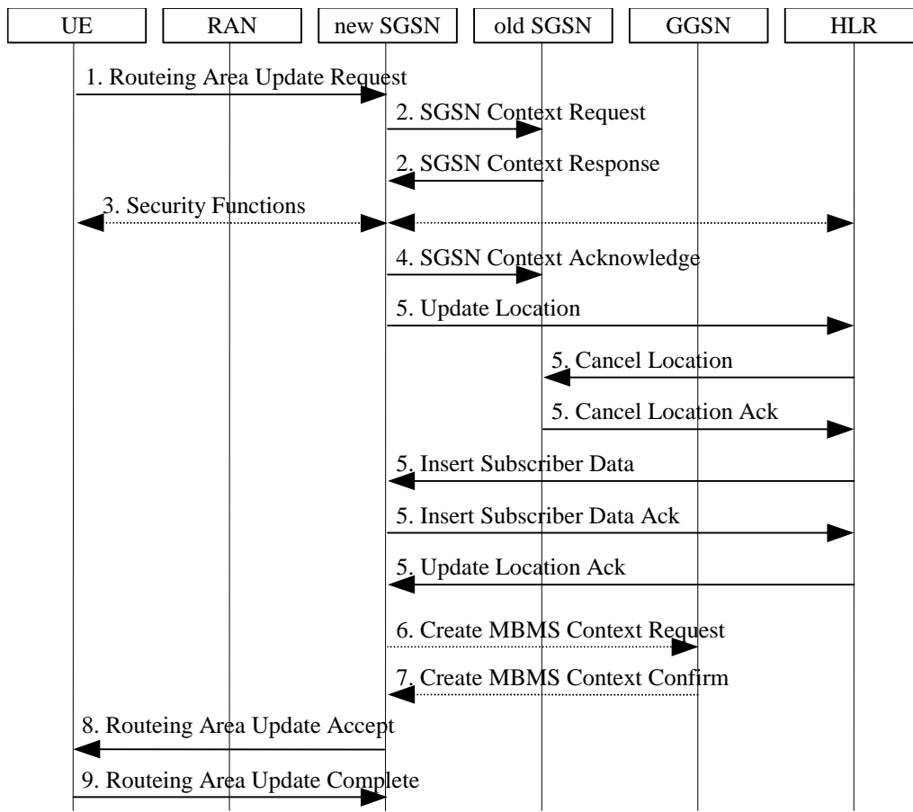
Figure 38. Mobility between SGSNs
