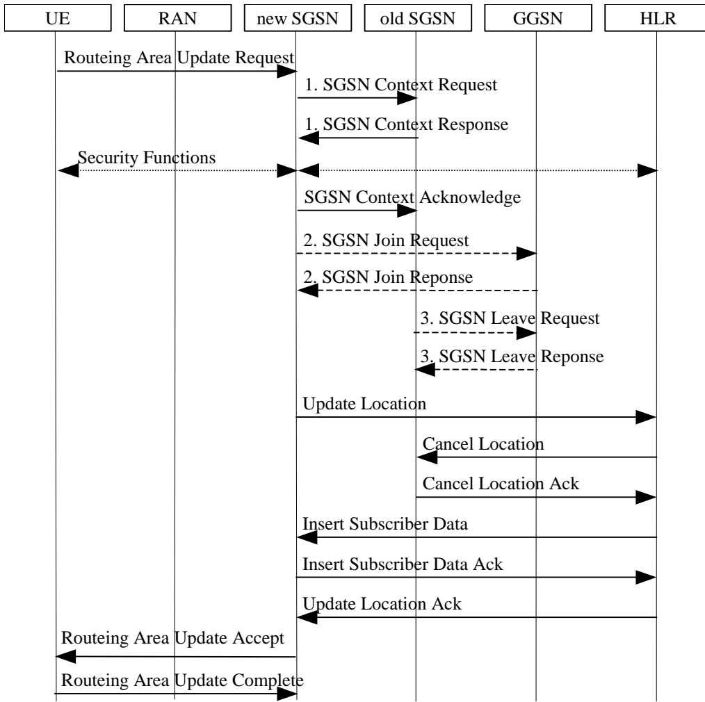
Figure 54: MBMS exchanges during RA update procedure
