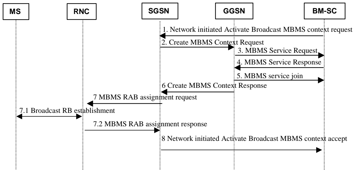
Figure 64: Broadcast service with MBMS Contexts activation
