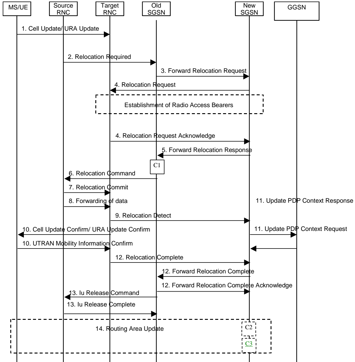
Figure 72: Combined Cell / URA Update and SRNS Relocation Procedure
