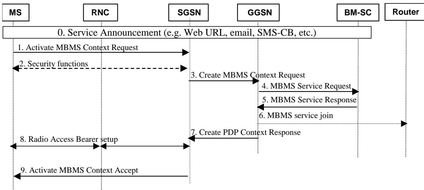
Figure 56: MBMS multicast mode service activation: MBMS context activation
