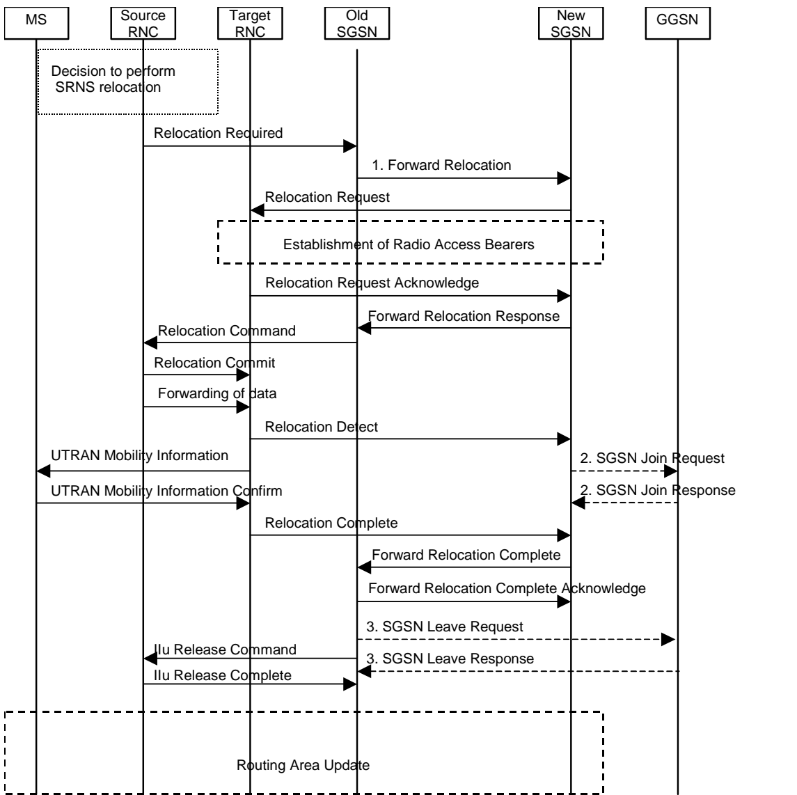
Figure 55: MBMS exchanges in SRNS relocation procedure
