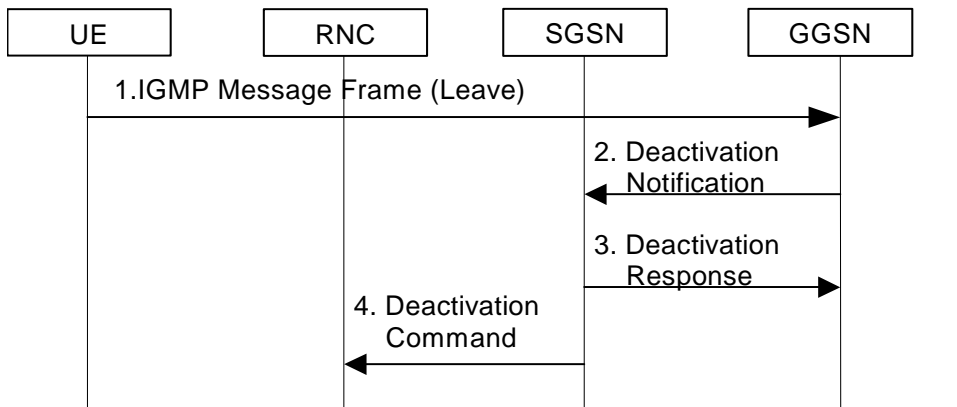
Figure 74: MBMS Multicast leave procedure
