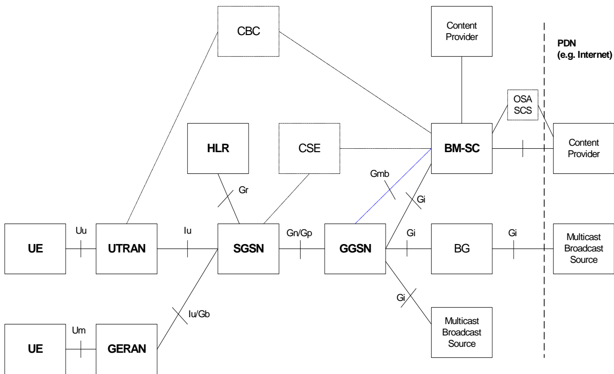
Figure 24. MBMS Architecture
