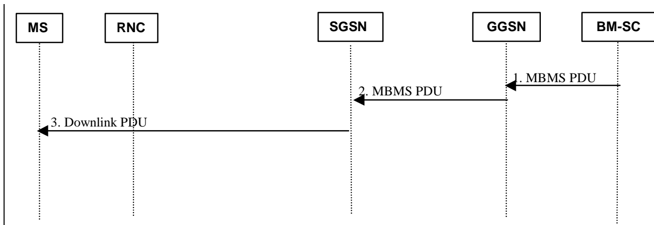
Figure 65: MBMS broadcast service notification and data transfer setup
