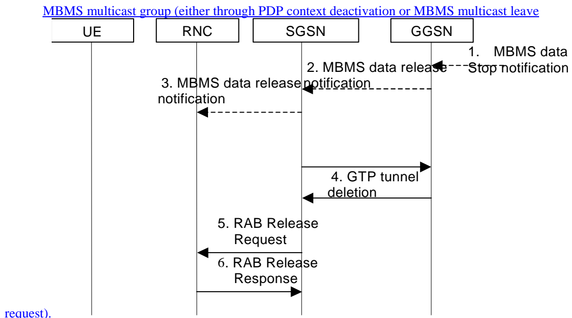
Figure 75: MBMS Bearer release procedure
