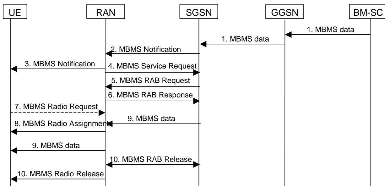
Figure 36. MBMS RAB set-up
