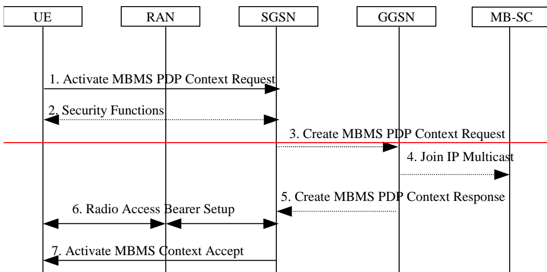
Figure 21. The activation of an MBMS multicast service
