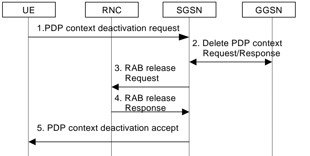
Figure 73: PDP context deactivation procedure
