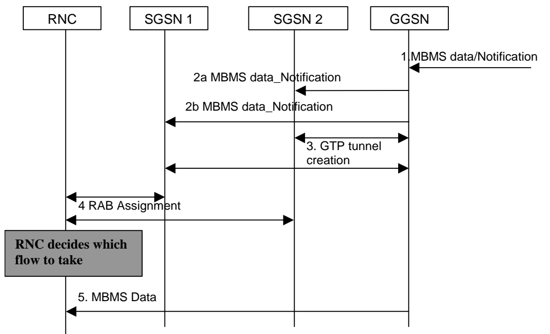
Figure 67: MBMS Bearer Path set-up with Iu-Flex configured
