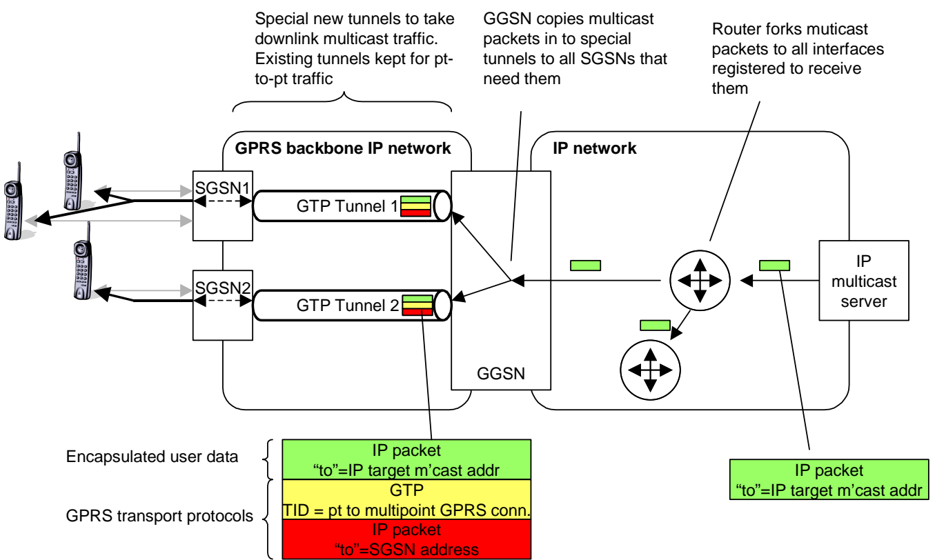
Figure 27: Optimised User Plane connections using IP unicast on the Gn interface
