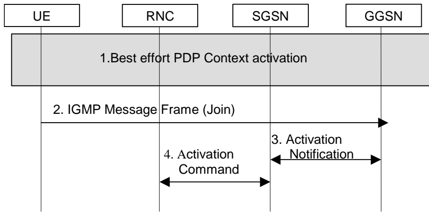
Figure 66: Activation of an MBMS multicast service
