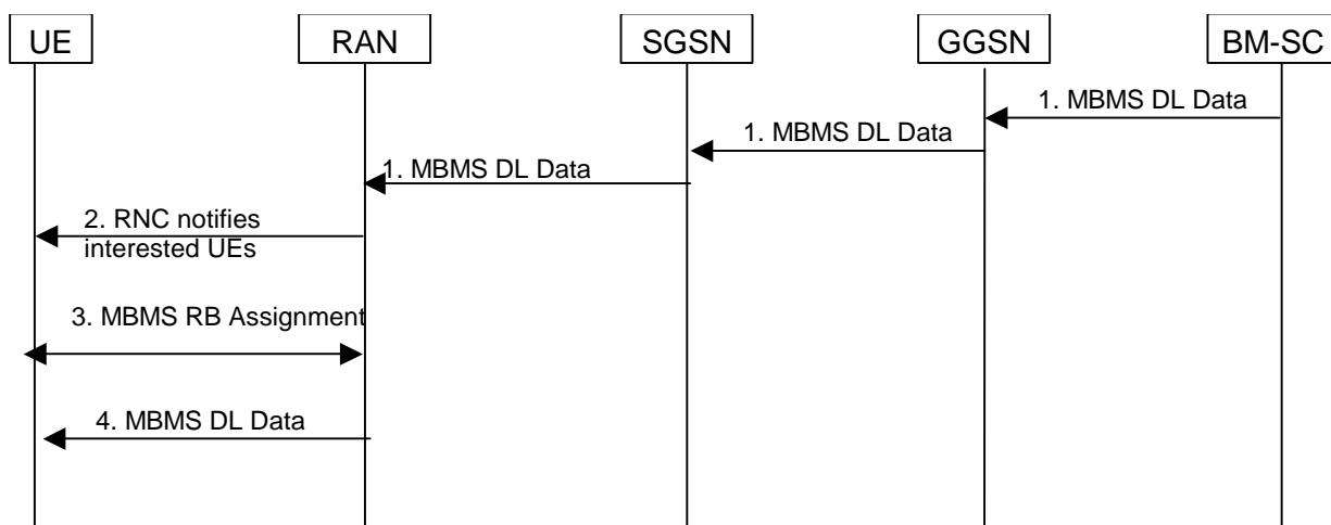
Figure 58: MBMS DL Data transfer when MBMS user plane is established
