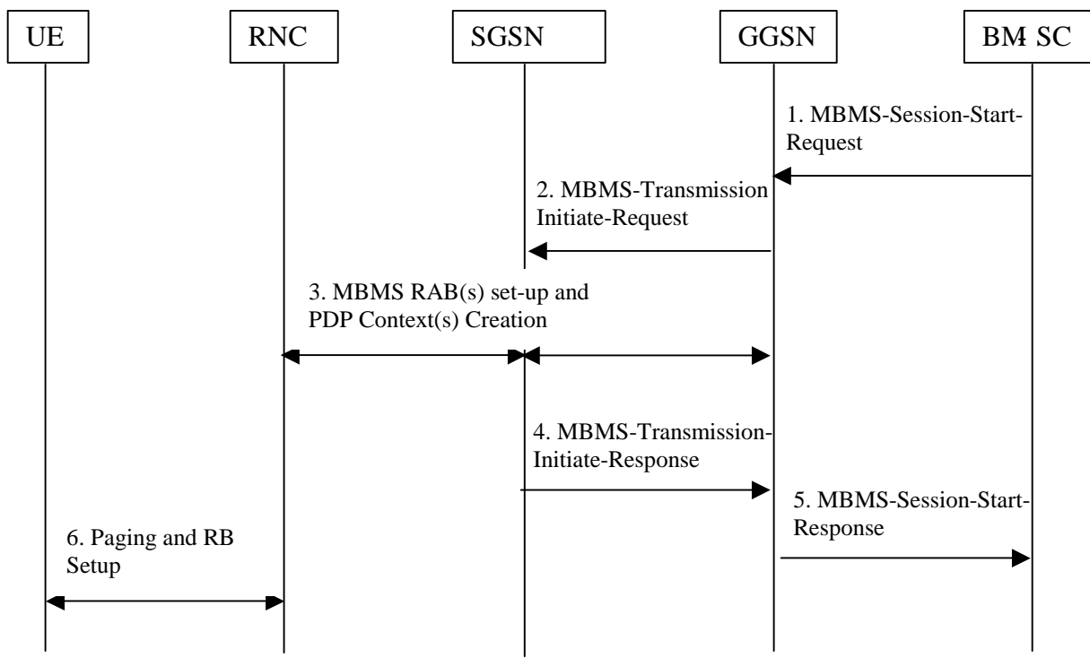
Figure 52. Initiating an MBMS Transmission
