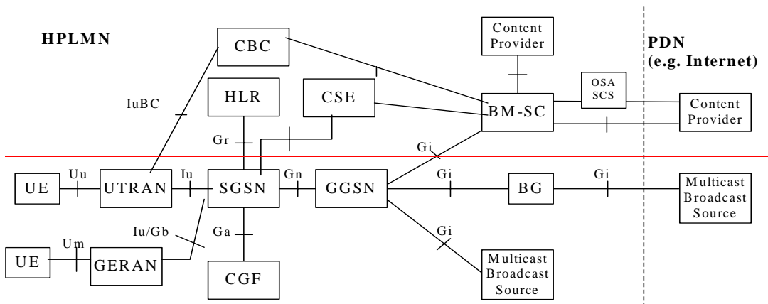
Figure 1. MBMS Architecture
