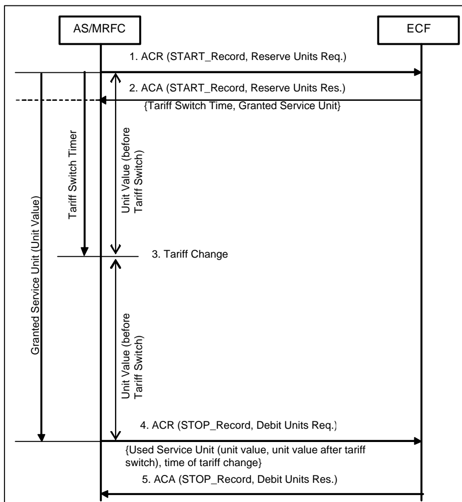
Figure 6.3: Tariff Change in the AS/MRFC
