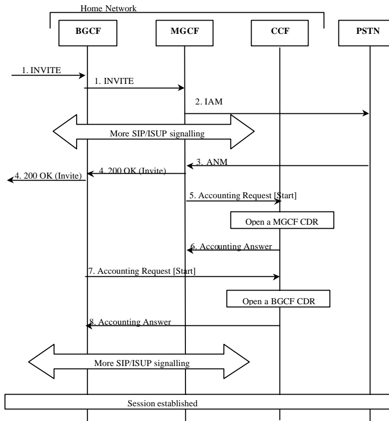
Figure 5.8: Message Sequence Chart for Session Establishment (IMS Initiated)
