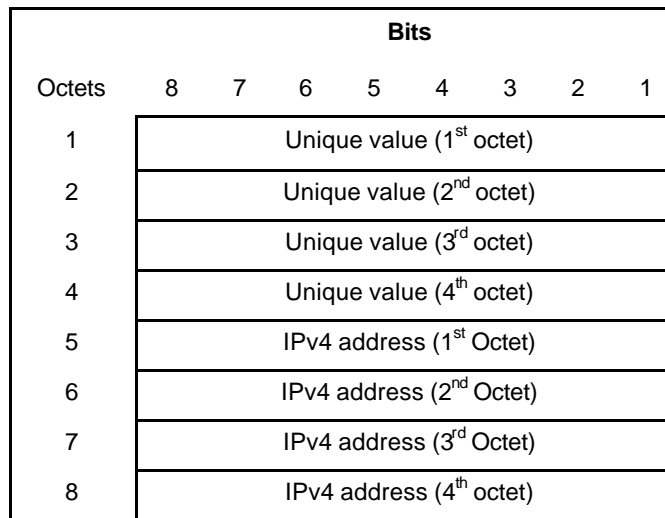
Figure 5.14: ICID layout with IPv4
