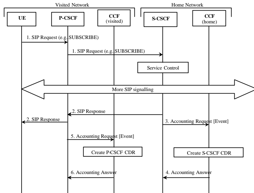
Figure 5.6: Message Sequence Chart for Session-Unrelated Procedure
