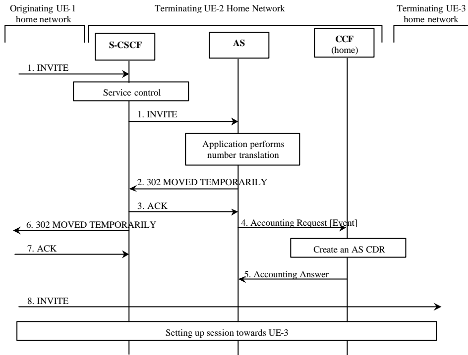
Figure 5.12: Message Sequence Chart for AS Acting as a Redirect Server
