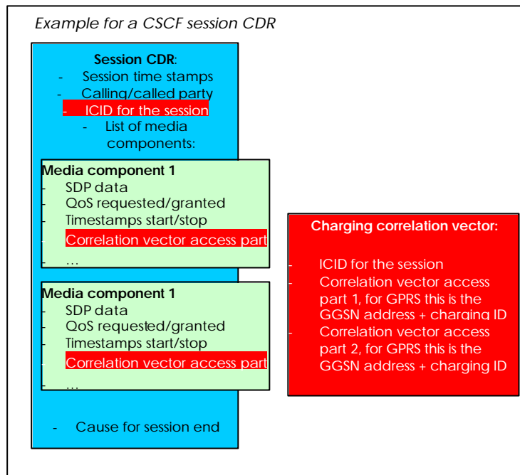
Figure 5.16: Charging Data Record Structure
