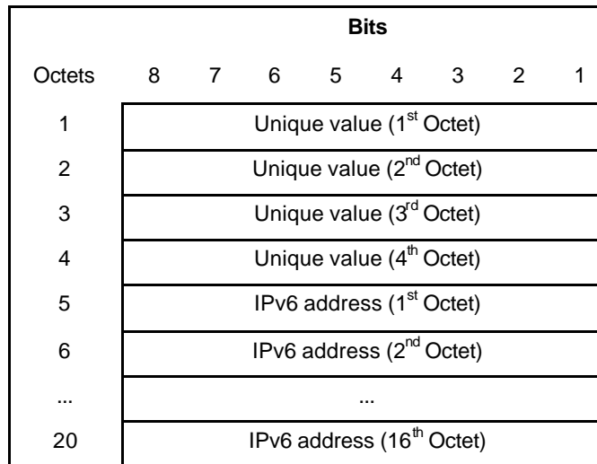
Figure 5.13: ICID layout with IPv6
