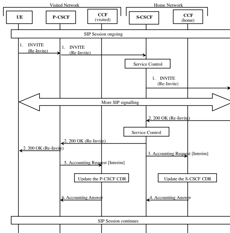
Figure 5.3: Message Sequence Chart for Media Modification
