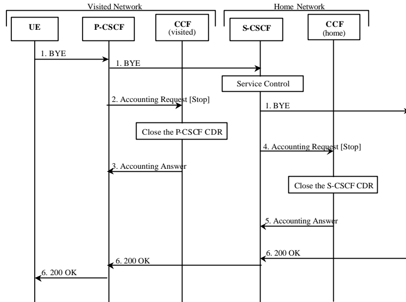
Figure 5.4: Message Sequence Chart for Session Release
