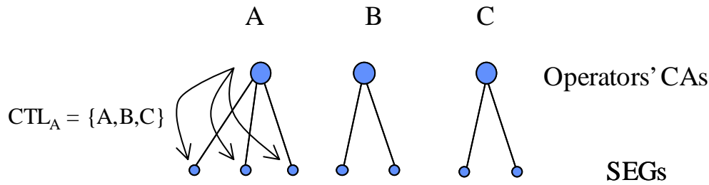
Figure 7: CTL model
