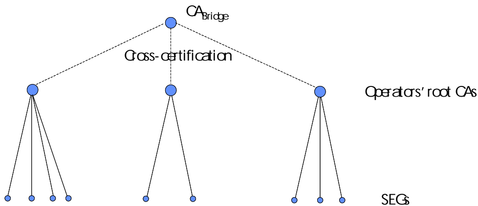
Figure 6: Bridge CA
