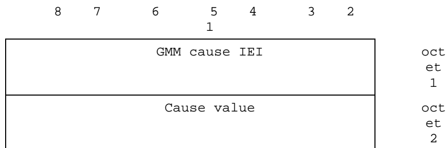
Figure 10.5.129/GSM 04.08: GMM cause information element
