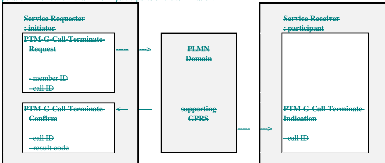
Figure 4: PTM-G call terminate operation
