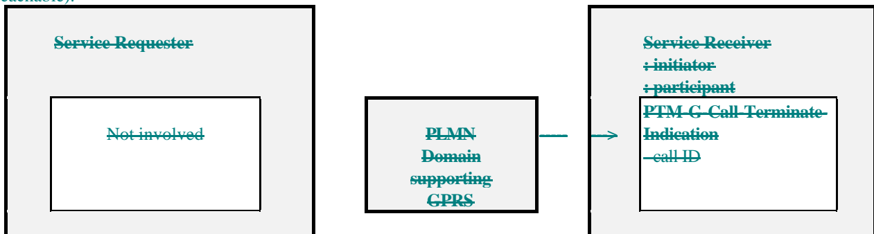
Figure 5: PTM-G network invoked call terminate operation
