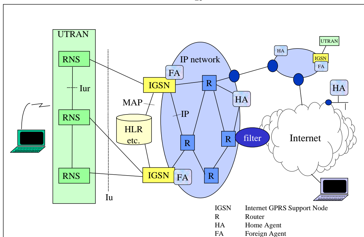
Figure 7.3.a. Core network architecture with Mobile IP+ MM within the CN and between different types of systems and between GPRS PLMN's.
