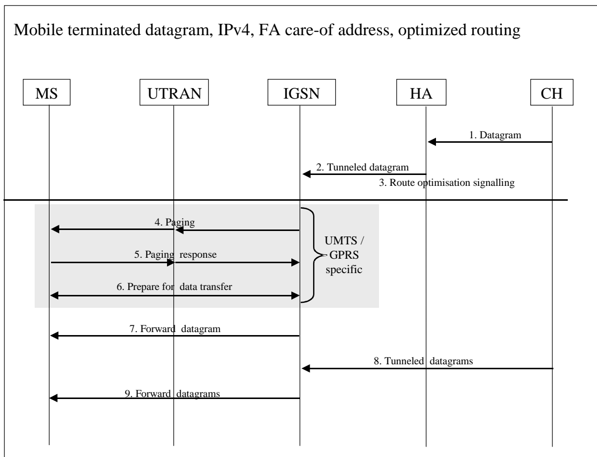
Figure 11.7.2.b: Delivery of mobile terminated datagrams, optimized routing.
