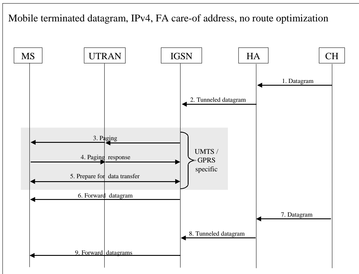
Figure 11.7.2.a: Delivery of mobile terminated datagrams, no route optimization
