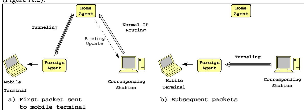
Figure A.2. Route Optimization in IPv4
