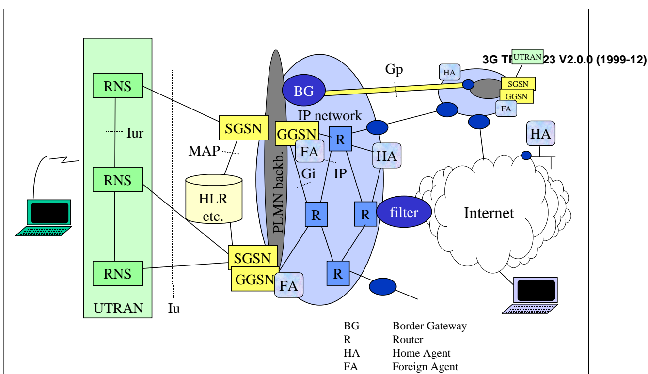
Figure 7.2.a. Core network architecture where GPRS MM handles active mobiles and Mobile IP(+) streamlining at inter SGSN handover. The SGSN and GGSN are here co-located.
