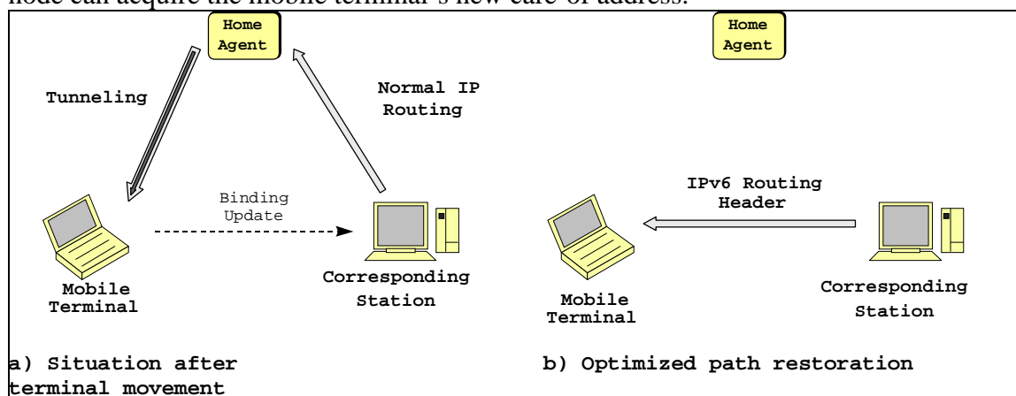
Figure A.5. Route Optimization in IPv6
