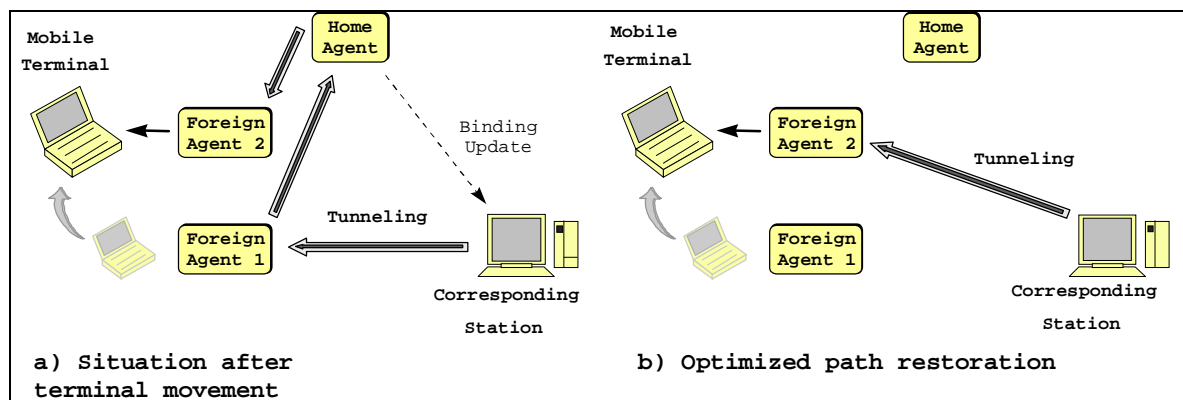
Figure A.4. Mobile terminal movement without notification to the previous foreign agent The Route Optimization mechanism specified for IPv4 has the advantage of minimizing signaling traffic carried by the portion of the network between the mobile terminal and the foreign agent, as all of the Binding Update messages addressed to the correspondent node are transmitted by the home agent rather than directly by the mobile terminal. This is an extremely important feature, given that the Binding Update messages are coded in UDP packets which are separate from data traffic and thus introduce an overhead that can become unacceptable on a wireless connection such as that between the mobile terminal and the foreign agent.
