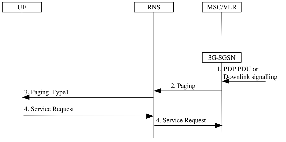
Figure 40: PS paging without RRC connection for CS
