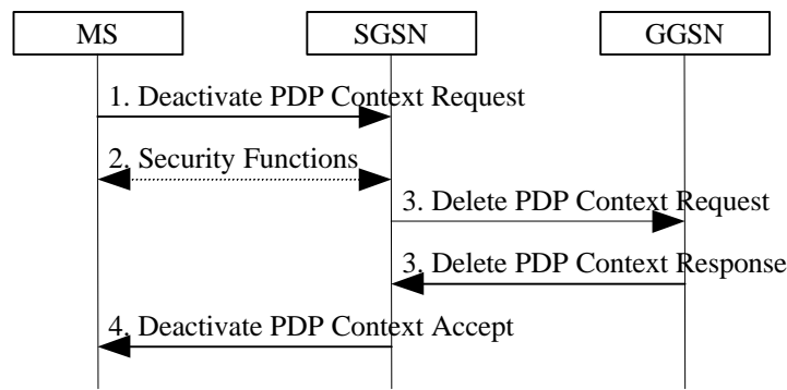
Figure 16: PDP Context Deactivation Initiated by MS Procedure for GPRS
