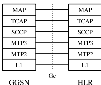
Figure 4214: Control Plane GGSN - HLR Using MAP
