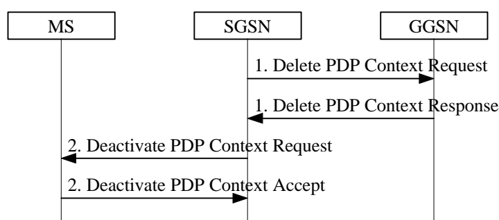
Figure 4: PDP Context Deactivation Initiated by SGSN Procedure
