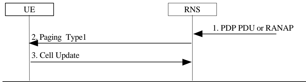
Figure 42: URA Paging Procedure
