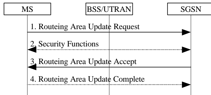
Figure 2: Intra SGSN Routing Area Update Procedure
