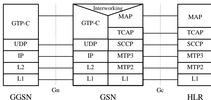
Figure 4315: Control Plane GGSN - HLR Using GTP and MAP
