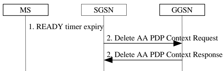
Figure 22: Anonymous Access PDP Context Deactivation Initiated by MS Procedure
