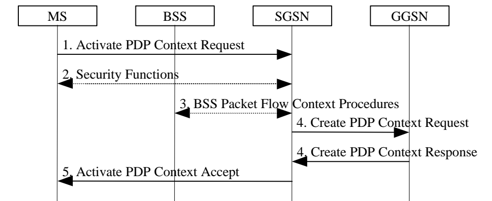
Figure 2: PDP Context Activation Procedure for GPRS
