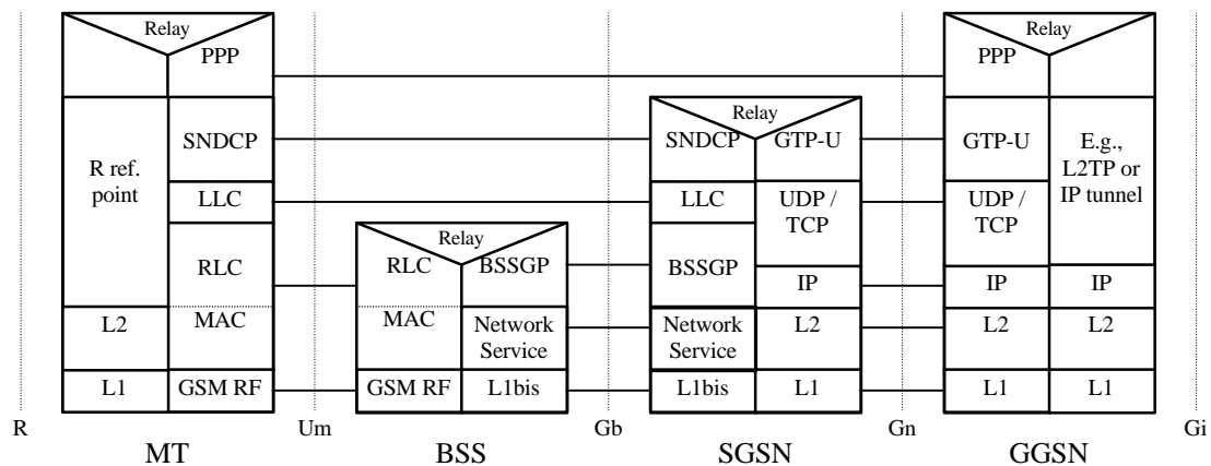
Figure 4: GPRS User Transmission Plane for PDP Type PPP
