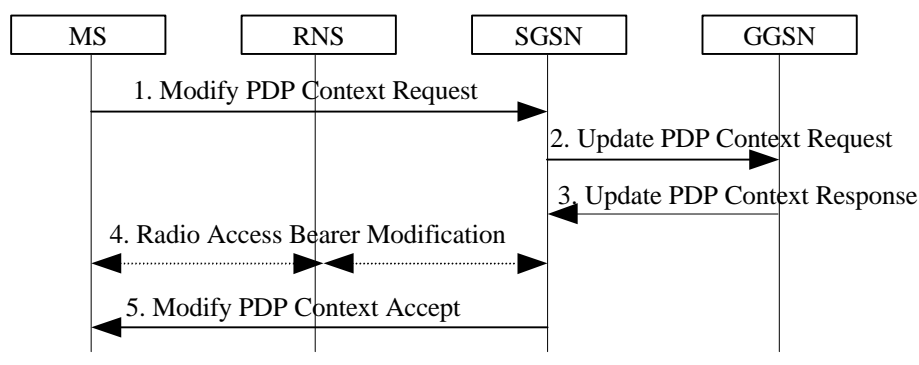
Figure 15: MS-Initiated PDP Context Modification Procedure for UMTS
