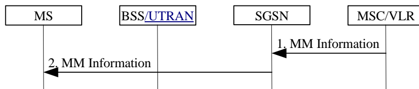
Figure 3: MM Information Procedure
