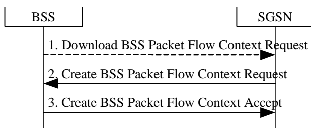
Figure 7: BSS Packet Flow Context Creation Procedure
