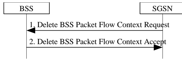
Figure 10: SGSN-Initiated BSS Packet Flow Context Deletion Procedure
