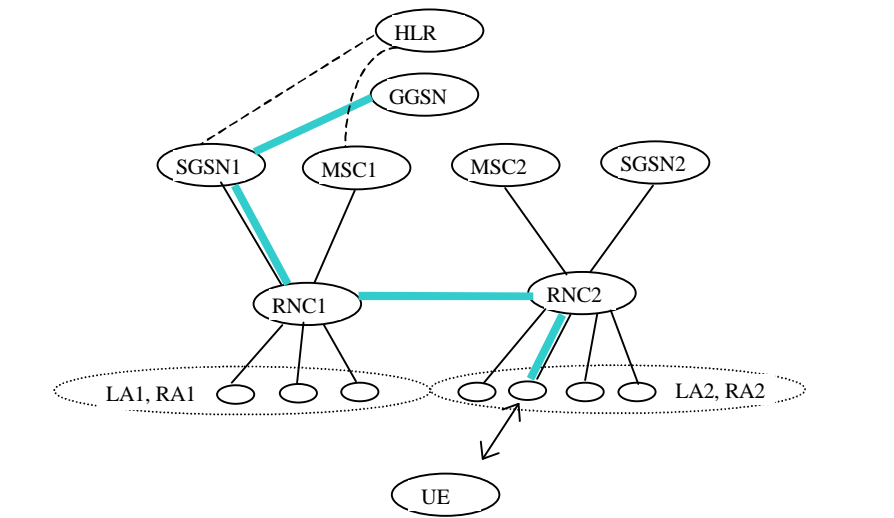
Figure 33 Before the SRNS relocation and location registration
