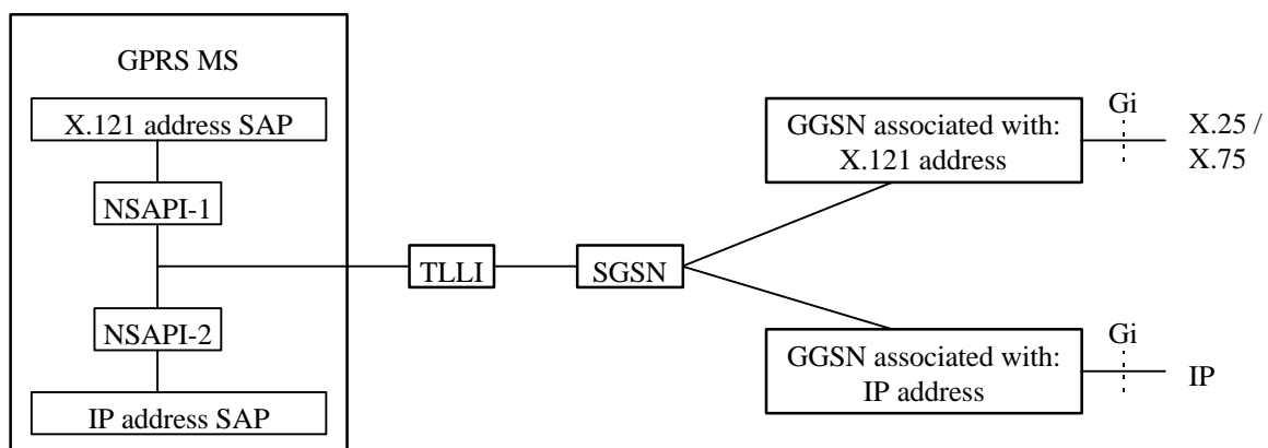
Figure 1: Use of NSAPI and TLLI
