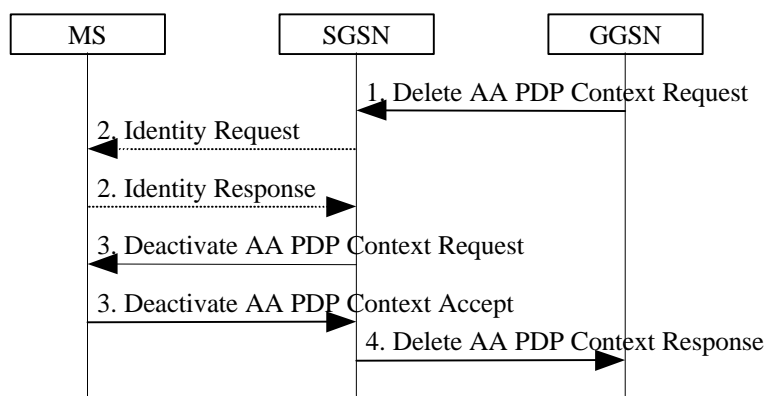
Figure 23: Anonymous Access PDP Context Deactivation Initiated by GGSN Procedure
