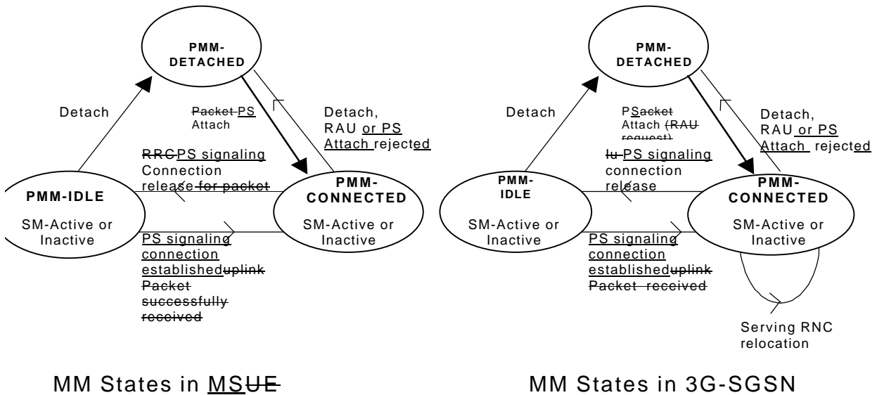
Figure 3: PMM State Model
