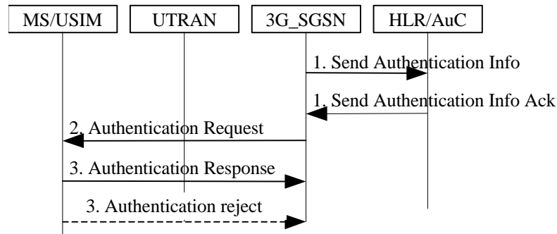
Figure 1-1: UMTS Authentication Procedure of UMTS subscriber
