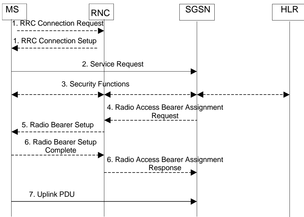
Figure 4: Uplink Transmission Procedure Service Request procedure initiated by MS
