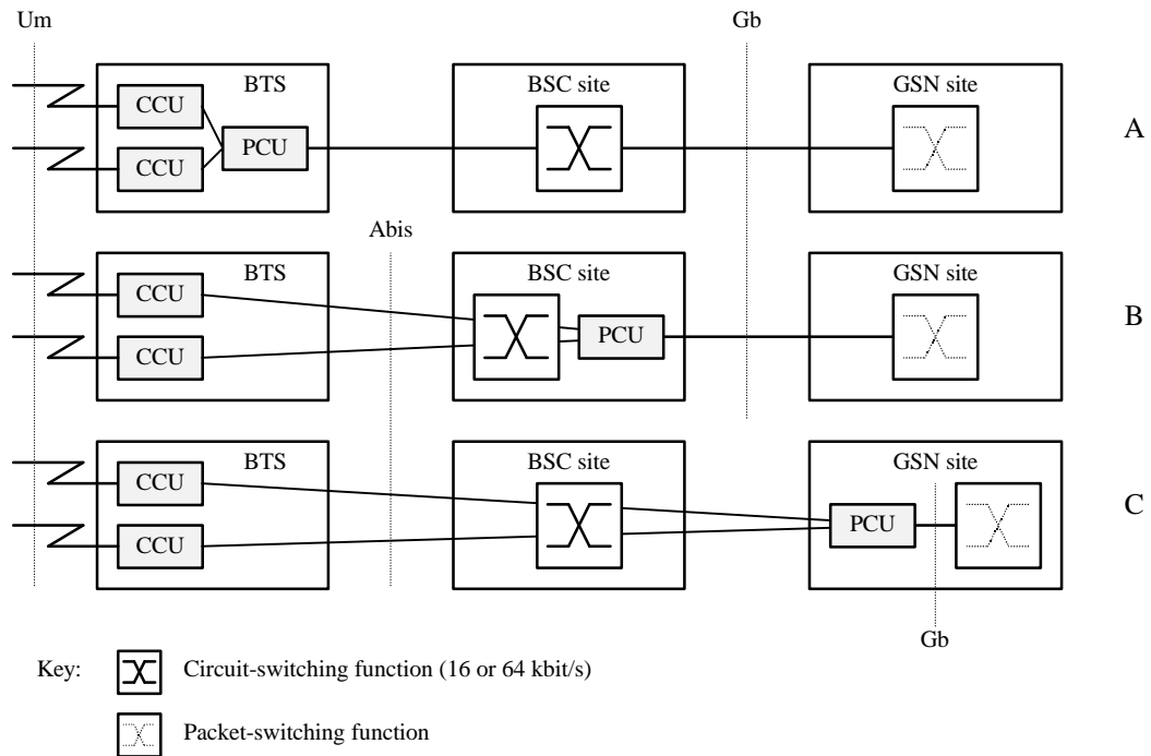
Figure 14: Remote Packet Control Unit (PCU) Positions
