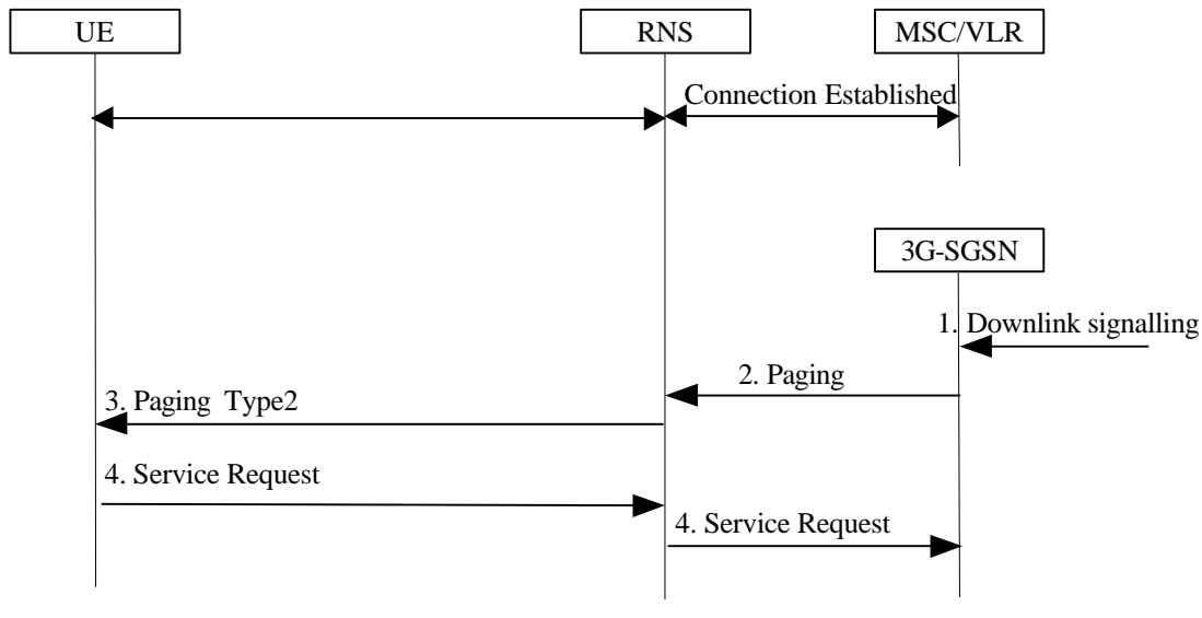
Figure 41: PS paging with RRC connection for CS
