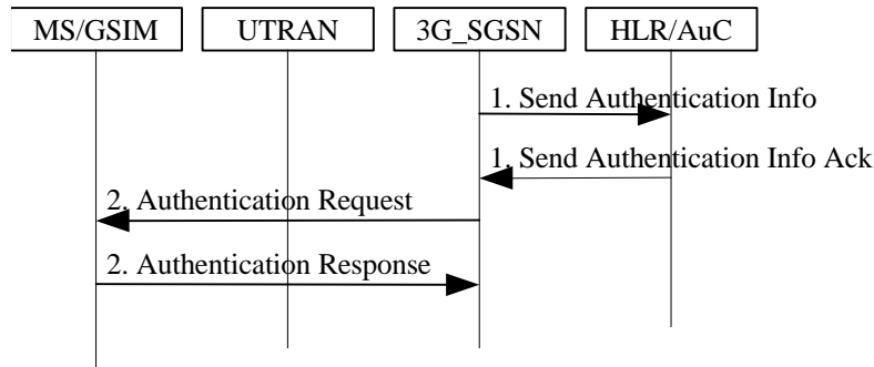
Figure 1-2: UMTS Authentication Procedure of GSM subscriber
