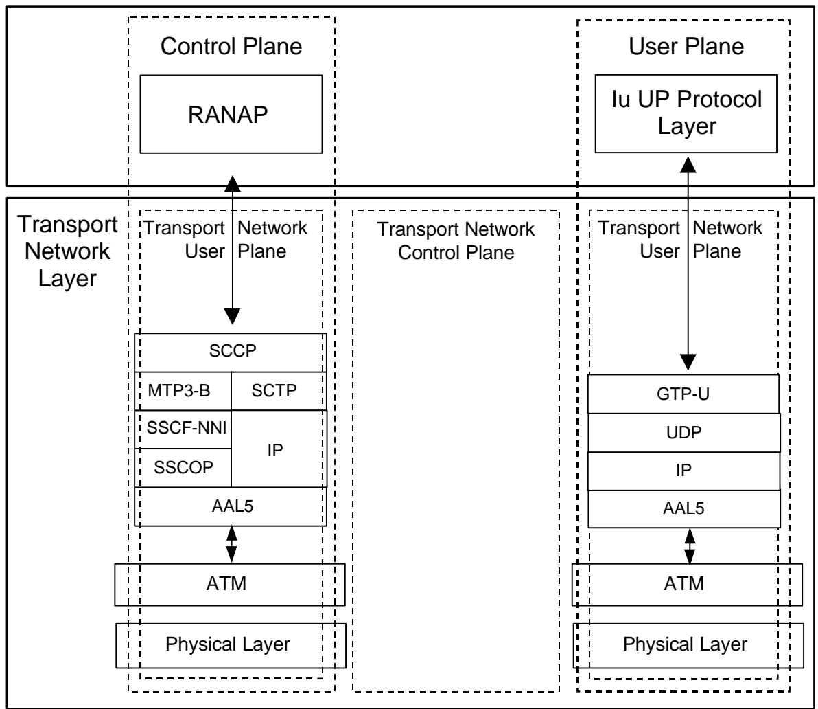
Figure 11: protocol configuration on the Iu user plane for packet switched traffic
