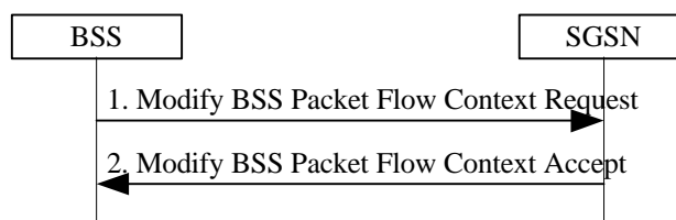
Figure 9: BSS-Initiated BSS Packet Flow Context Modification Procedure
