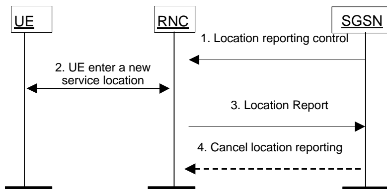
Figure 13: Location Reporting Procedure
