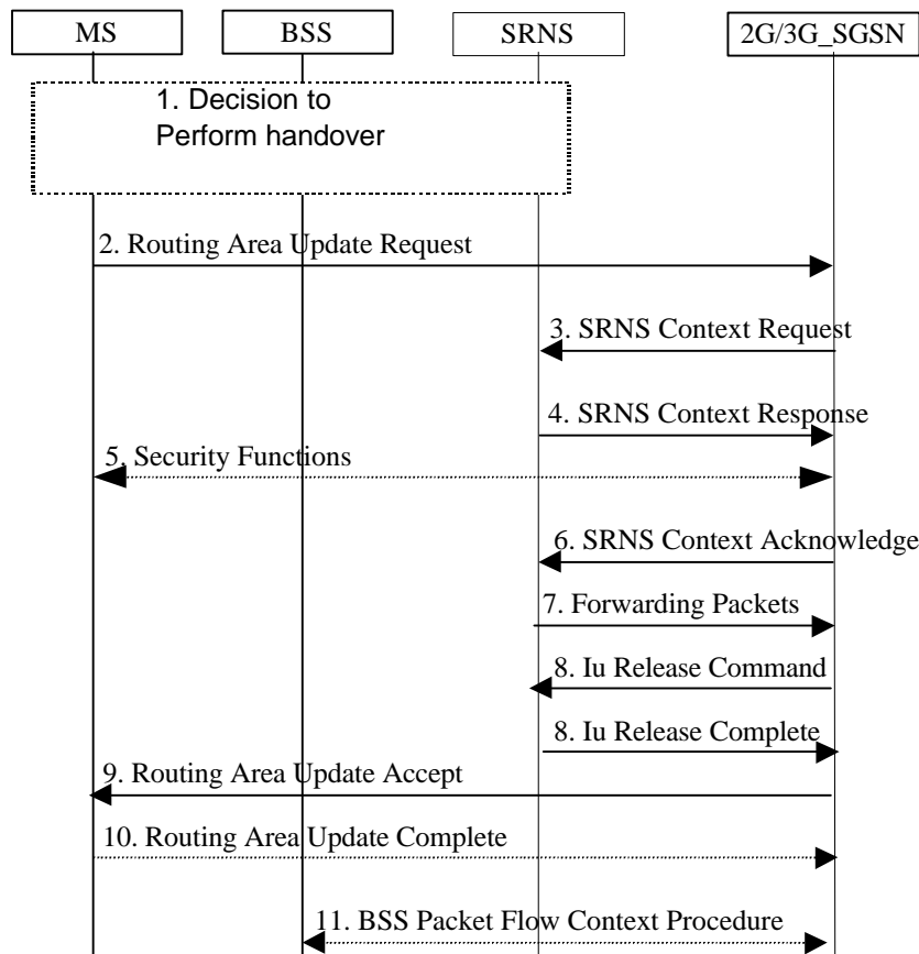
Figure ZZD: UMTS to GSM GPRS handover between cells belonging to the same RA
