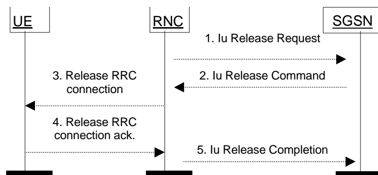
Figure 12: Iu Release Procedure
