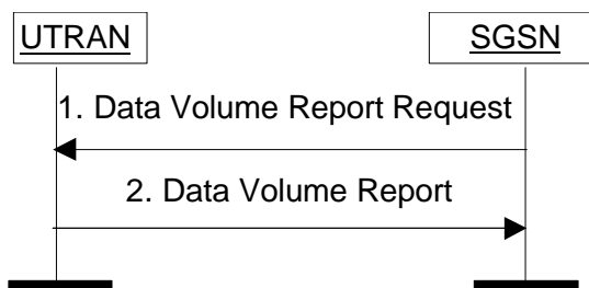
Figure 70: Data Volume Report procedure initiated by SGSN
