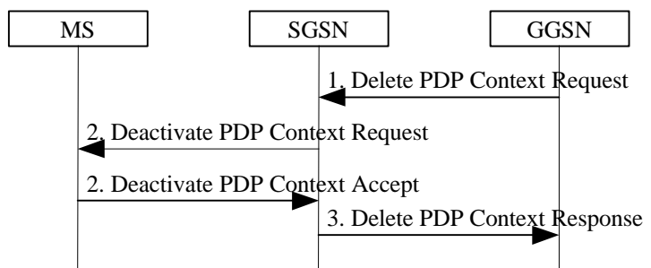
Figure 20: PDP Context Deactivation Initiated by GGSN Procedure for GPRS
