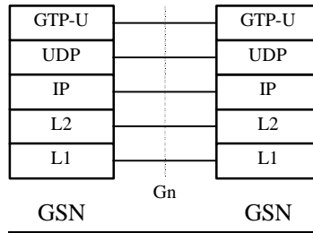
Figure 5: User Plane GSN - GSN
