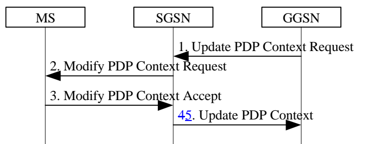
Figure 12: GGSN-Initiated PDP Context Modification Procedure for GPRS
