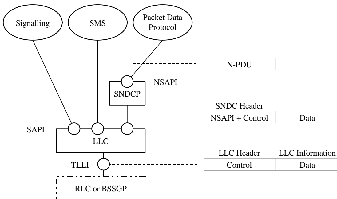
Figure 1: Multiplexing of Network Protocols
