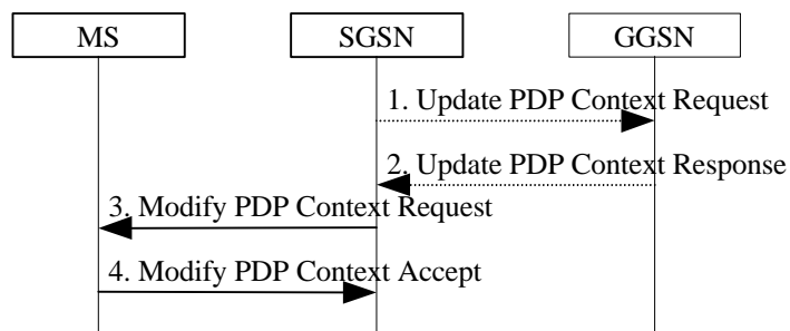
Figure 10: SGSN-Initiated PDP Context Modification Procedure for GPRS
