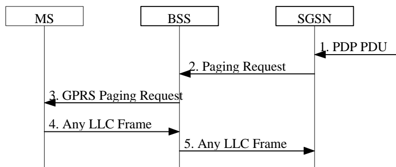
Figure 1: GPRS Paging Procedure
