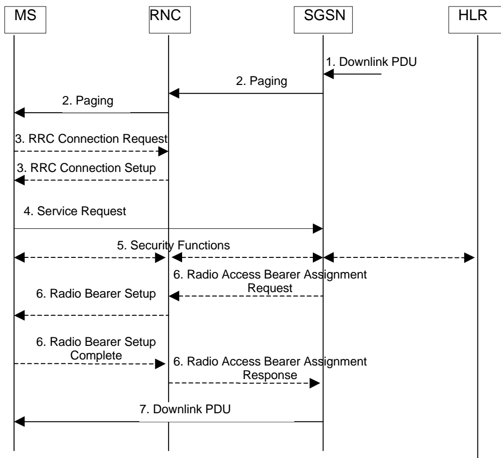
Figure 5: Service Request procedure initiated by network Downlink Transmission Procedure
