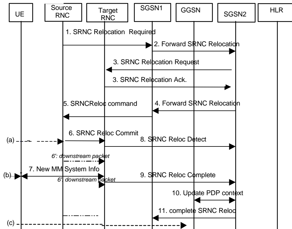
Figure 34 Phases 1 & 2 of the Serving RNC Relocation.
