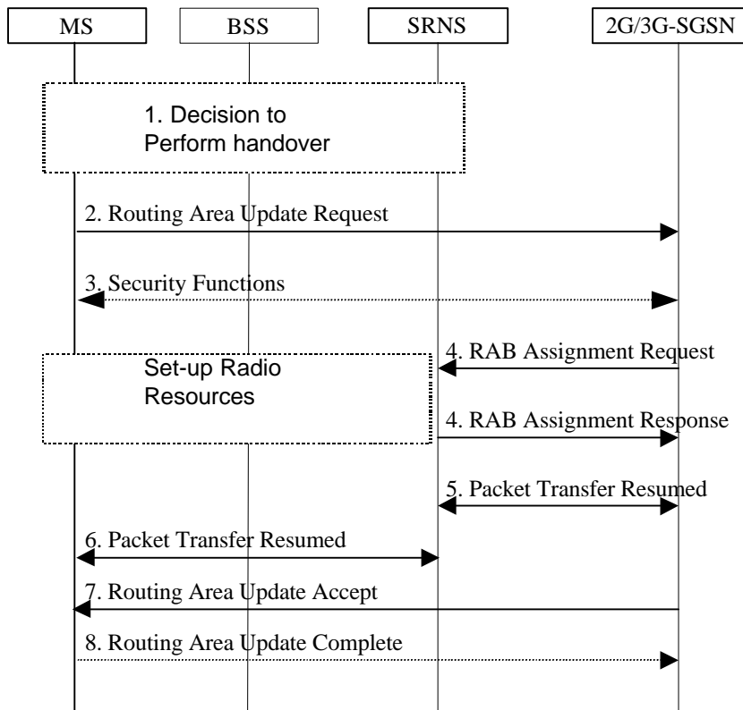
Figure ZZD: GSM GPRS to UMTS handover between cells belonging to the same RA
