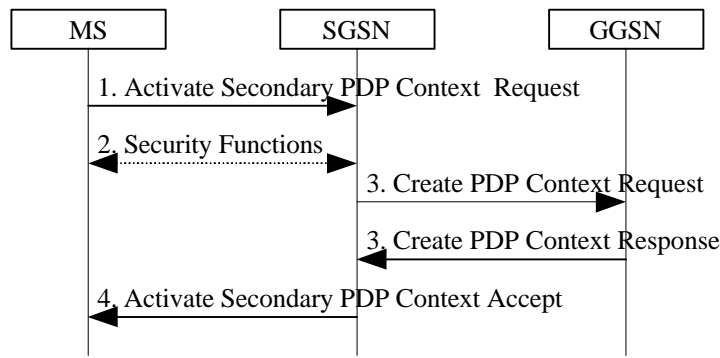
Figure 4: Secondary PDP Context Activation Procedure for GPRS
