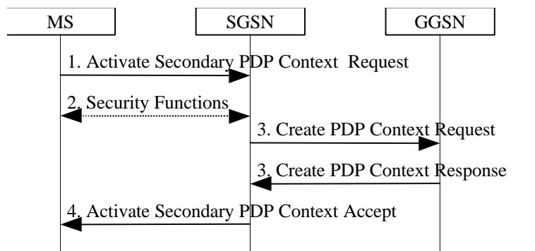
Figure 1: Secondary PDP Context Activation Procedure
