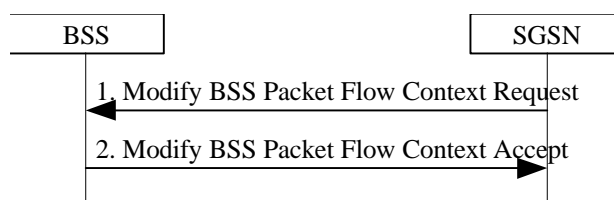
Figure 8: SGSN-Initiated BSS Packet Flow Context Modification Procedure
