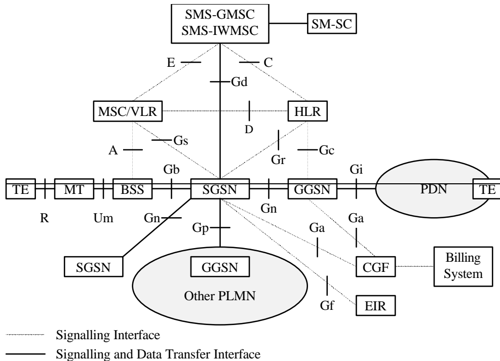
Figure 2: Overview of the Packet Domain Logical Architecture
