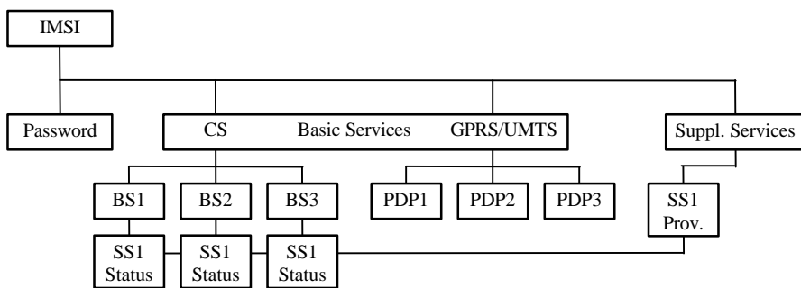
Figure 68: GPRS Subscription Data
