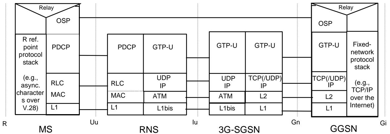
Figure 4: UMTS User Plane for PDP Type OSP
