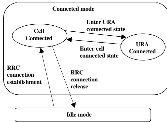
Figure 39: RRC modes, main RRC states and main mode/state transition
