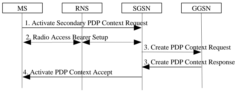
Figure 5: Secondary PDP Context Activation Procedure for UMTS
