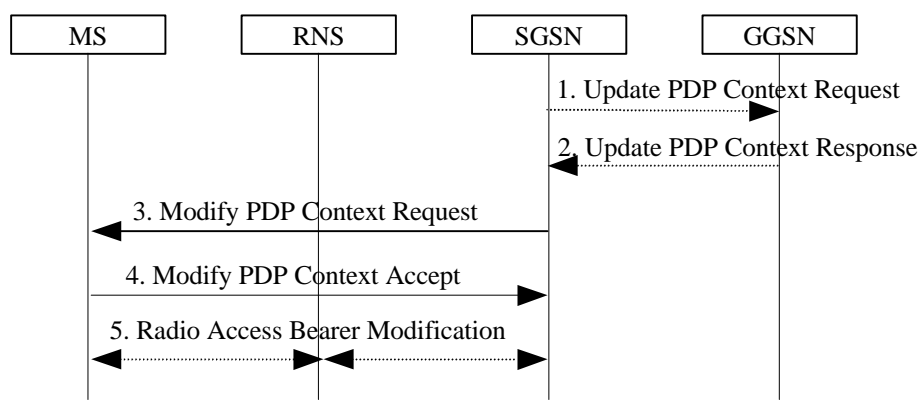
Figure 11: SGSN-Initiated PDP Context Modification Procedure for UMTS
