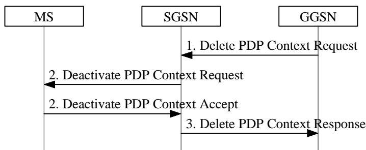
Figure 5: PDP Context Deactivation Initiated by GGSN Procedure
