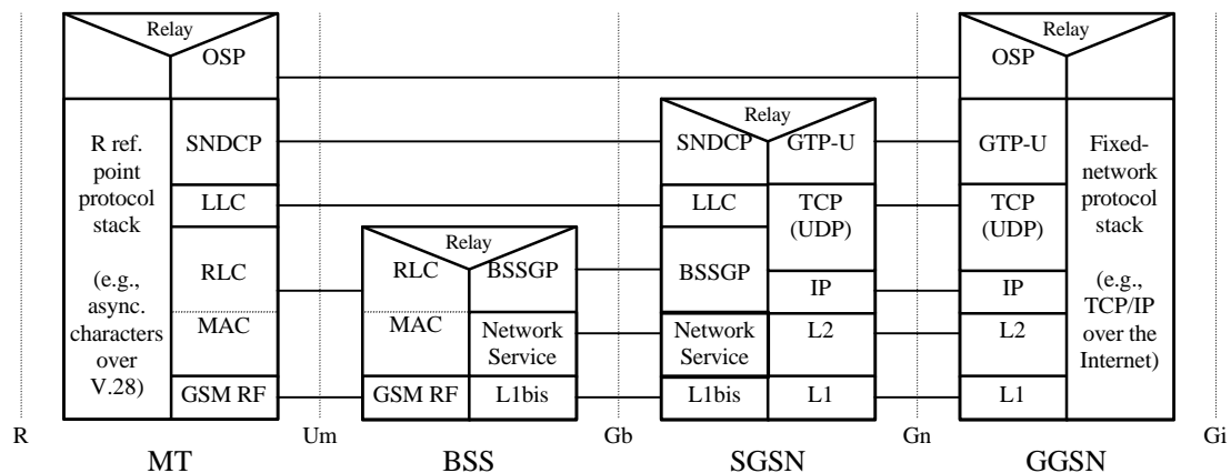
Figure 3: GPRS User Plane for PDP Type OSP Relationship of OSP to the Rest of the GPRS Protocol Architecture
