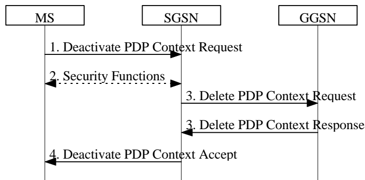
140 141 Figure xx: PDP Context Deactivation Initiated by MS Procedure
