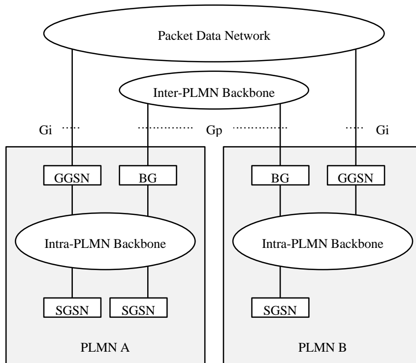
Figure 43: Intra- and Inter-PLMN Backbone Networks
