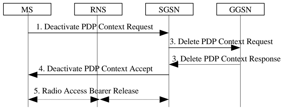
Figure 17: PDP Context Deactivation Initiated by MS Procedure for UMTS
