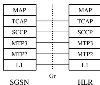
Figure 8 Figure 9: Control Plane SGSN - HLR
