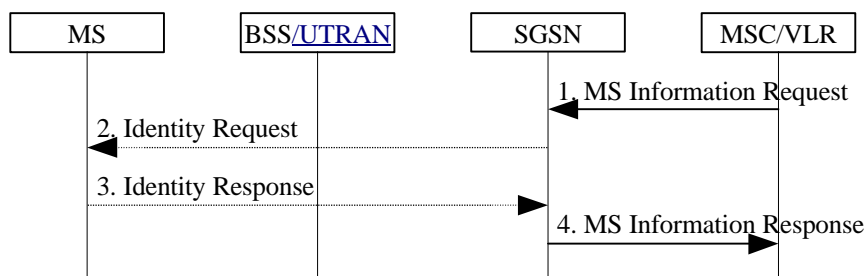
Figure 2: MS Information Procedure
