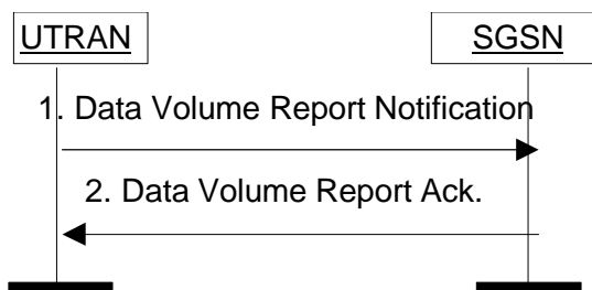
Figure 71: Data Volume Report procedure initiated by RNC
