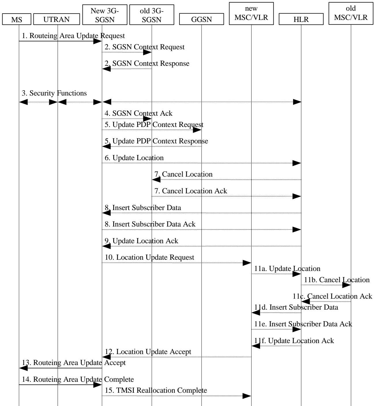
Figure 33: RA Update Procedure in UMTS
