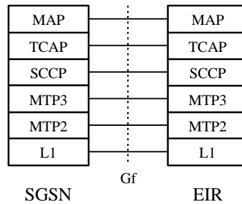
Figure 119: Control Plane SGSN - EIR
