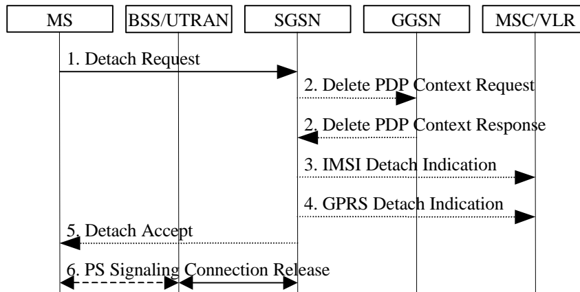
Figure 1: MS-Initiated Combined PS / IMSICS Detach Procedure
