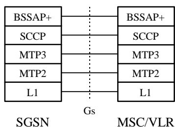
Figure 9 Figure 10: Control Plane SGSN - MSC/VLR
