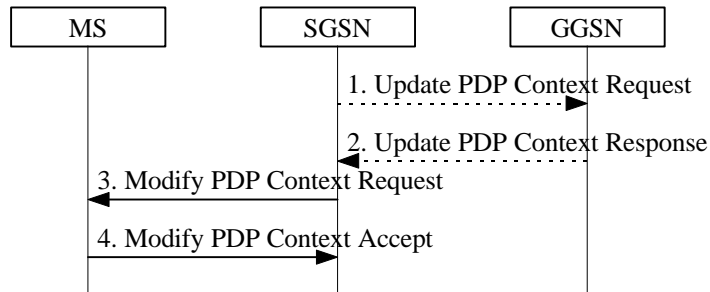
Figure 2: PDP Context Modification Procedure
