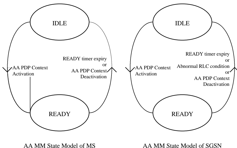
Figure 2: Functional Anonymous Access Mobility Management State Model
