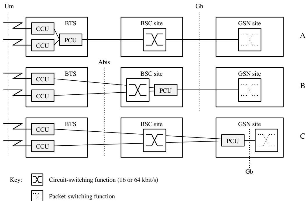
Figure 1: Remote Packet Control Unit (PCU) Positions
