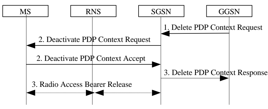
Figure 21: PDP Context Deactivation Initiated by GGSN Procedure for UMTS
