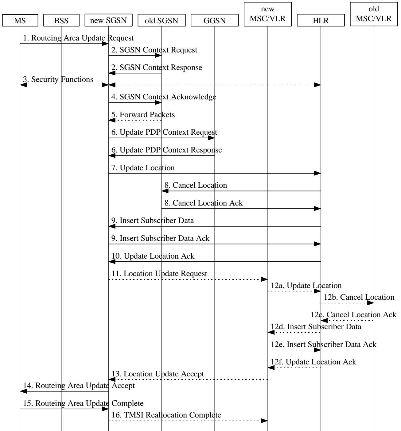
Figure 5: Combined RA / LA Update in the Case of Inter SGSN RA Update Procedure
