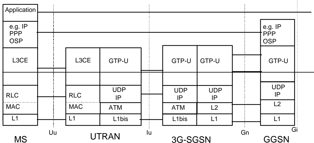
Figure 6: User Plane for UMTS
