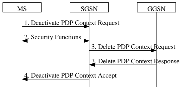
Figure 3: PDP Context Deactivation Initiated by MS Procedure
