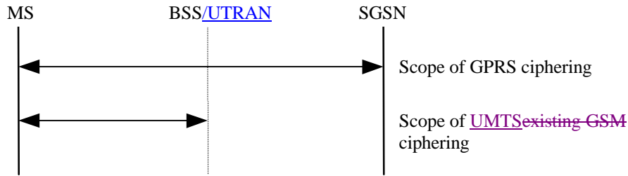
Figure 2: Scope of GPRS Ciphering
