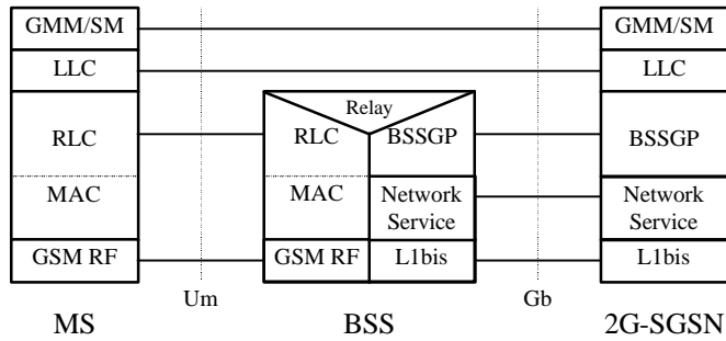
Figure 6 Figure 7 : Control Plane MS – 2G-SSN
