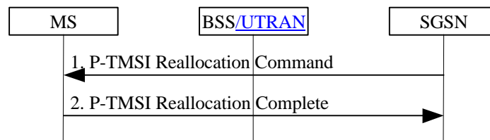
Figure 1: P-TMSI Reallocation Procedure
