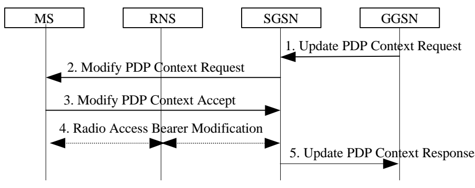
Figure 13: GGSN-Initiated PDP Context Modification Procedure for UMTS
