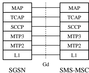
Figure 4012: Control Plane SGSN - SMS-GMSC and SGSN - SMS-IWMSC
