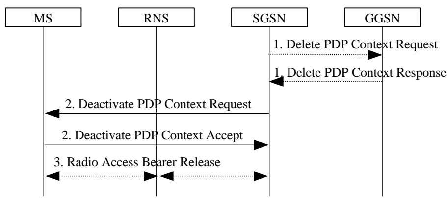
Figure 19: PDP Context Deactivation Initiated by SGSN Procedure for UMTS
