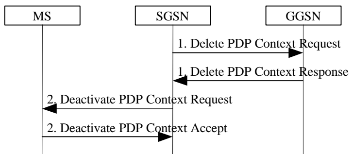
Figure 18: PDP Context Deactivation Initiated by SGSN Procedure for GPRS
