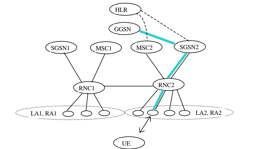
Figure 34 After the SRNS relocation and RA Update
