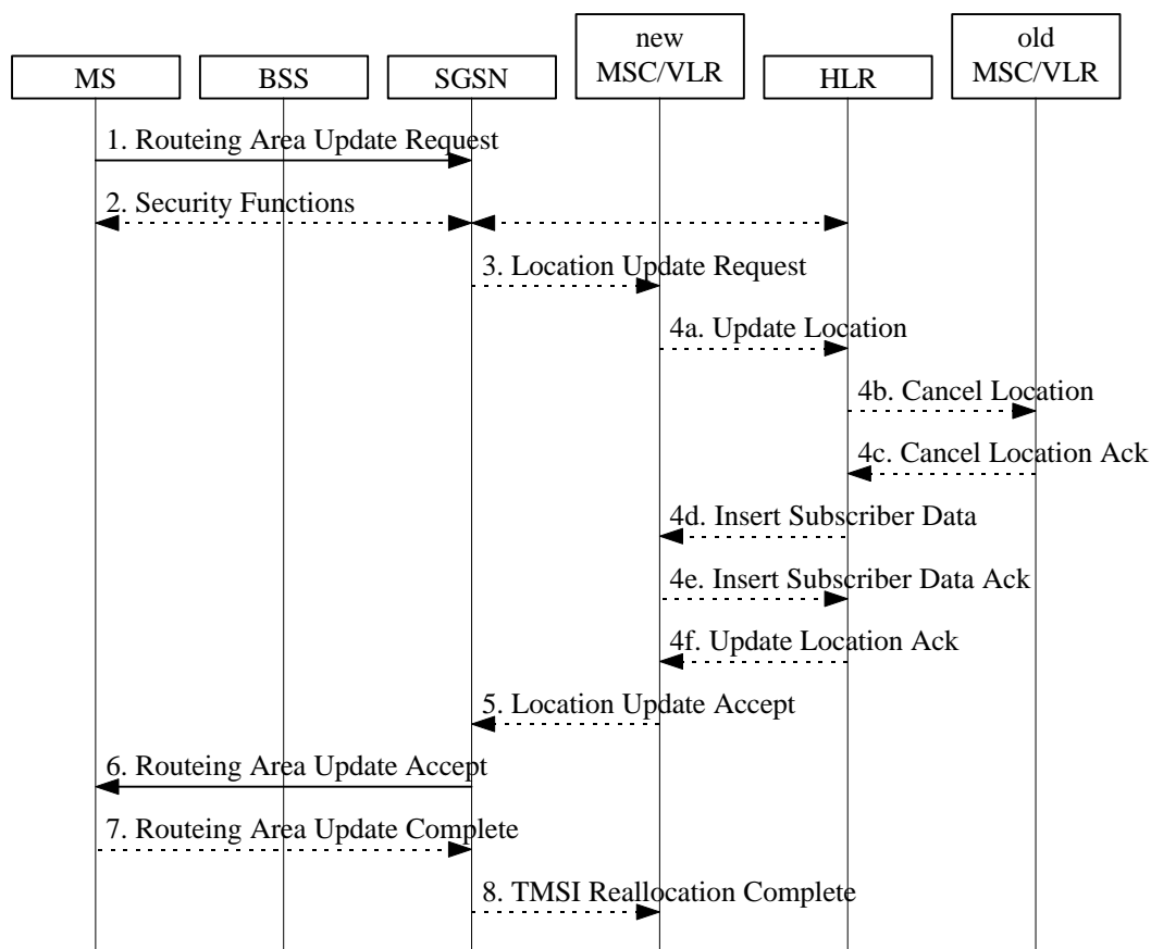
Figure 4: Combined RA / LA Update in the Case of Intra SGSN RA Update Procedure
