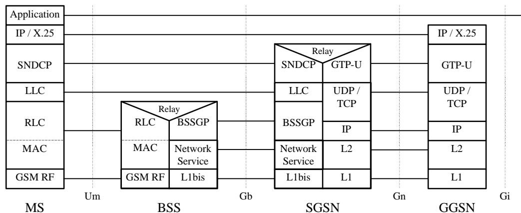
Figure 54: User Plane for GPRS
