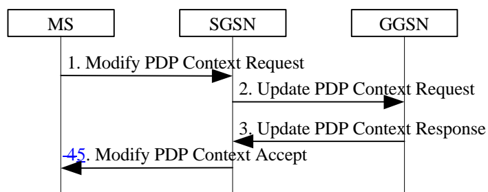
Figure 14: MS-Initiated PDP Context Modification Procedure for GPRS
