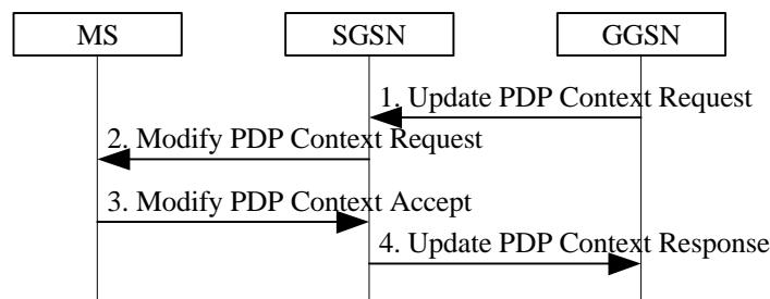
122 123 Figure X: GGSN-Initiated PDP Context Modification Procedure
