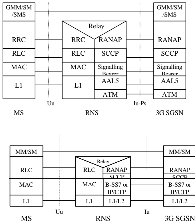
Figure 7 Figure 8 : Control Plane MS - 3G-SSN
