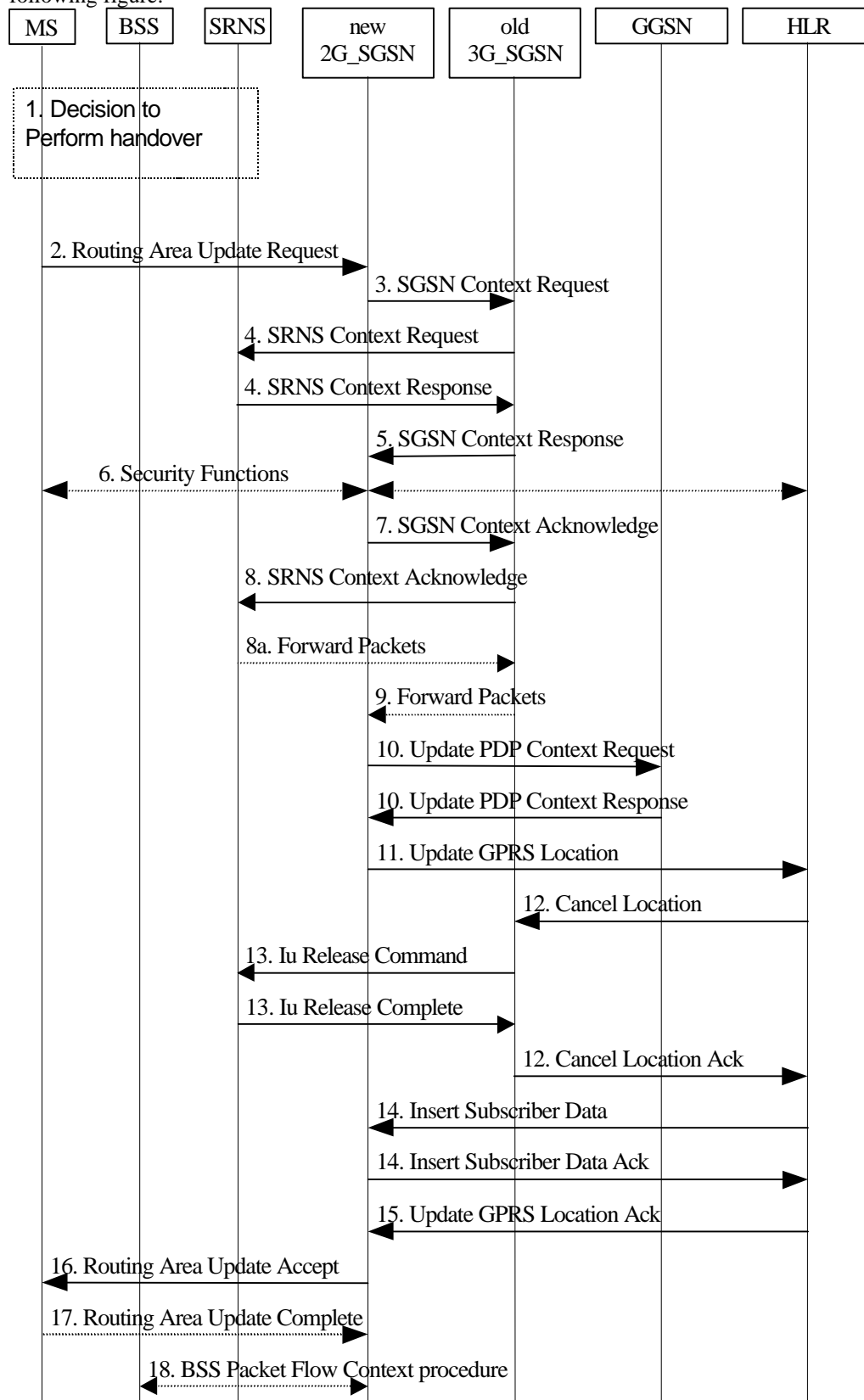
Figure ZZD: UMTS to GSM GPRS, Inter SGSN Routing Area Update Procedure
