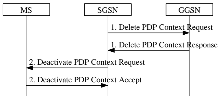
154 155 Figure xx: PDP Context Deactivation Initiated by SGSN Procedure
