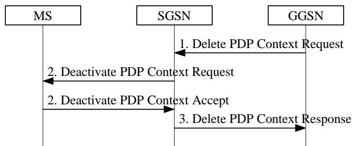
167 168 Figure xx: PDP Context Deactivation Initiated by GGSN Procedure
