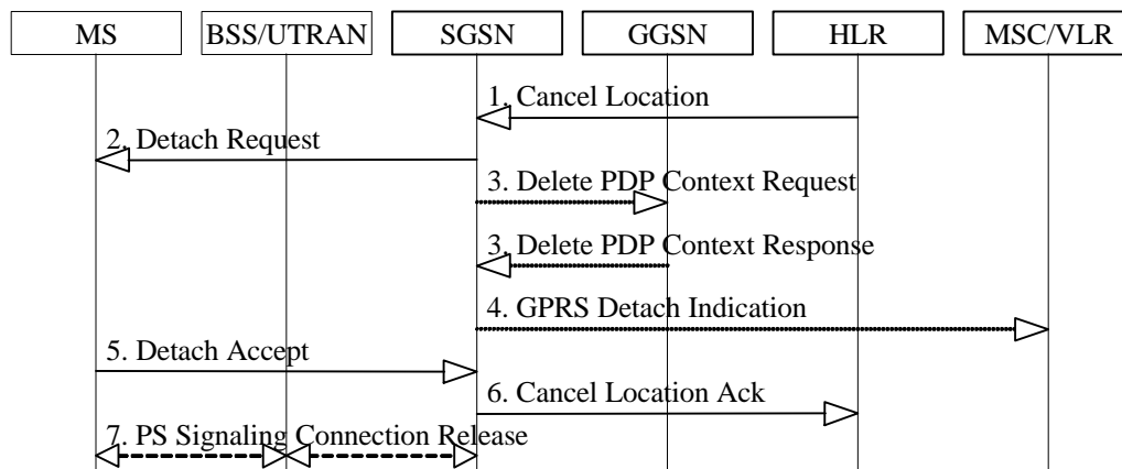
Figure 3: HLR-Initiated PS Detach Procedure
