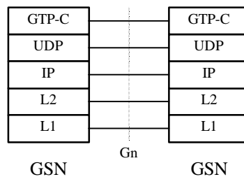
Figure 4413: Control Plane GSN - GSN
