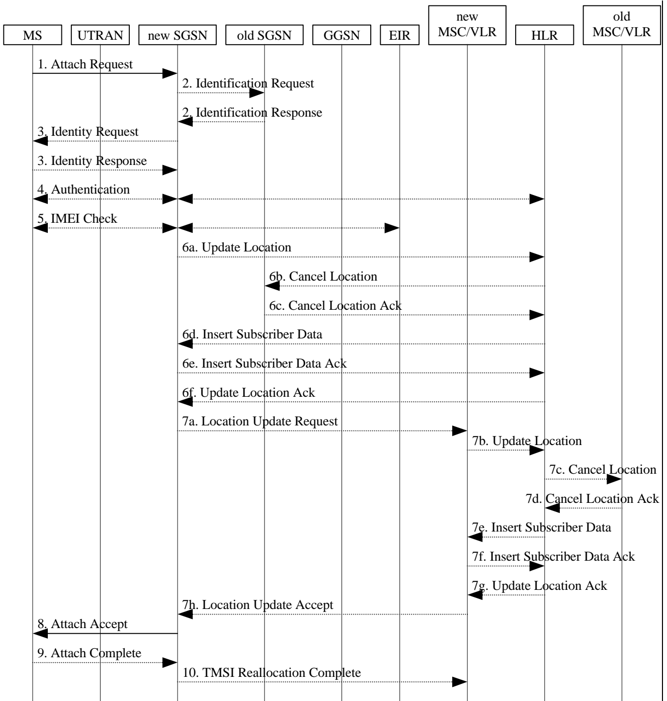
Figure 1: Combined PS / CS Attach Procedure
