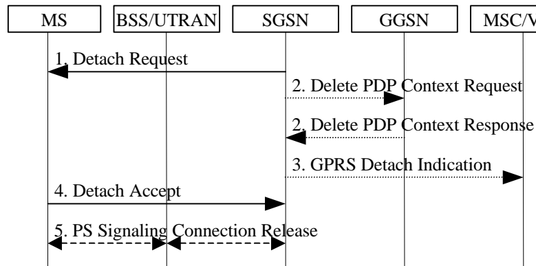
Figure 2: SGSN-Initiated PS Detach Procedure
