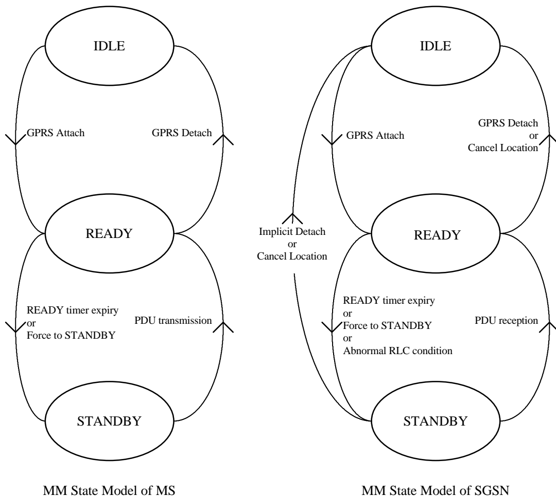
Figure 1: Functional Mobility Management State Model
