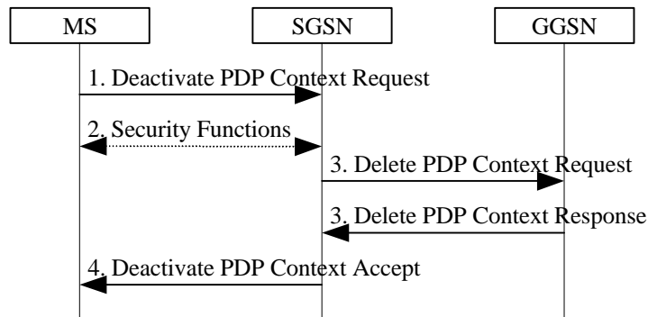
Figure 1: PDP Context Deactivation Initiated by MS Procedure
