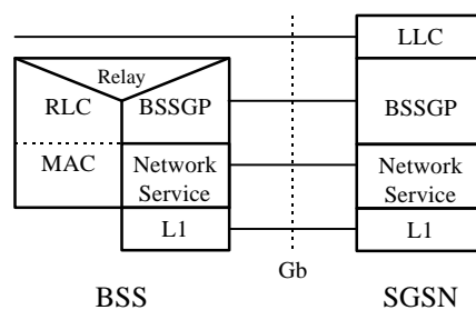
Figure 6: BSSGP Protocol Position
