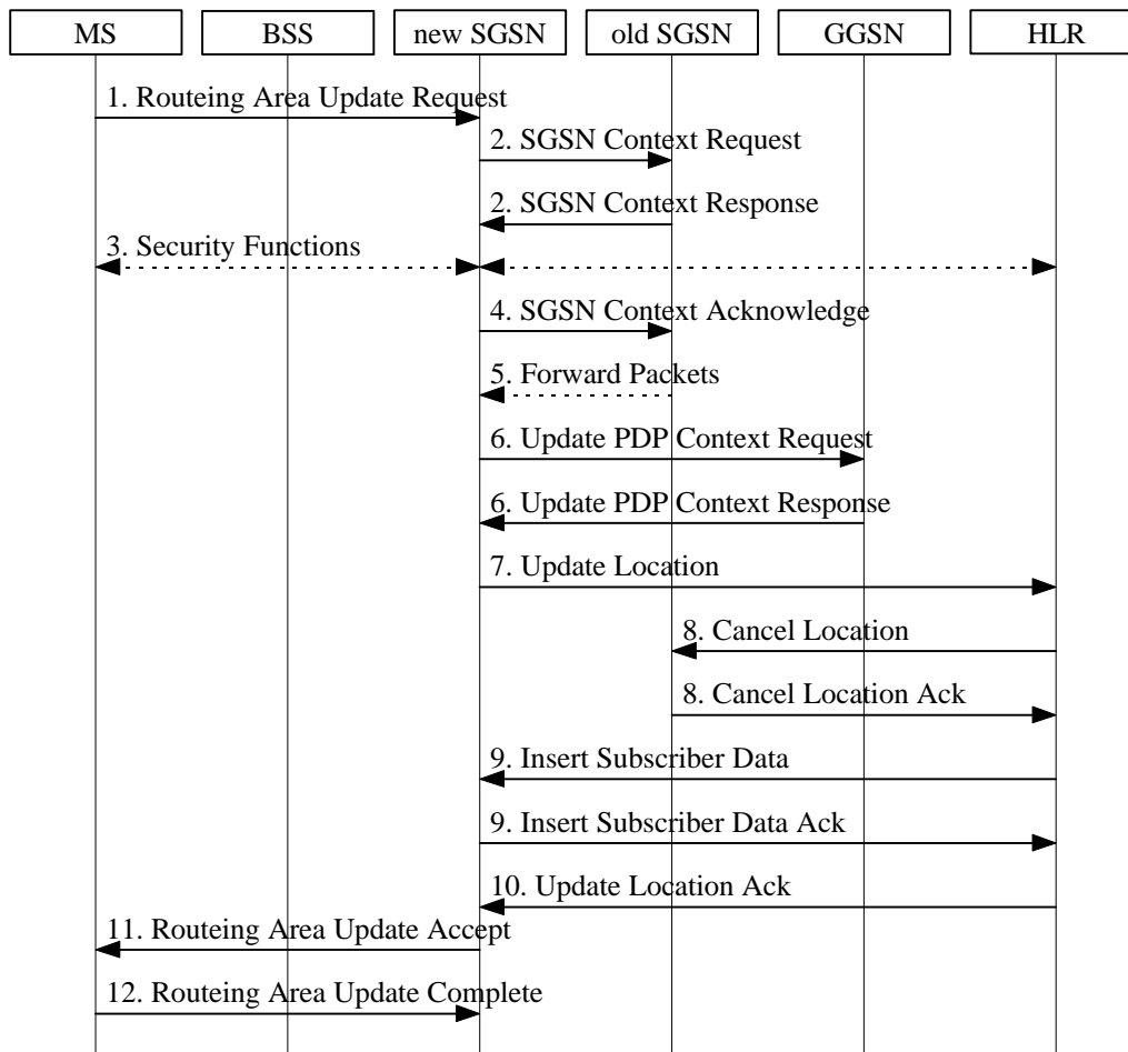
Figure 3: Inter SGSN Routing Area Update Procedure
