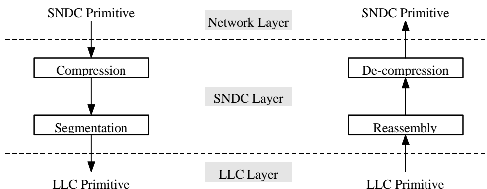
Figure 2: Sequential Invocation of SNDC Functionality
