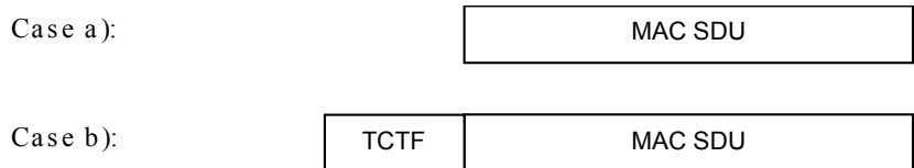
Figure 9.2.1.2.1: MAC PDU formats for BCCH
