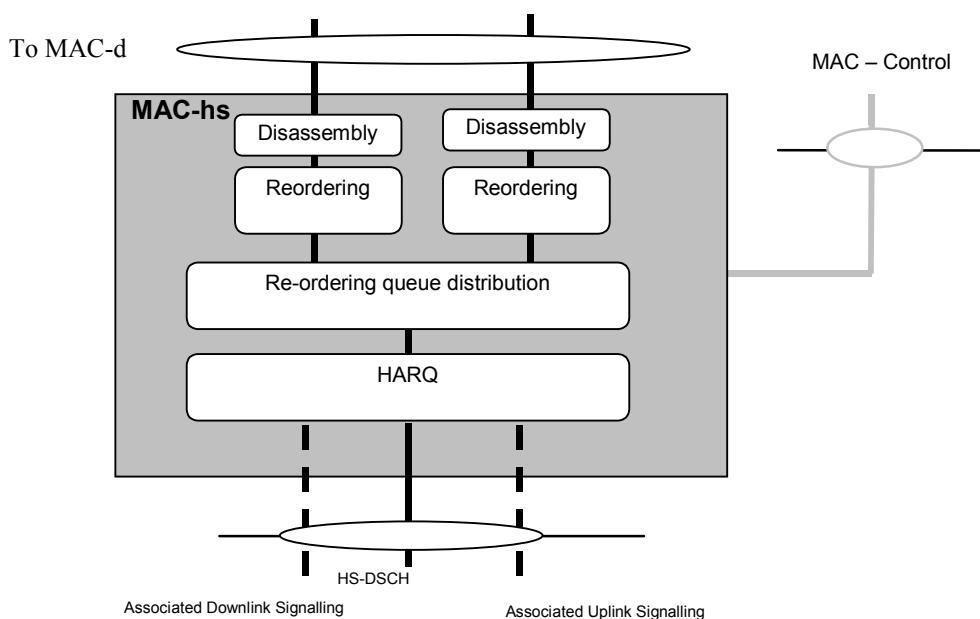
Figure 4.2.3.3.1: UE side MAC architecture / MAC-hs details
