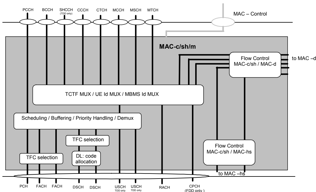
Figure 4.2.4.1.1: UTRAN side MAC architecture / MAC-c/sh/m details
