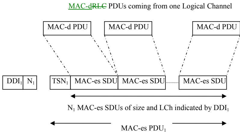
Figure 9.1.5.1: MAC-es PDU
