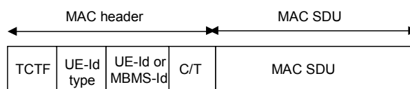
Figure 9.1.2.1: MAC PDU
