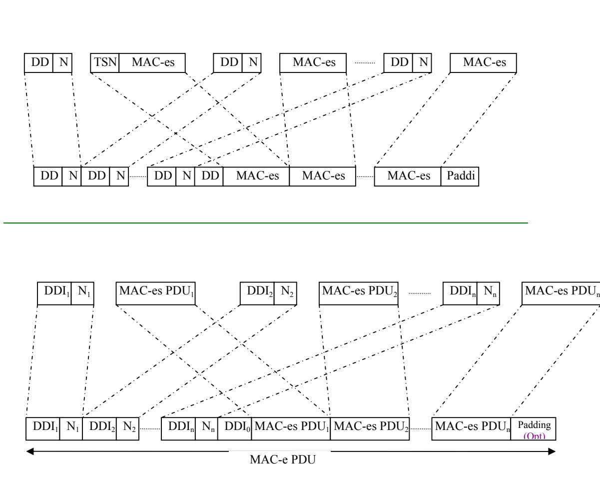
Figure 9.1.5.2: MAC-e PDU
