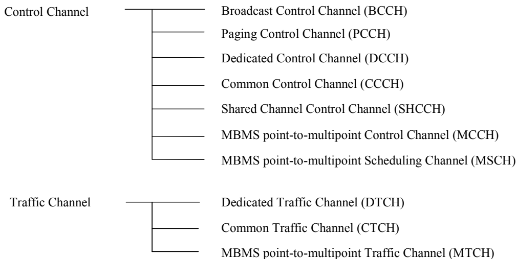
Figure 4.3.2.1: Logical channel structure
