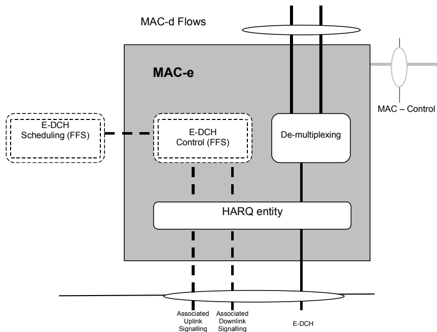
Figure 4.2.4.5-1: UTRAN side MAC architecture / MAC-e details
