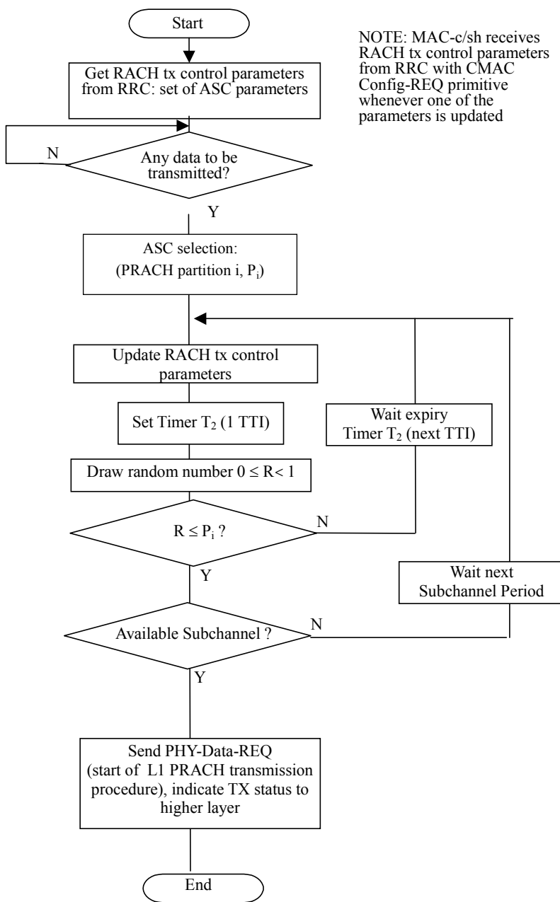
Figure 11.2.3.2: RACH transmission control procedure for TDD (UE side, informative)
