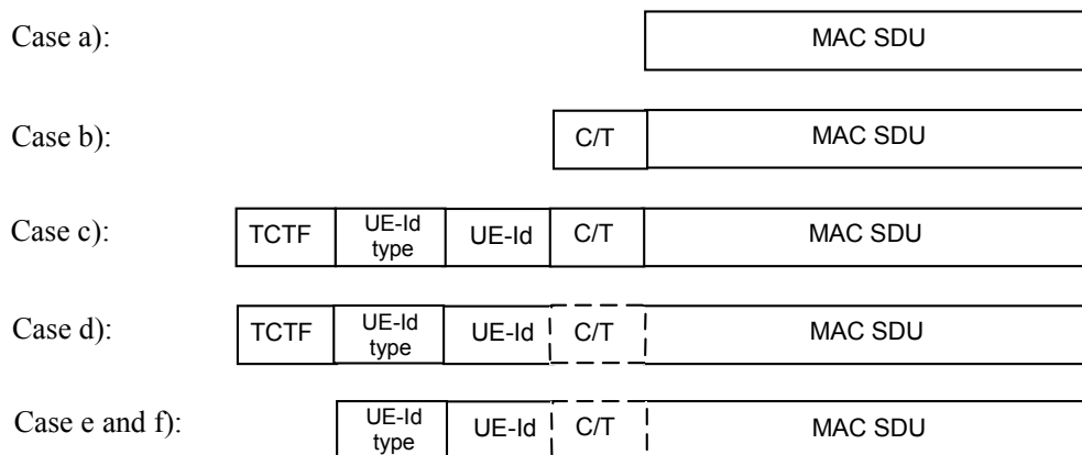
Figure 9.2.1.1.1: MAC PDU formats for DTCH and DCCH
