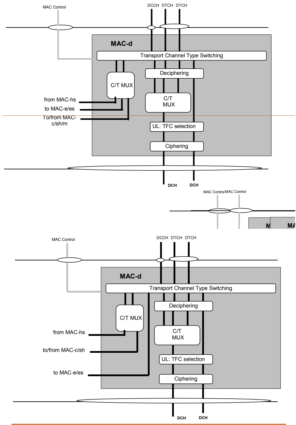
Figure 4.2.3.2.1: UE side MAC architecture / MAC-d details
