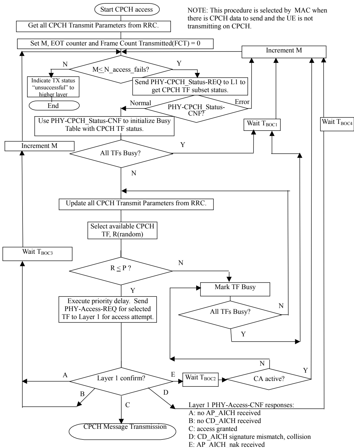
Figure 11.3.1: CPCH transmission control procedure for access (informative)
