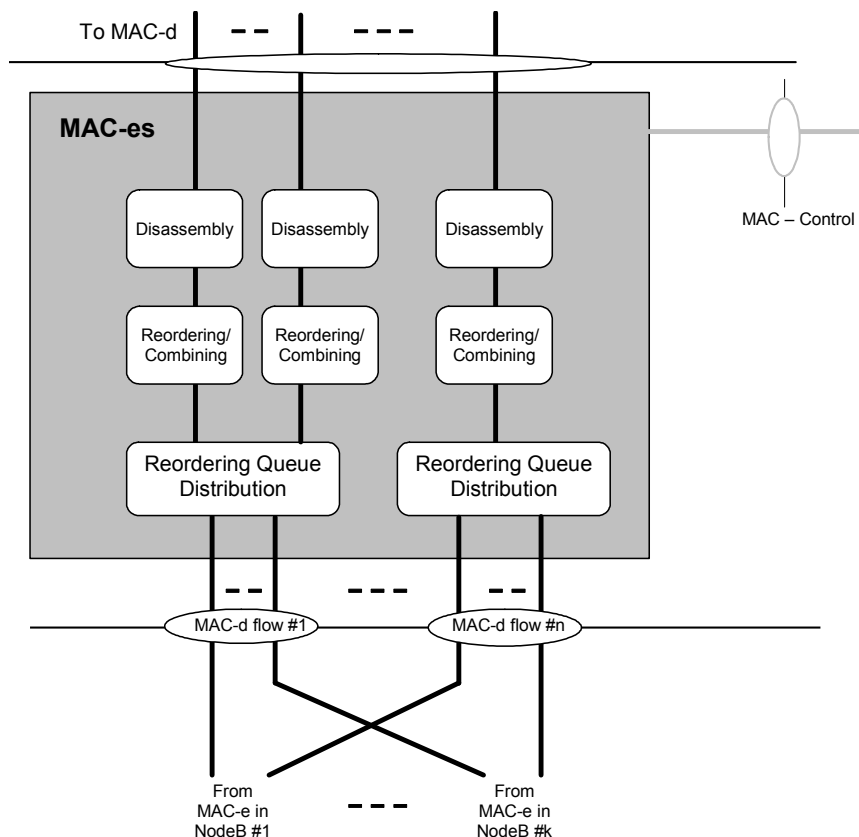
Figure 7.3.5-1: UTRAN side MAC architecture / MAC-es details (SHO case)
