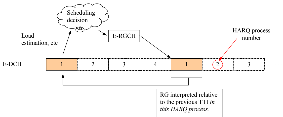
Figure 9.2.1-1: Timing relation for Relative Grant
