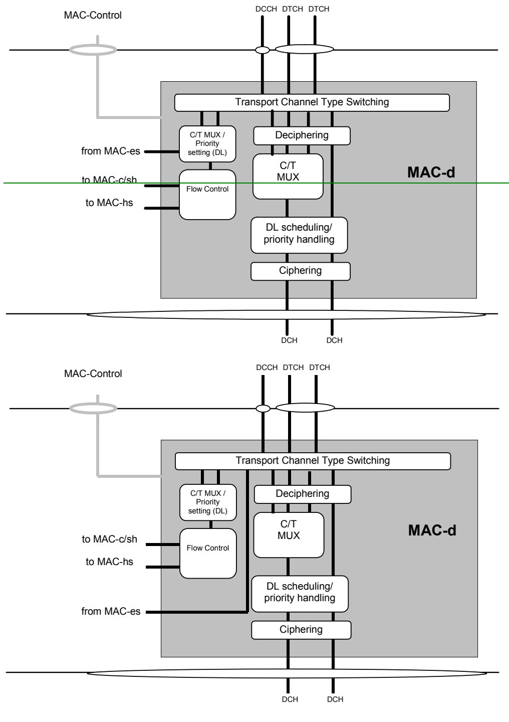
Figure 7.3.2-1: UTRAN side MAC architecture / MAC-d details
