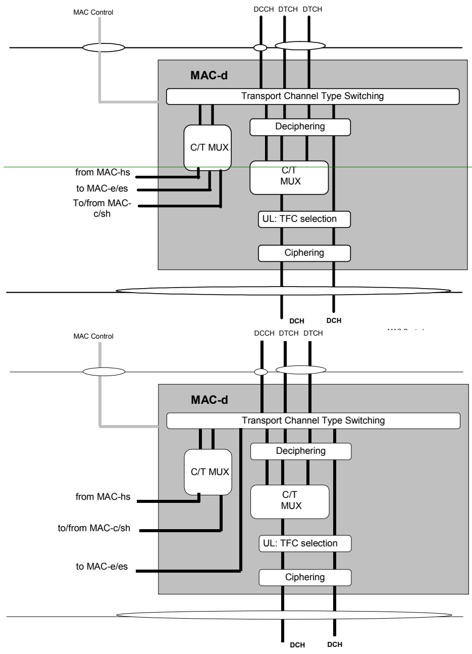
Figure 7.2.2-1: UE side MAC architecture/ MAC-d details
