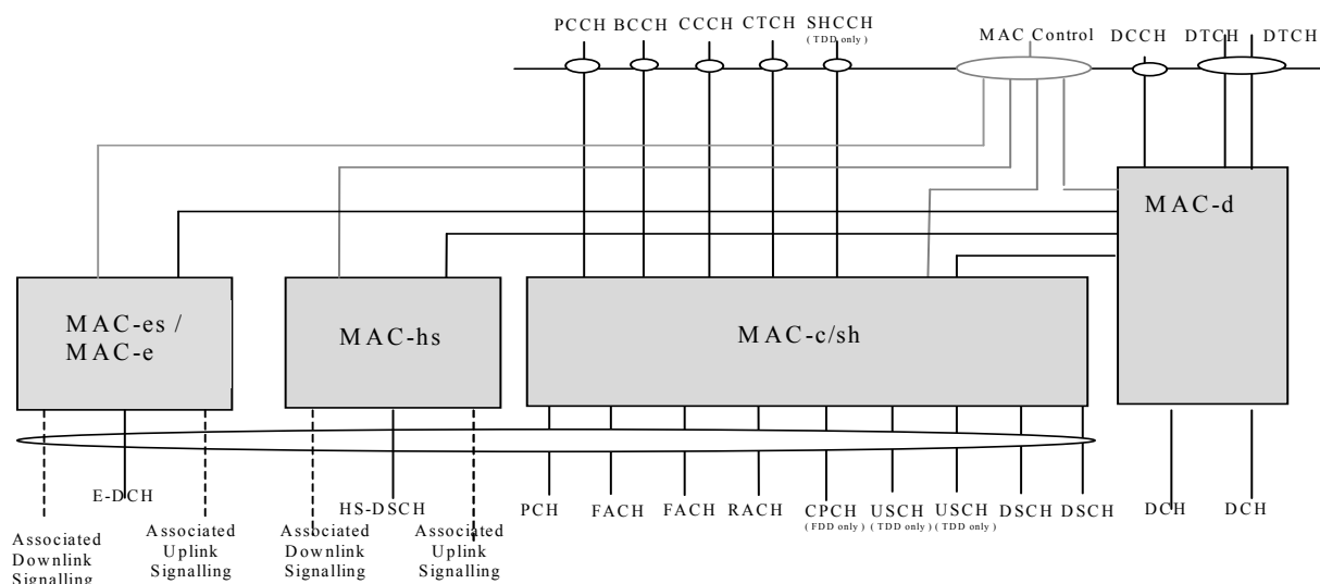
Figure 7.2.1-1: UE side MAC architecture
