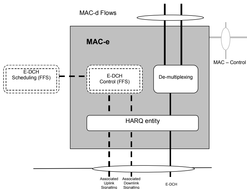
Figure 7.3.6-1: UTRAN side MAC architecture / MAC-e details
