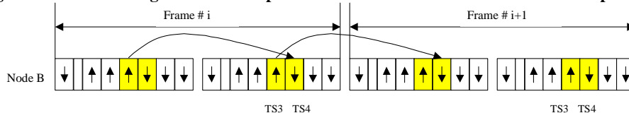
Figure 12. Beam-forming scheme 2 in "special case in conventional scheme" in 1.28Mcps TDD
