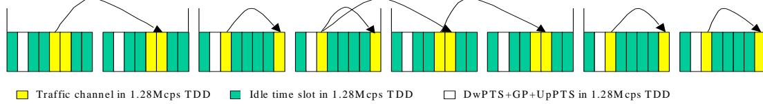
Figure 16. Beam-forming scheme 2 for pattern combination scheme in 1.28Mcps TDD
