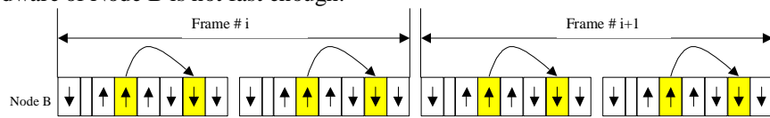
Figure 10. Beam-forming in conventional scheme in 1.28Mcps TDD
