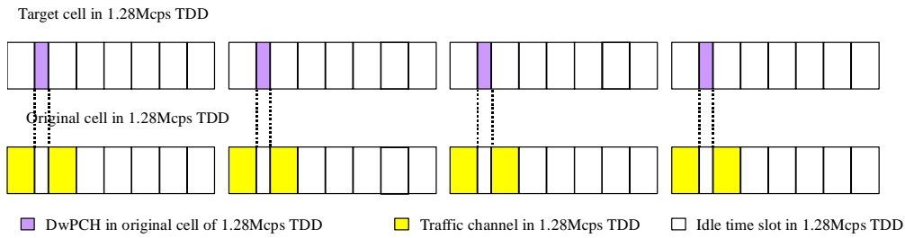
Figure1 Scenario 2 for improvement during 1.28Mcps TDD measurement for coordinated inter-frequency cells
