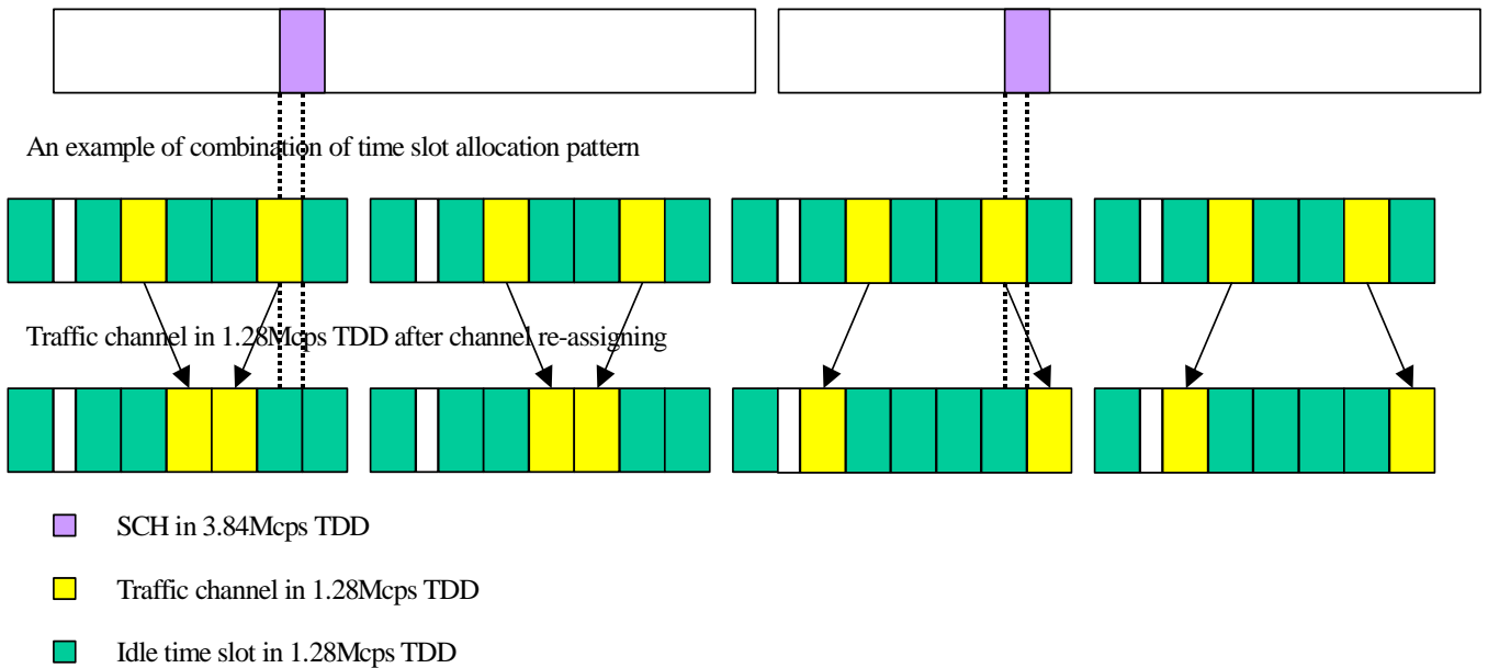
Figure 8. Comparison of monitoring SCH in 3.84Mcps TDD by using combination of time slot allocation pattern and conventional scheme in case 1
