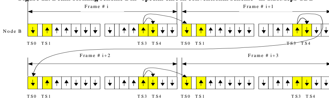
Figure 12. Beam-forming scheme 2 in "special case in conventional scheme" in 1.28Mcps TDD
