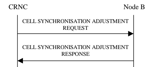
Figure 6 Cell Synchronisation Adjustment, Successful Operation
