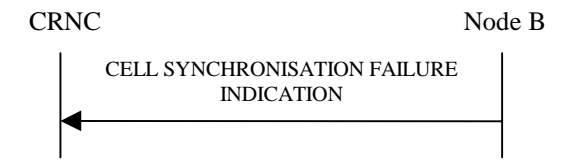
Figure 9 Cell Synchronisation Failure procedure, Successful Operation
