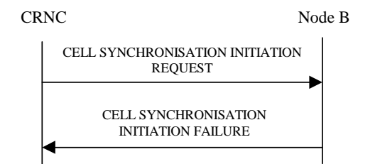
Figure 2 Cell Synchronisation Initiation procedure, Unsuccessful Operation
