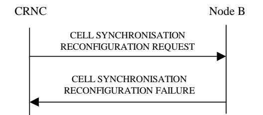
Figure 4 Cell Synchronisation Reconfiguration procedure, Unsuccessful Operation
