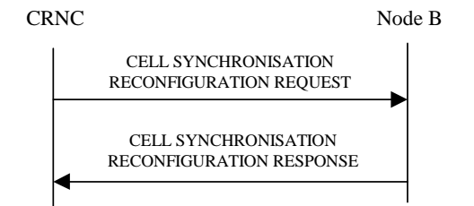
Figure 3 Cell Synchronisation Reconfiguration procedure, Successful Operation
