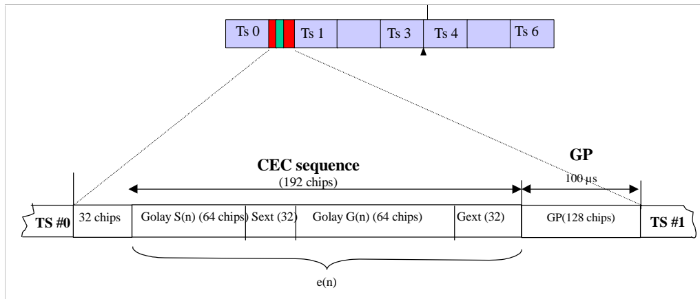
Figure: Structure of the combination of the CEC implementation for Node B synchronization
