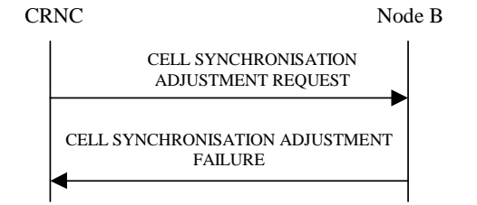
Figure 7 Cell Synchronisation Adjustment, Unsuccessful Operation
