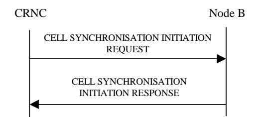
Figure 1 Cell Synchronisation Initiation procedure, Successful Operation
