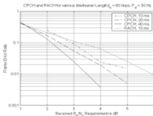
Figure 3: Frame error rate of CPCH and RACH with various interleaver lengths.
