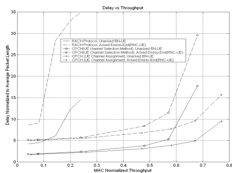
Figure 5: Throughput delay performance of CPCH and RACH.
