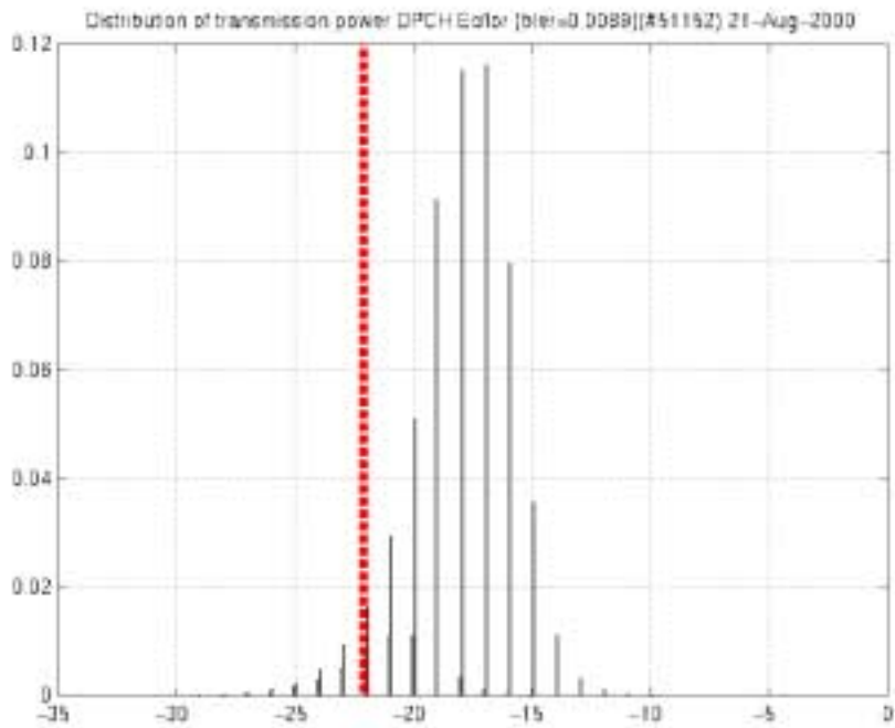
Figure 1549-11: Distribution of transmission power DPCH_{Ec} / I_{or} when compressed mode is on. TGL = 7 slots. The gap in the PDF probably exists because of the bin widths.
