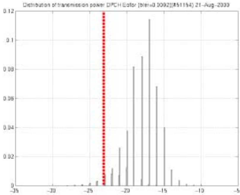
Figure 1519-13: Distribution of transmission power DPCH_{Ec} / I_{or} when compressed mode is on. TGL = 14 slots. The gap in the PDF probably exists because of the bin widths.
