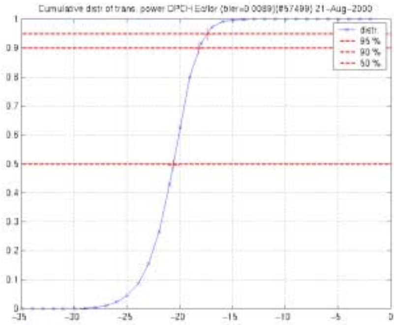
Figure 1549-8: Cumulative distribution of transmission power DPCH_{Ec} / I_{or} when compressed mode is off.
