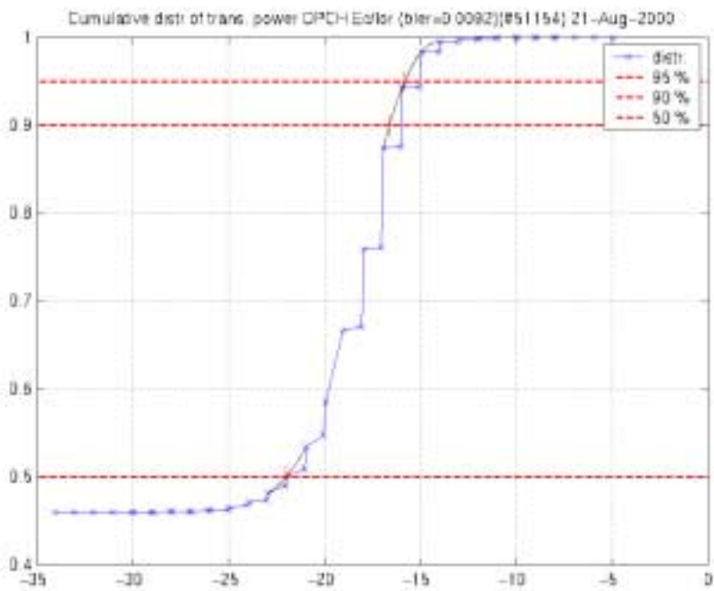
Figure 1519-14: Cumulative distribution of transmission power DPCH_{Ec} / I_{or}
