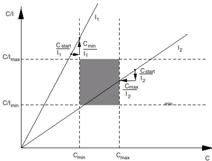
Figure 16-23 Example of power algorithm
