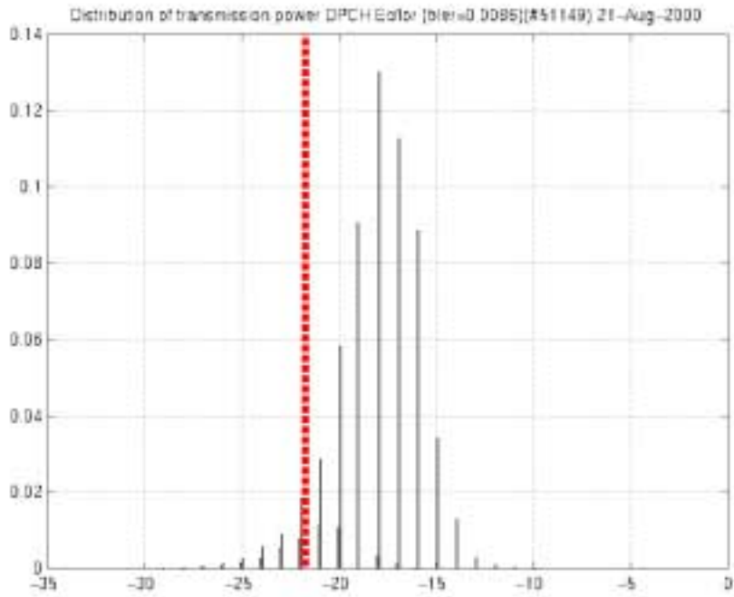
Figure 1519-9: Distribution of transmission power DPCH_{Ec} / I_{or} when compressed mode is on. TGL = 4 slots. The gap in the PDF probably exists because of the bin widths.
