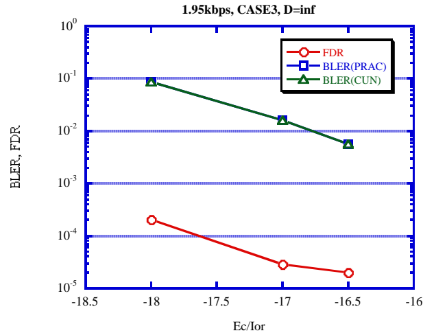
Figure 1519-6 Ec/Ior vs. BLER(CASE3, 1.95k)
