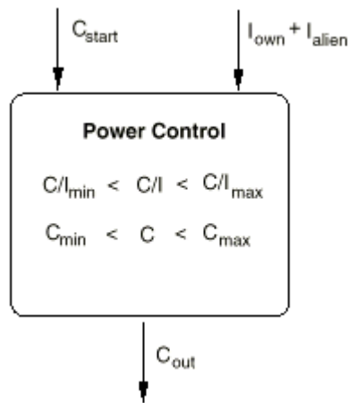
Figure 6-11 C/I based Power Control algorithm
