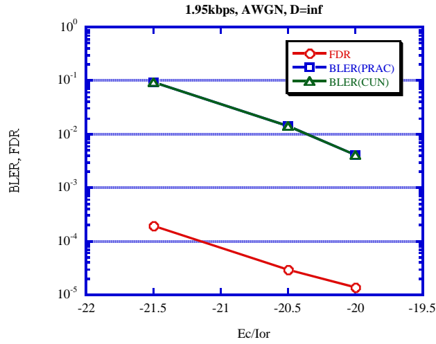
Figure 1549-3 Ec/Ior vs. BLER(STATIC, 1.95k)
