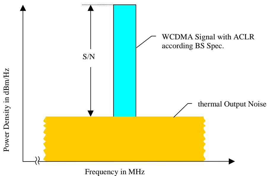
Fig. 4.4.2: Repeater output frequency spectrum.
