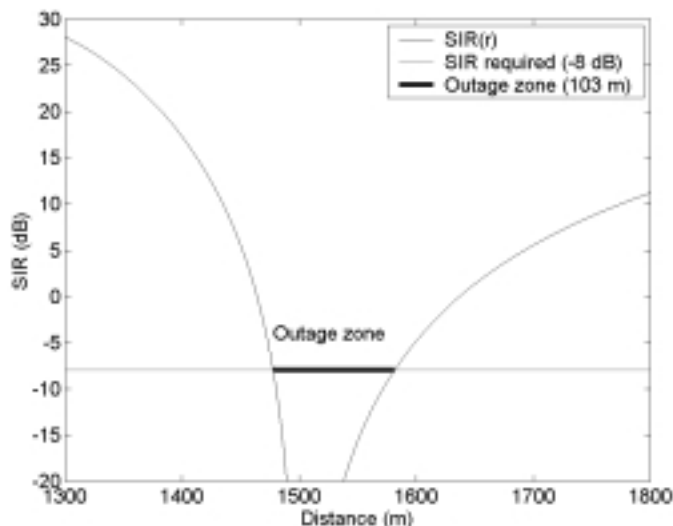
Figure 6.1.2: The figure shows the signal-to-interference (SIR) ratio and the threshold of -8 dB. The outage zone where the SIR drops below this threshold is around 103 m.
