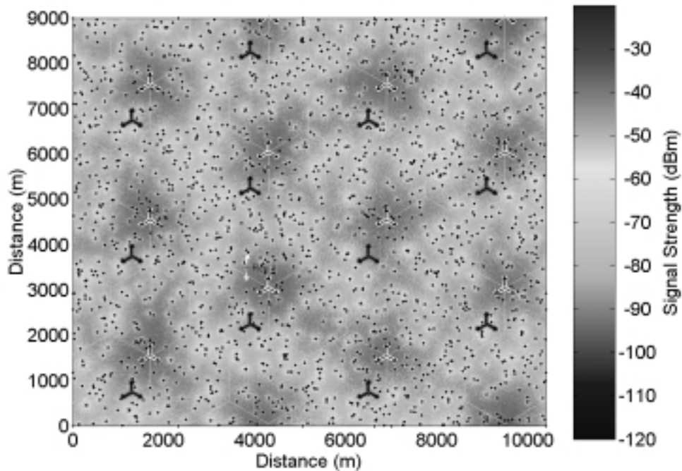
Figure 6.4.2: An illustration of the uncoordinated scenario. The repeater's position is indicated with a red + (positioned @ 3800; 3500 m). The figure also shows the total uplink power in operator B's network.
