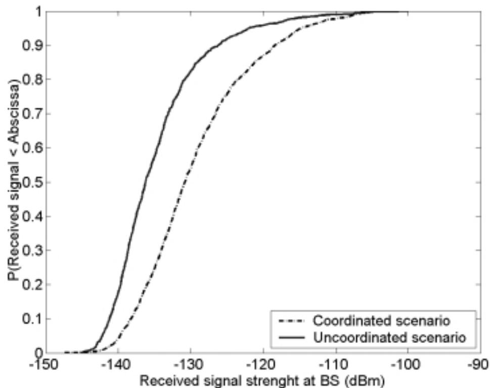
Figure 6.4.3: Cumulative distribution function of the received signal strength at operator BS base station due to the repeaters out of band gain. The picture shows results for both uncoordinated and co-ordinated scenario. The 99% level is -110 dBm and -107 dBm for the uncoordinated and co-ordinated scenario, respectively.
