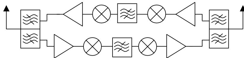
Figure 4.4.1: Simplified Repeater model.
