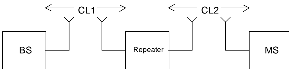
Fig. 6.2.1: Schematic illustration of the radio link between BS and MS via a Repeater.
