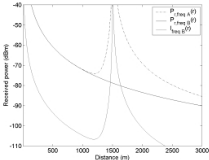
Figure 6.1.1: Simulation on the received average power from a base station on two 5 MHz channels, frequency A and B. The output power is the same for both base stations. P_{r, \text{freqB}} represents a signal on frequency B and P_{r, \text{freqA}} on frequency A where a repeater is used. I_{\text{freqB}} indicates the interference on frequency B that the base station and repeater on frequency A have produced.
