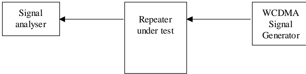
Figure 7: Measuring system set-up for modulation accuracy: peak code domain error.
