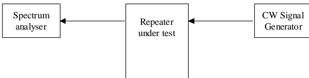
Figure 3: Measuring system set-up for out of band gain.
