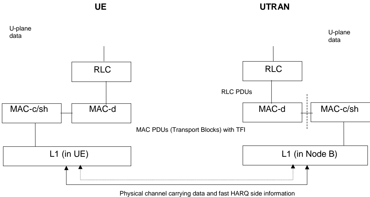
Figure 2 Protocol stack overview for fast hybrid ARQ type II/III.
