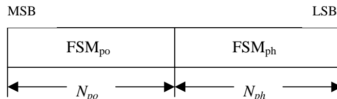
Figure 2. Format of feedback signaling message. FSM_{po} transmits the power setting and FSM_{ph} the phase setting.
