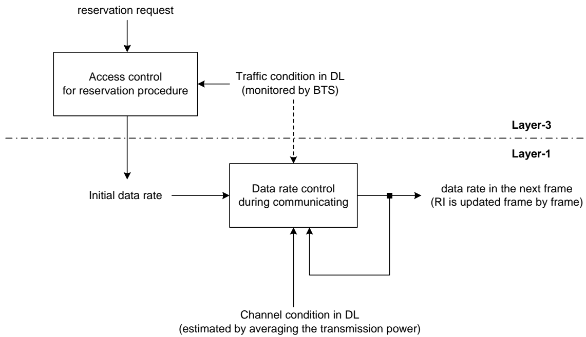
Figure 12: Data rate control diagram
