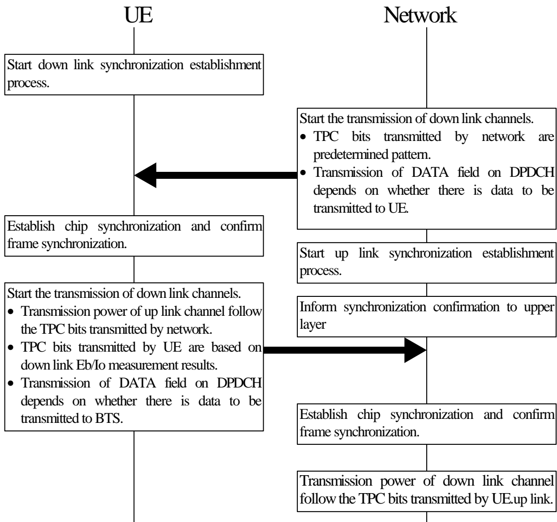
Figure 1: Synchronization Establishment Flow of Dedicated Channels
