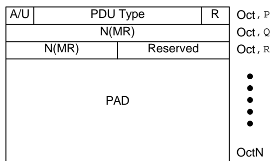
Figure Error! Style not defined.-Error! Bookmark not defined.. BGAK PDU
