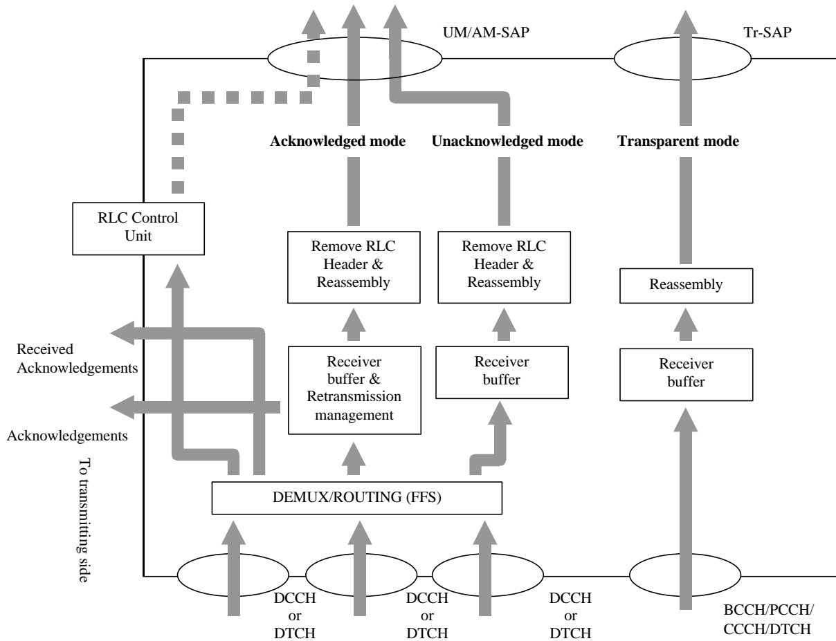
Figure Error! Style not defined.-Error! Bookmark not defined.. RLC receiver entity.
