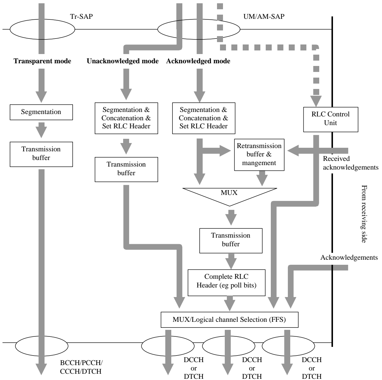
Figure Error! Style not defined.-Error! Bookmark not defined.. The transmitting side of a RLC entity.
