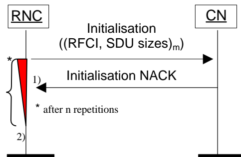
Figure x+1. Unsuccessful initialisation of Iu UP: 1) n negative acknowledgment or 2) n timer expiries
