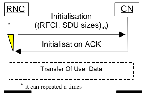
Figure x. Successful Initialisation of Iu UP for m RFCIs
