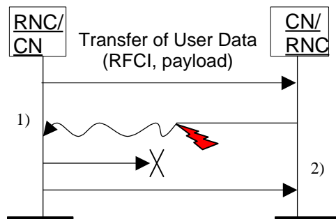
Figure x. Unsuccessful Transfers of User Data: 1) Corrupted Frame, 2) Detection of Frame loss
