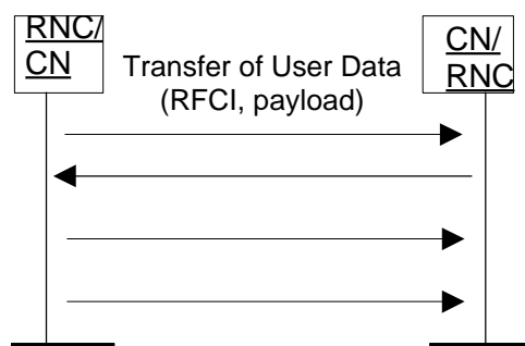
Figure x. Successful Transfers of User Data
