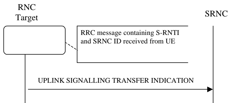
Figure 9-8: An example RNSAP message flow at I_{ur} interface for Uplink Signalling Transfer
