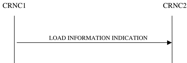
Figure 9-x: An example RNSAP message flow at I_{ur} interface for Load Information.
