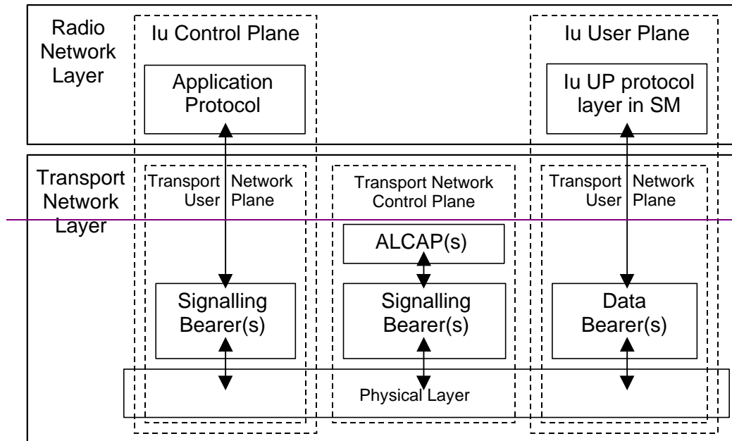
Figure 2: Iu -UP protocol layer interfaces in Support Mode
