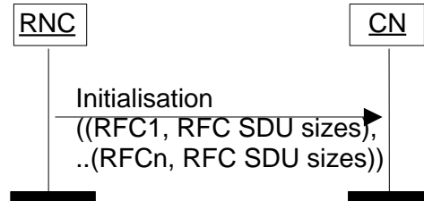
Figure x. Initialisation of Iu UP for n RFCs
