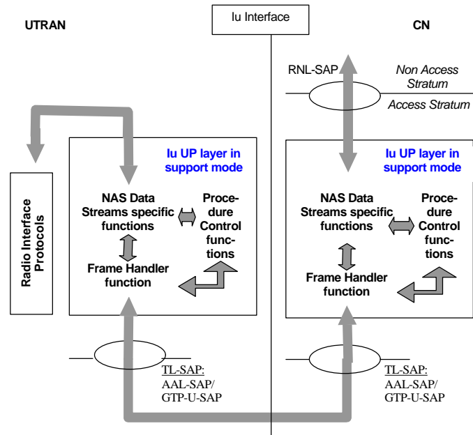
Figure 5: Functional model of the lu UP protocol layer in Support mode
