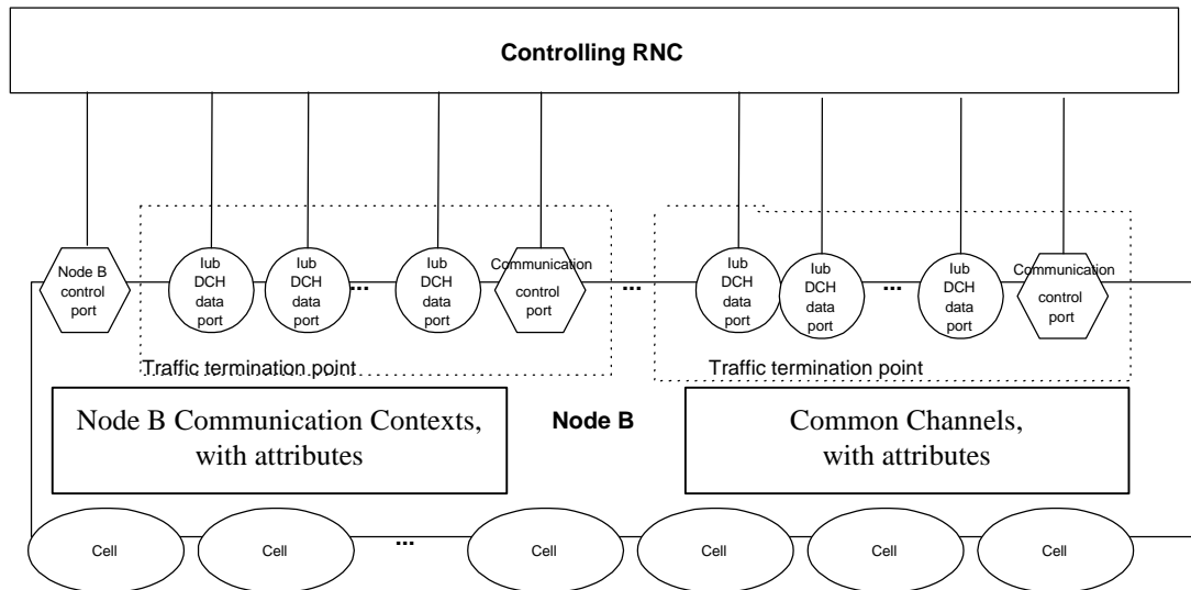
Figure 18. Logical Model of Node B
