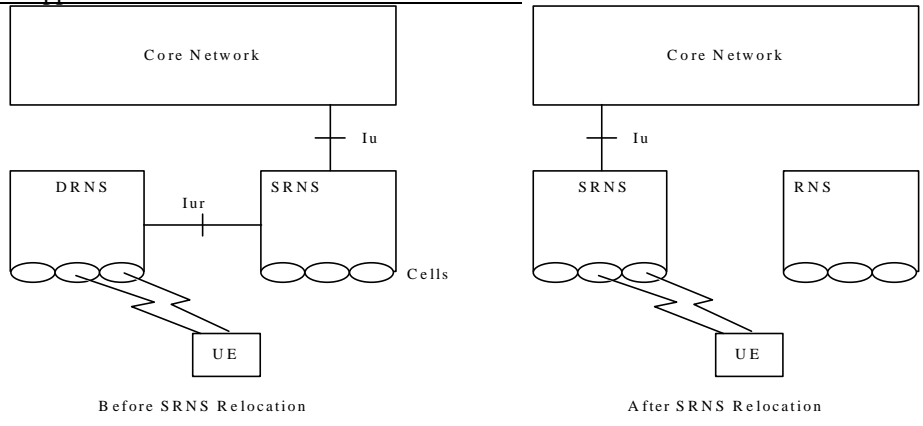
Figure 14. Serving RNS Relocation
