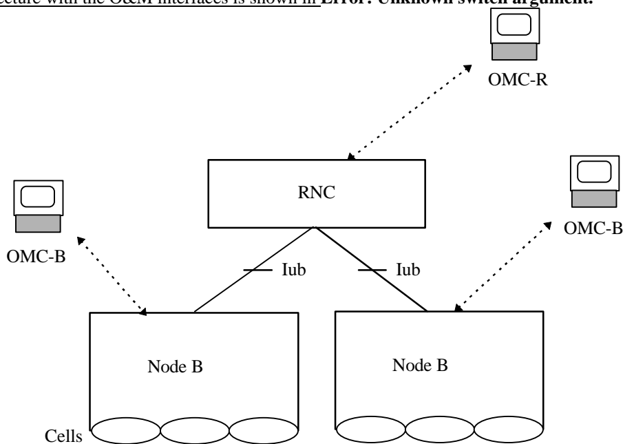
Figure 13.RNS architecture with O&M interfaces
