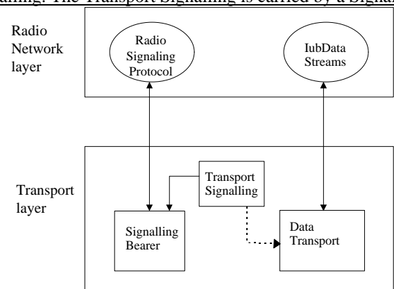
Figure 19. Separation of Radio Network protocols and transport over Iub
