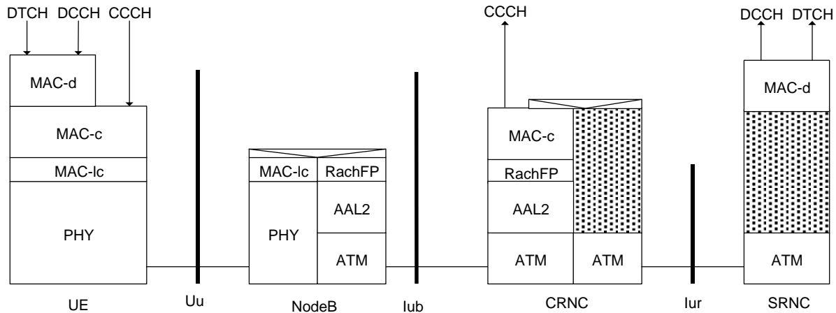
Figure 21. shows the protocol model for the RACH transport channel with separate Controlling and Serving RNC. In this case, Iur RACH Frame Protocol (DchFP) is used to interwork the Common MAC (MAC-c) at the Controlling RNC with the Dedicated MAC (MAC-d) at the Serving RNC (The exact Iur RACH Frame Protocol is FFS)
