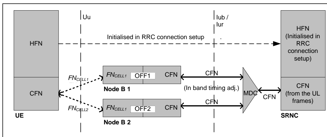
Figure 12. UE-UTRAN synchronisation
