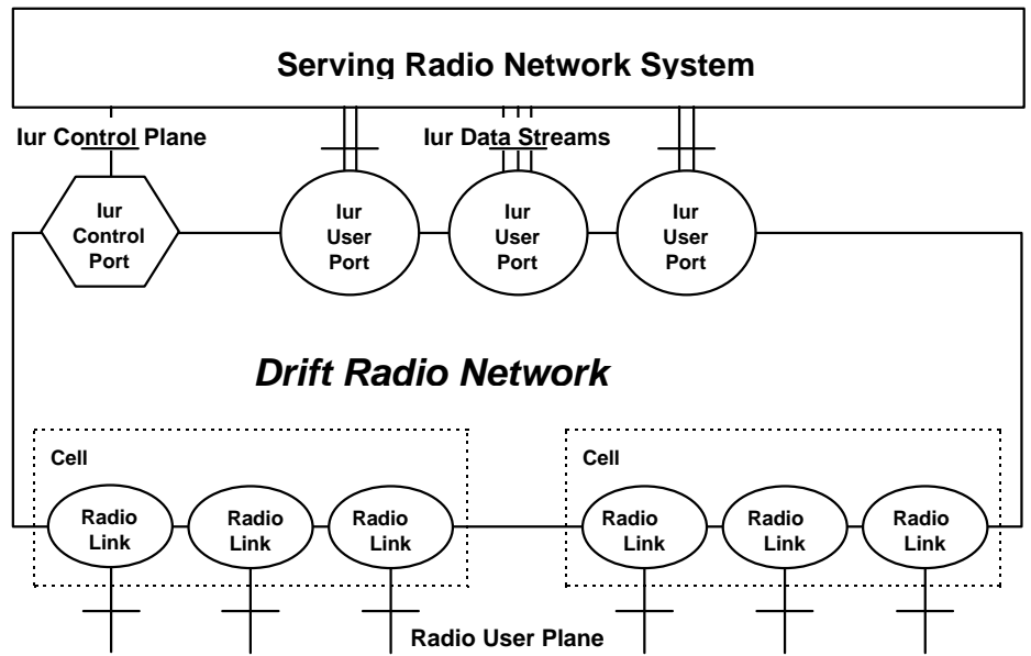
Figure 16. Drift RNS Logical Model
