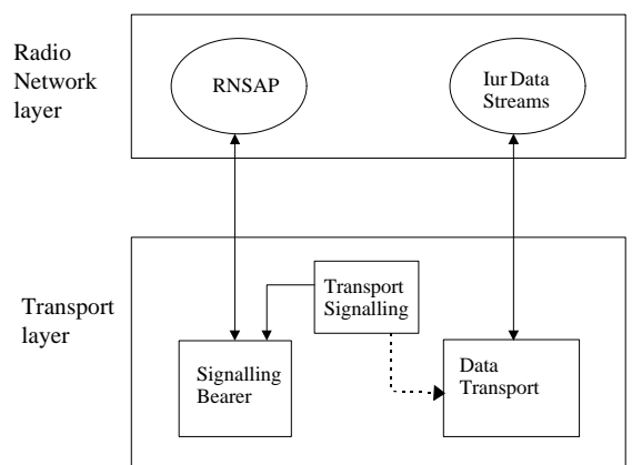
Figure 17. Separation of RNSAP and transport over Iur
