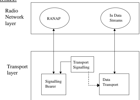
Figure 15. Separation of RANAP and transport over Iu
