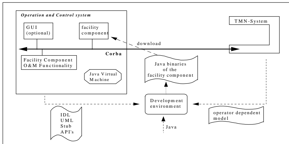
Figure 2 Use of Java to realise a secure "download mechanism"
