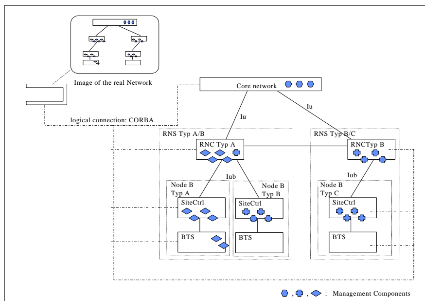
Figure 3: A management architecture without dedicated Operation and control systems
