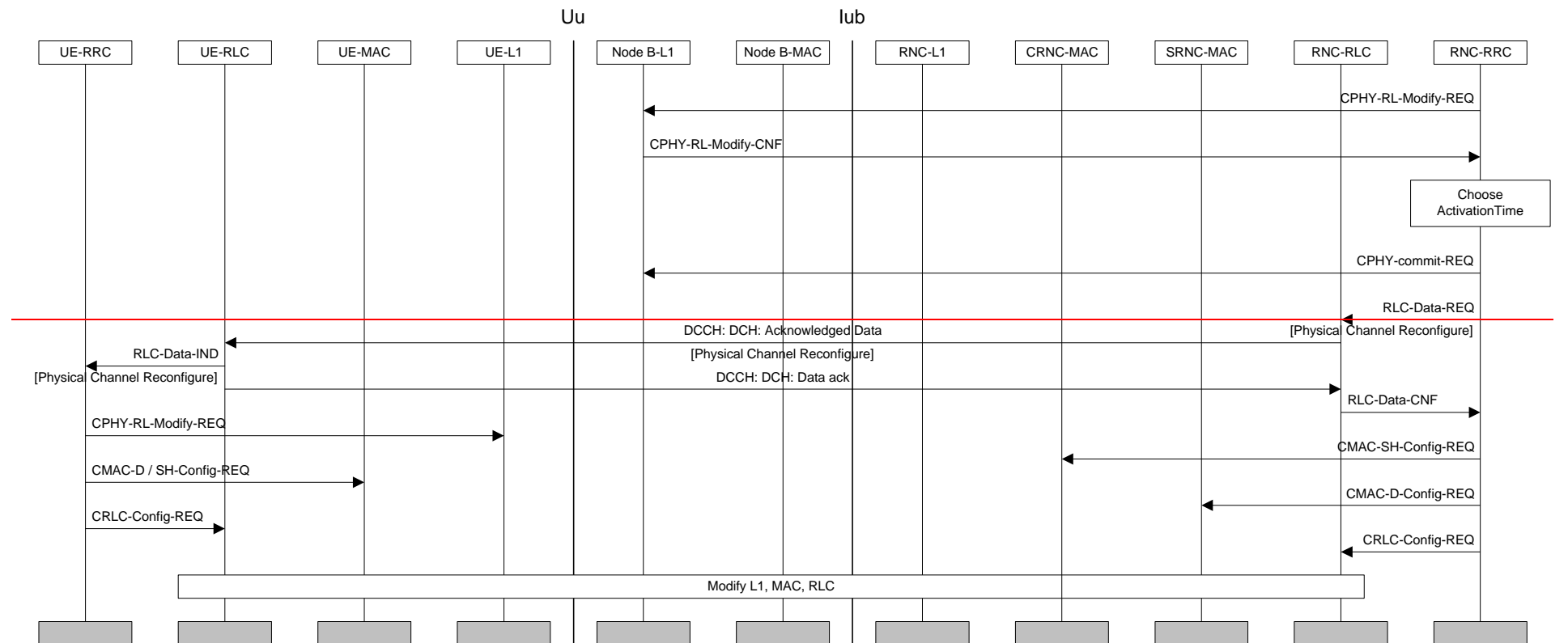
Figure 19: UE-terminated synchronised DCH Modify
