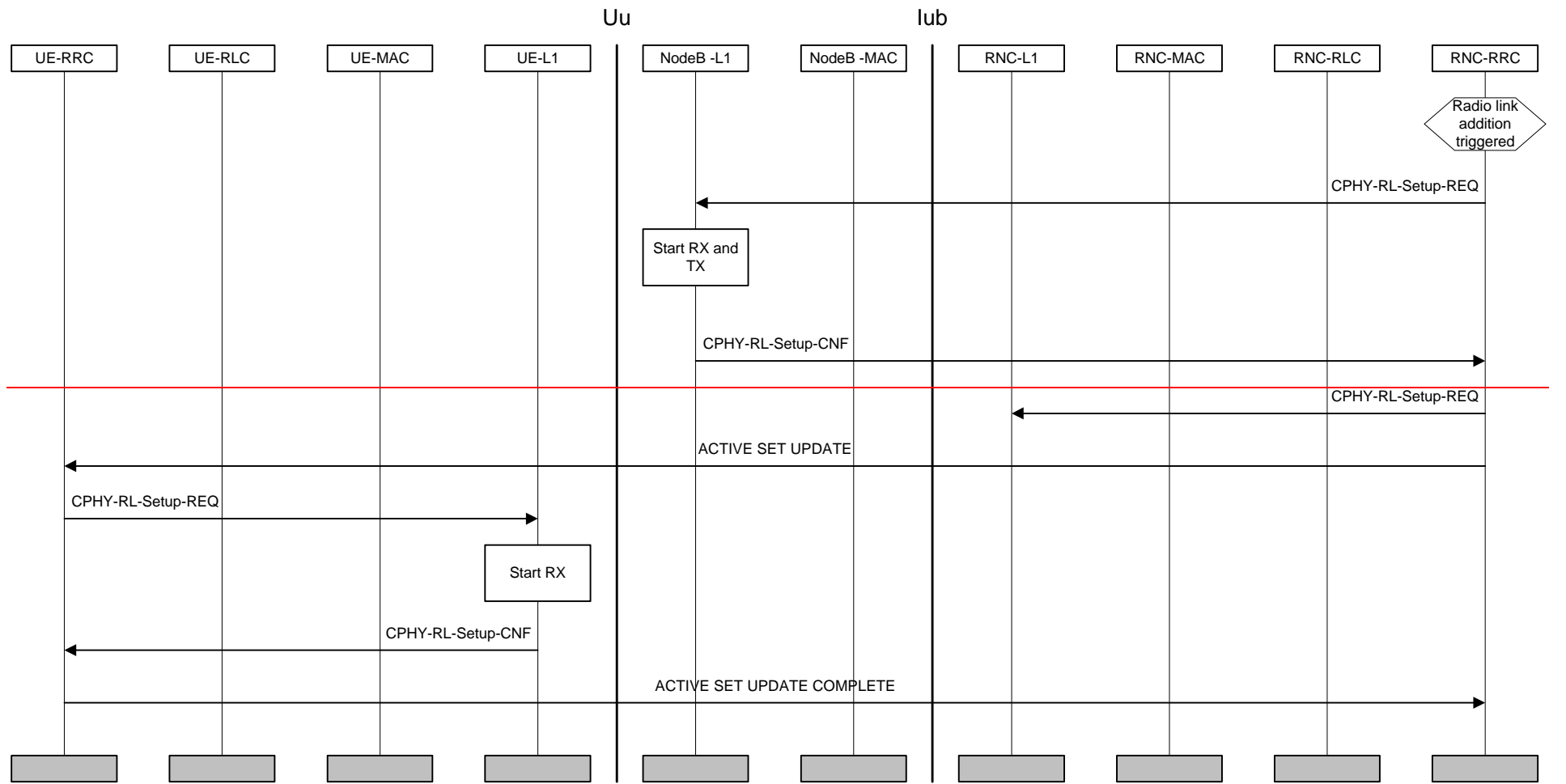
Figure 27: Radio Link Addition
