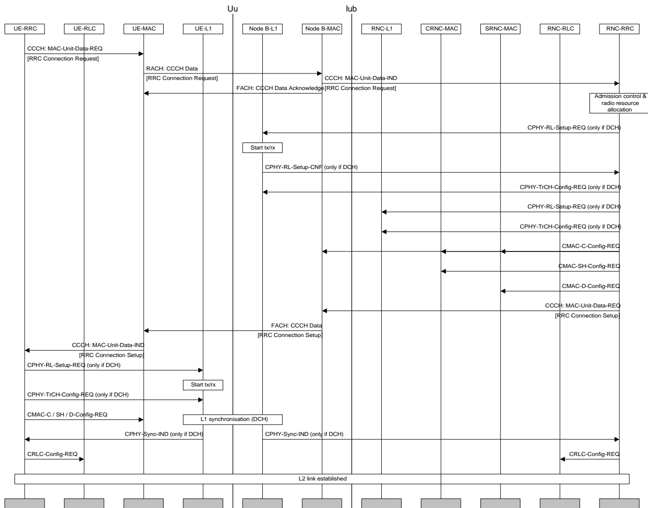
Figure 36: RRC connection establishment with common channel termination case C
