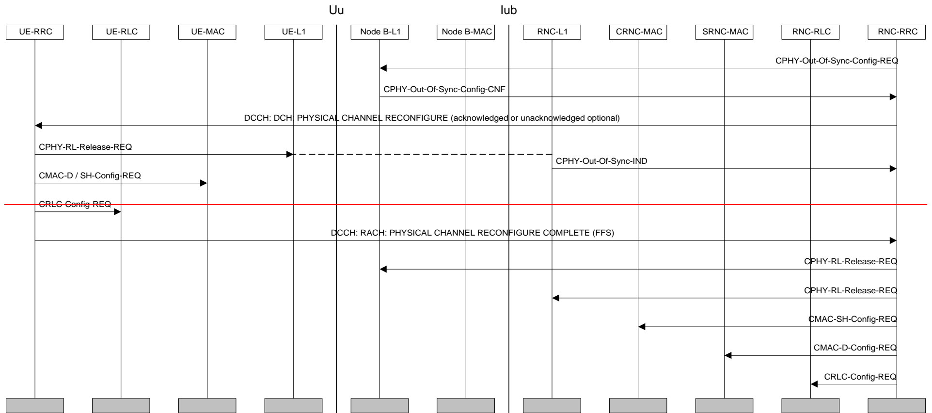
Figure 20: UE-terminated DCH Release
