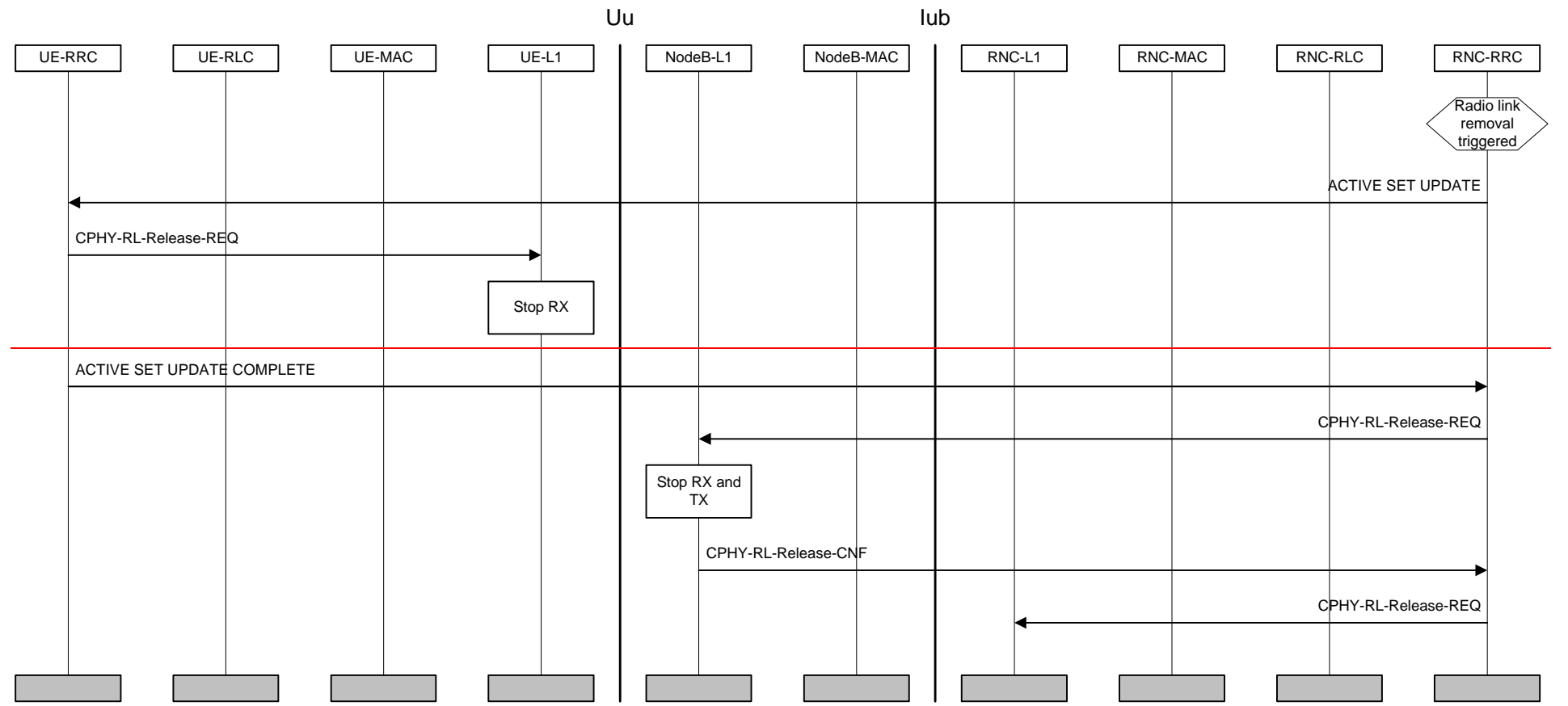
Figure 28: Radio link removal
