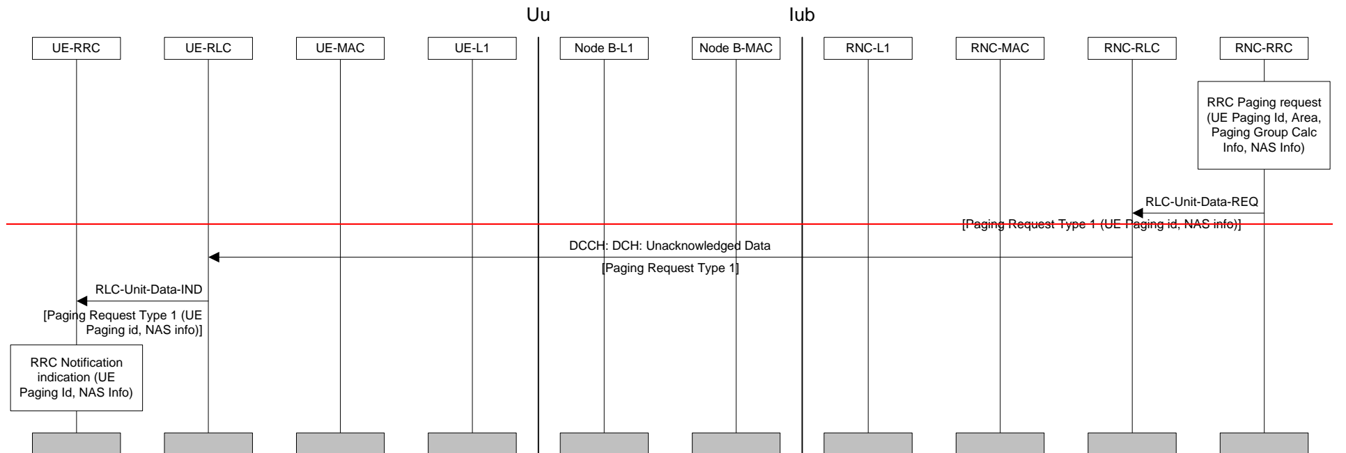
Figure 34. Example sequence of CN initiated paging request using DCCH
