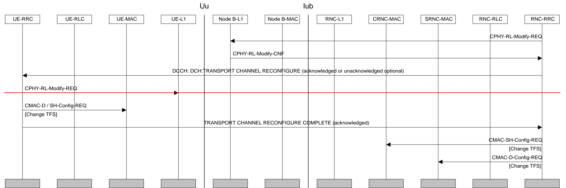
Figure 17: Unsyncronised Transport Format Set Reconfiguration
