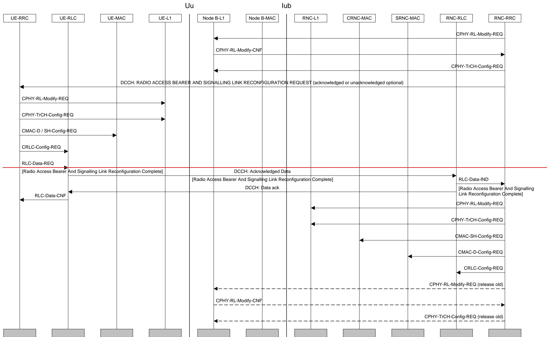
Figure 16: Unsynchronised Radio Access Bearer Reconfiguration
