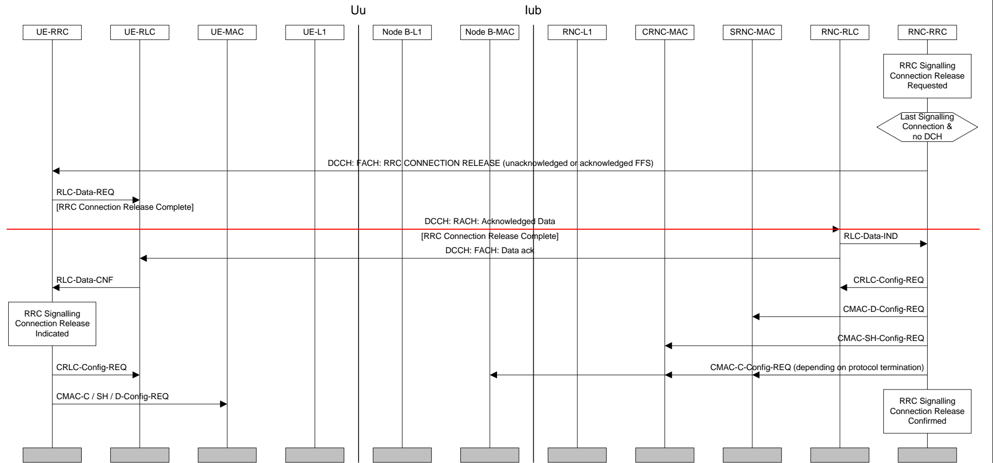
Figure 10: RRC Connection Release without Dedicated Physical Channel
