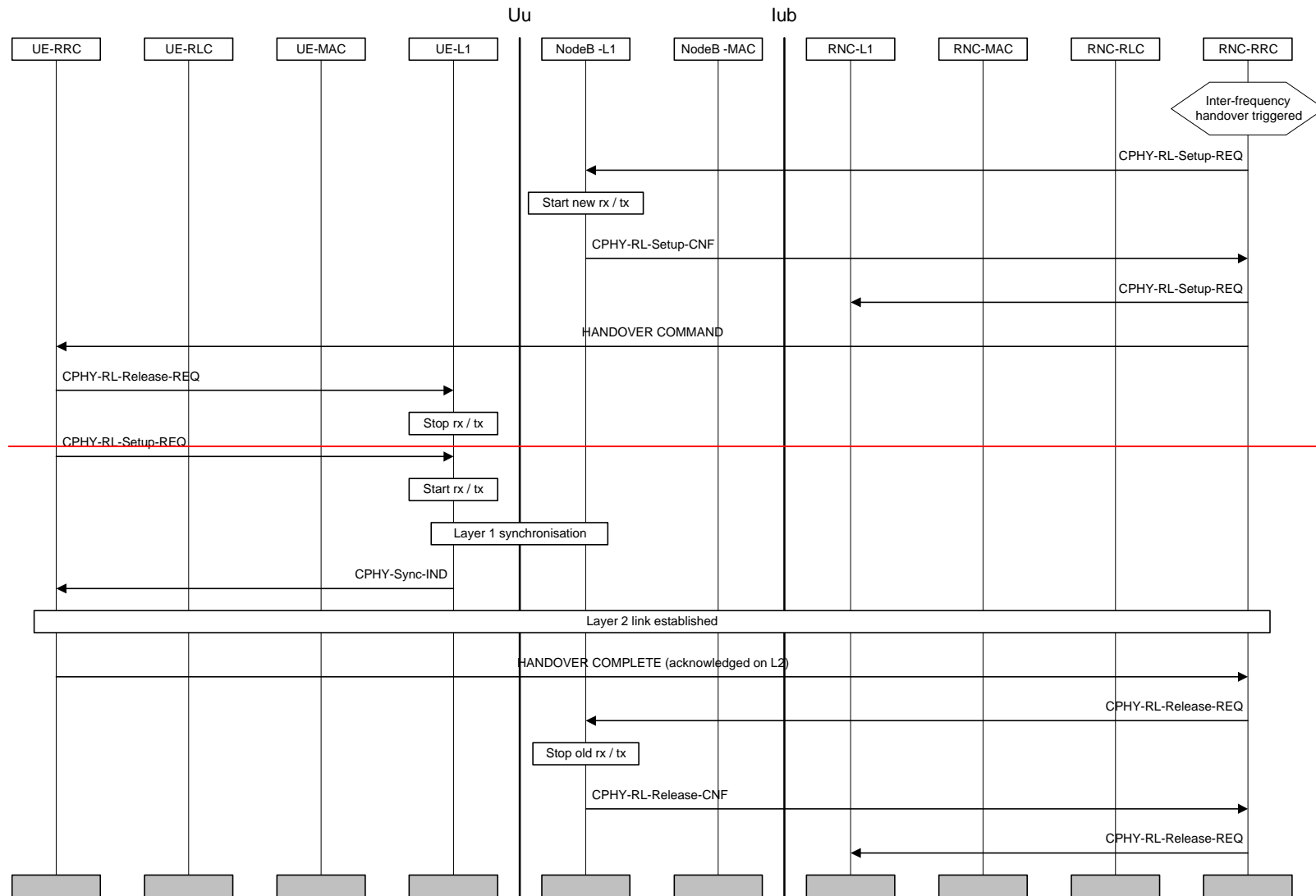
Figure 30: Hard handover
