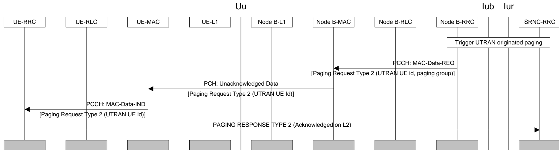
Figure 35. Example sequence for UTRAN initiated paging request with paging response
