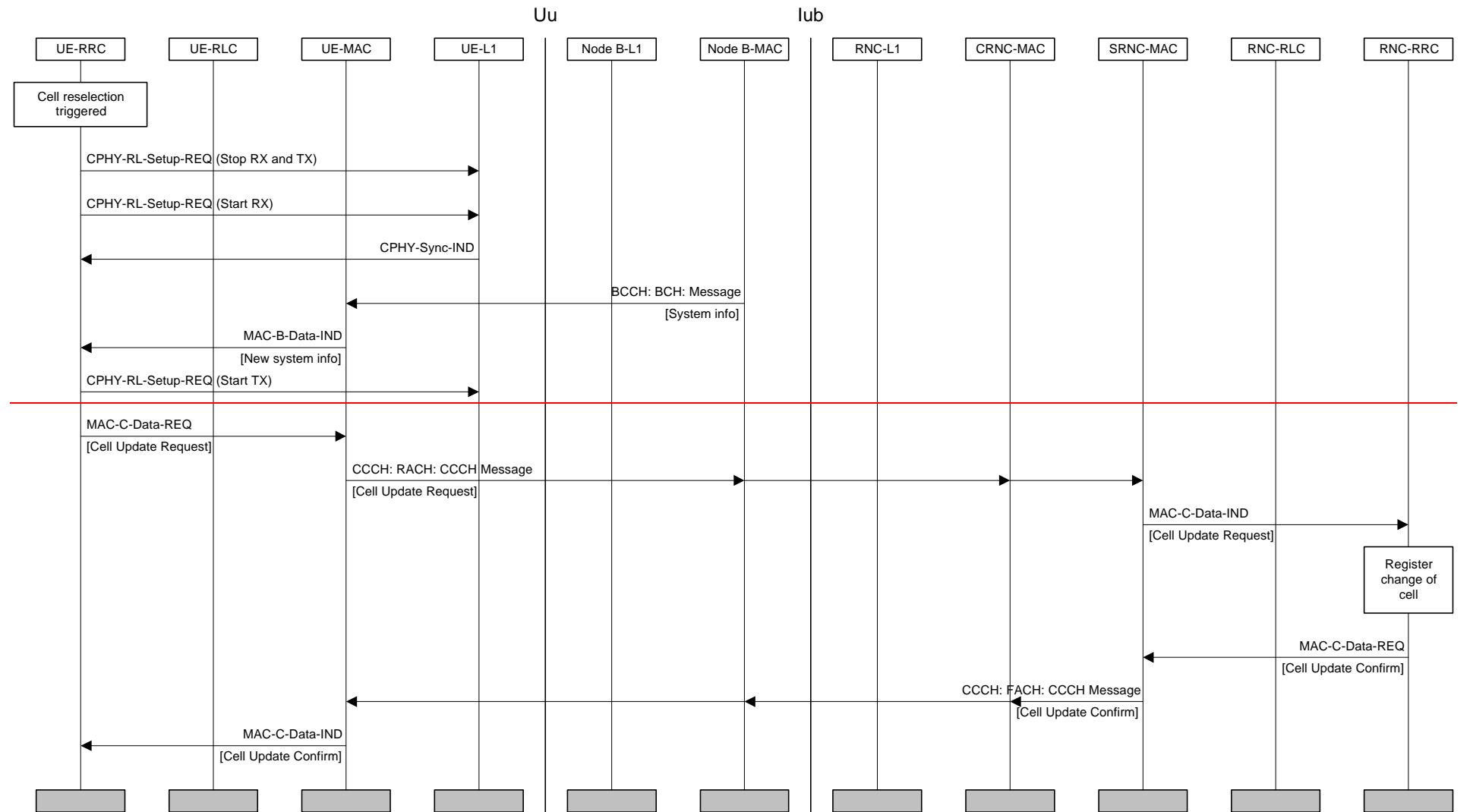
Figure 25: Cell update procedure
