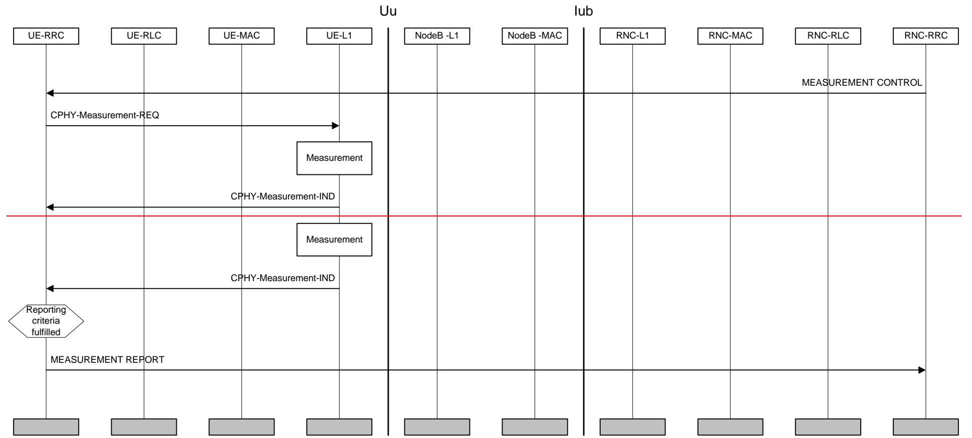
Figure 24: Handover measurement reporting
