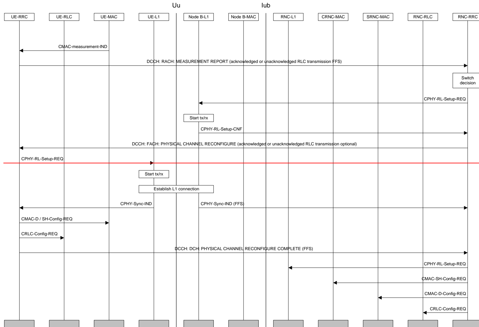
Figure 18: UE-Originated DCH Activation
