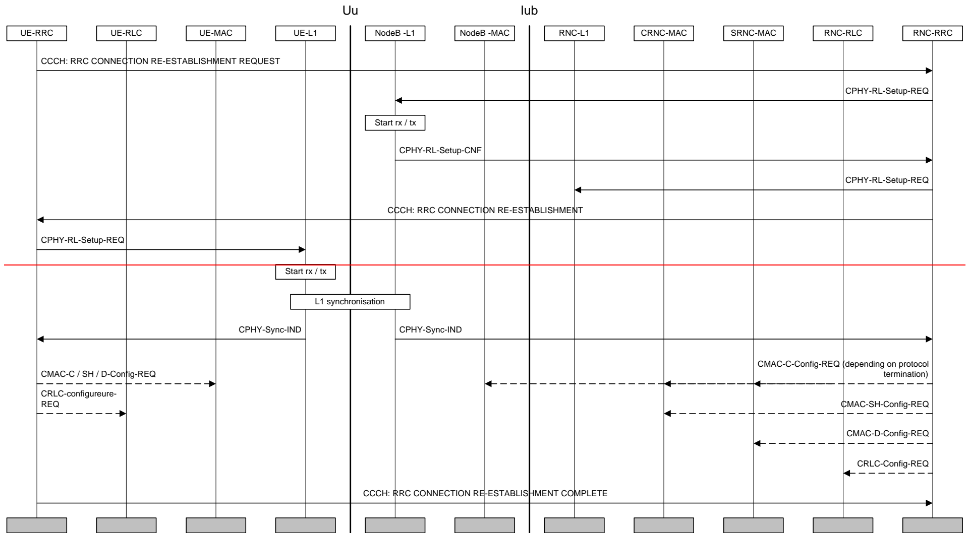
Figure 31: RRC connection re-establishment
