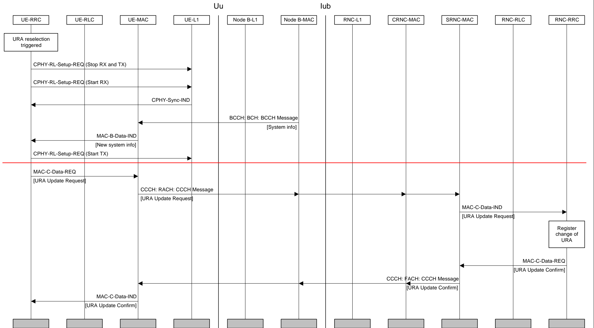
Figure 26: URA update procedure
