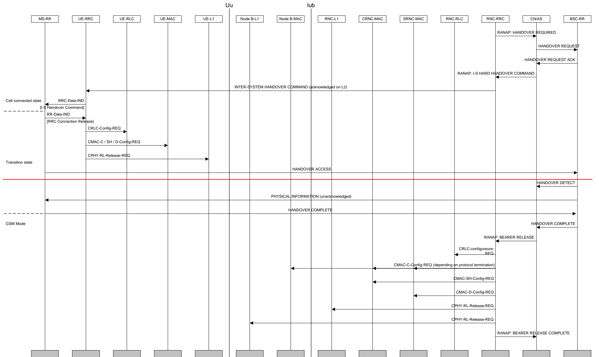
Figure 33: UTS to GSM inter-system handover
