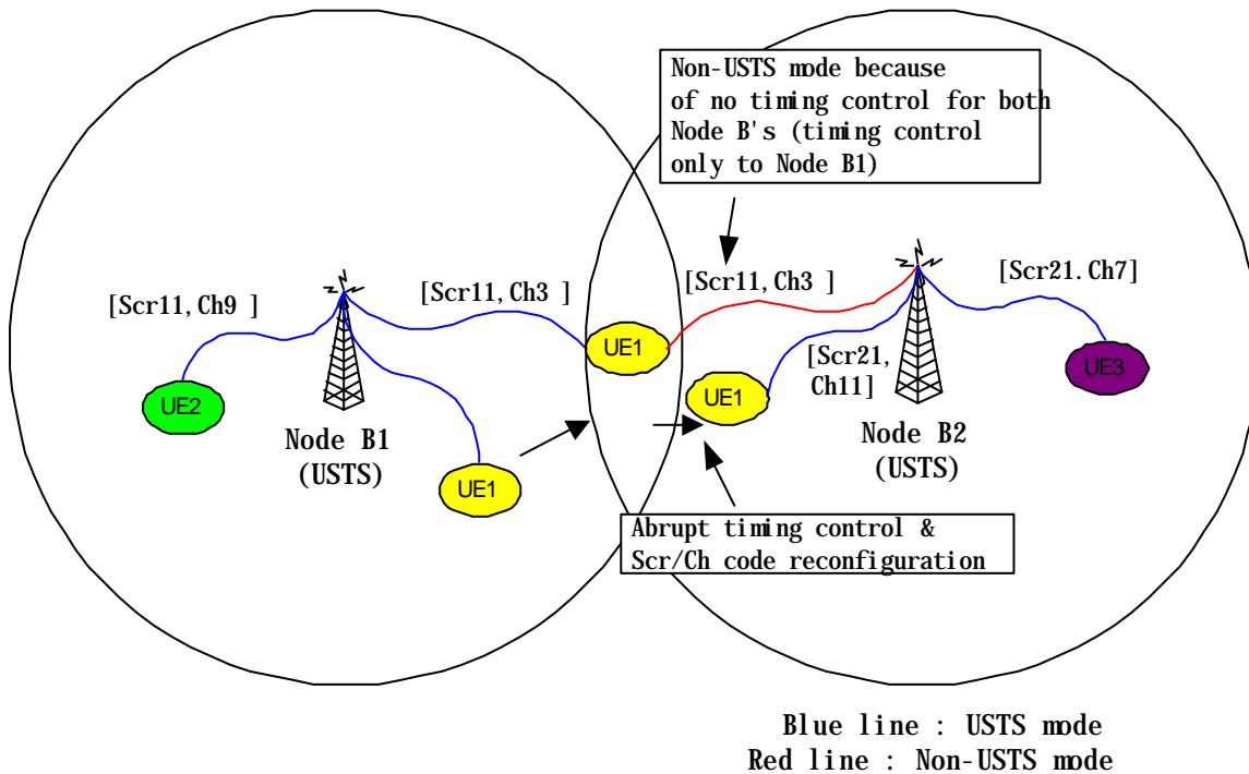
Figure 4.43 Two-way soft handover procedure for Candidate 3 .
