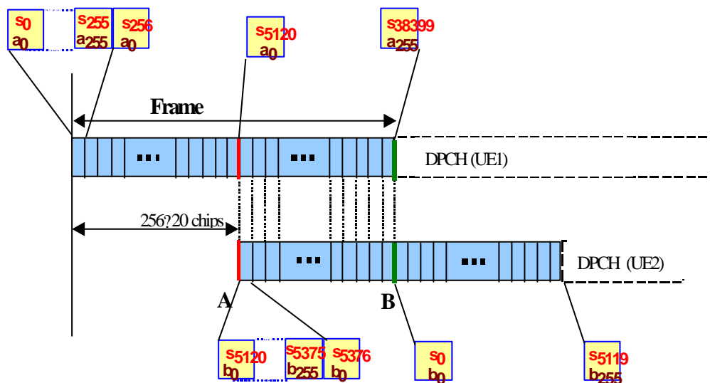
Figure 4.32 Timing at Node B and usage of scrambling and orthogonal codes in case of two UEs (a,b : channelisation codes, s : scrambling code, SF = 256)
