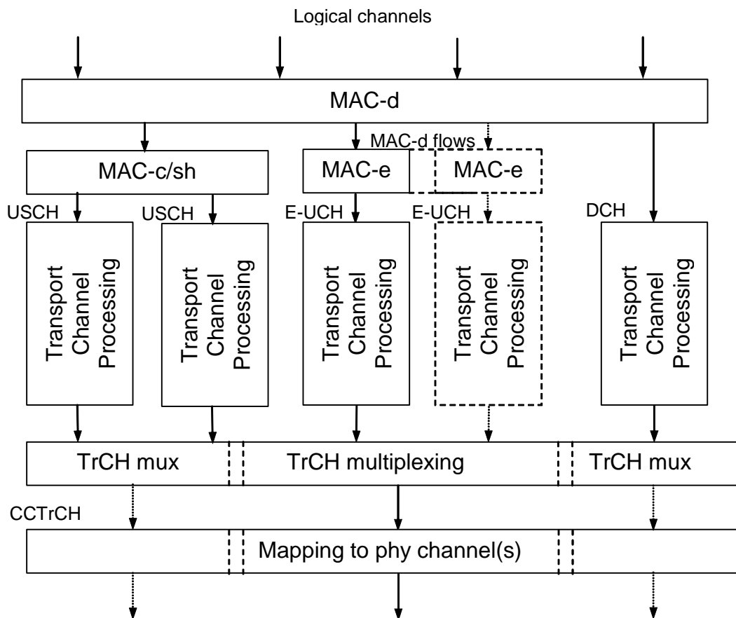
Figure 7.1.1.1: Simplified illustration of possible transport channel structures(UE side).
