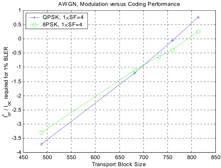
Figure 8.1.6.1.5: 8-PSK vs: QPSK at the same data rate and using equal code resources, AWGN
