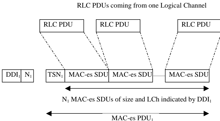
Figure 9.1.5.1: MAC-es PDU
