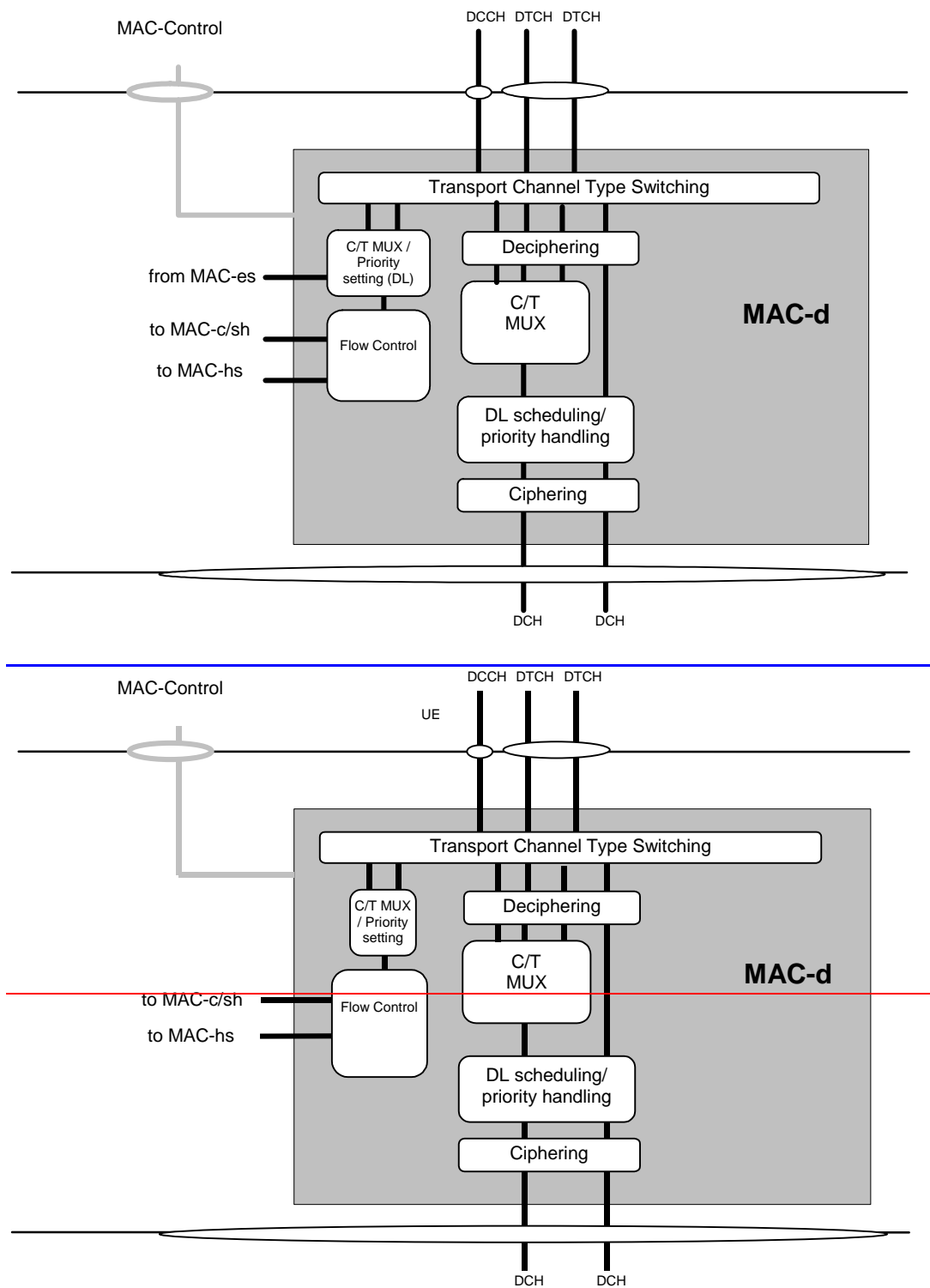
Figure 4.2.4.2.1: UTRAN side MAC architecture / MAC-d details
