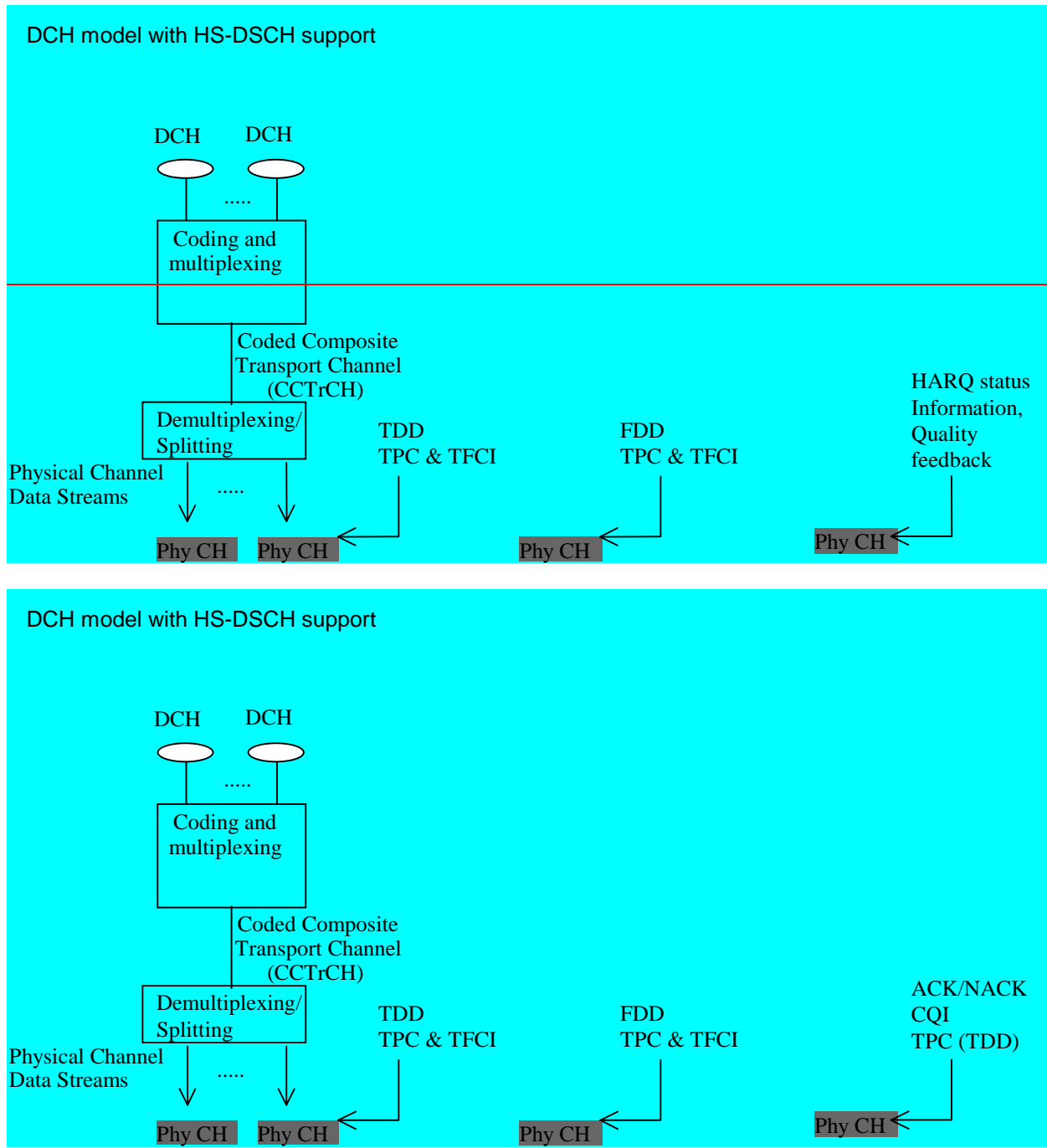
Figure 5.2.3-1: Model of the UE's Uplink physical layer
