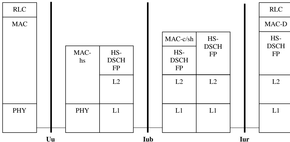
Figure 5.1-1: Protocol Architecture of HSDPA HS-DSCH , Configuration with MAC-c/sh
