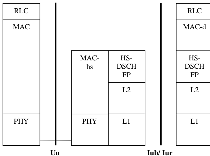
Figure 5.1-2: Protocol Architecture of HSDPA HS-DSCH , Configuration without MAC-c/sh
