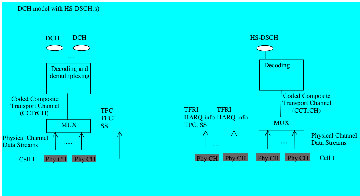
Figure 5.2.2.2-2: Model of the UE's physical layer (1.28 Mcps TDD)
