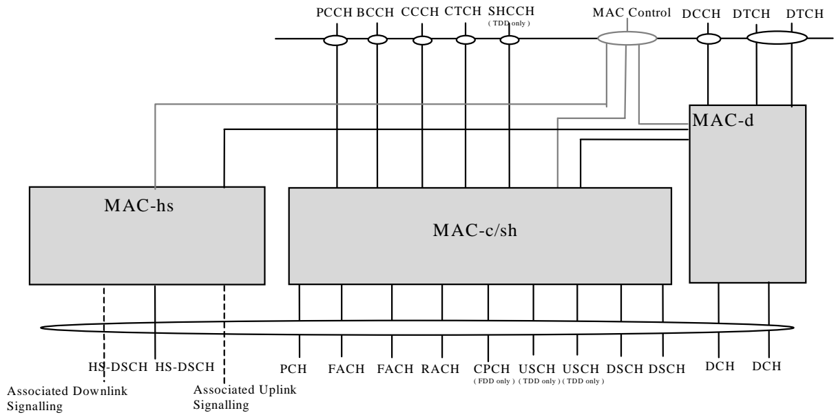
Figure 6.1.1-1: UE side MAC architecture with HSDPA/HS-DSCH
