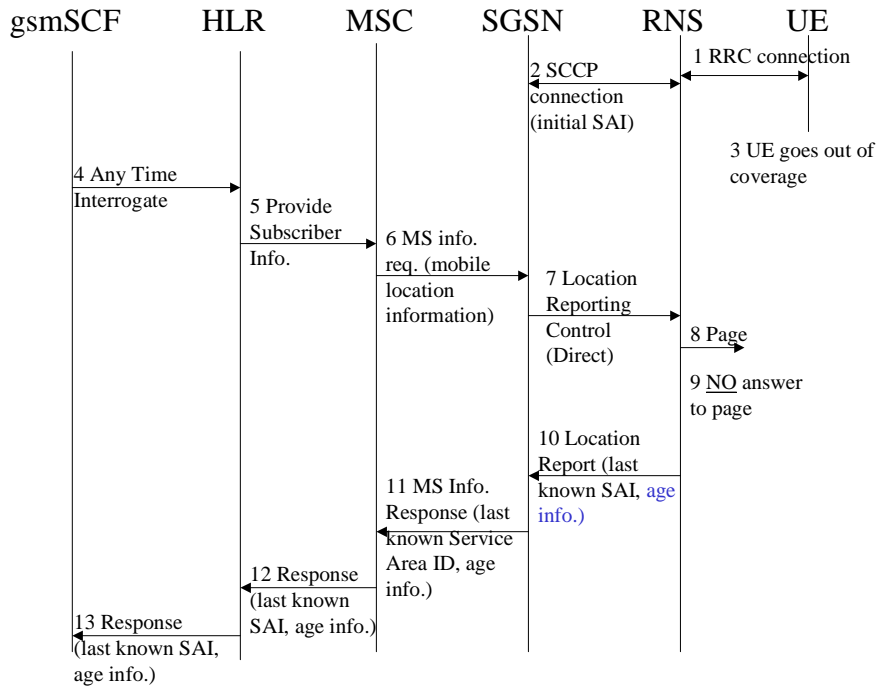
Fig 9. UMS MS attached to CS and PS domains. No Iu interface connection to MSC. Gs interface present. Iu interface connection to SGSN. MS in URA-PCH state, but out of coverage.
