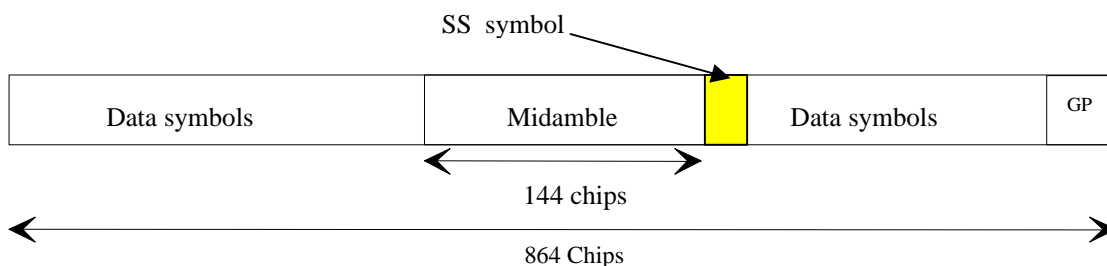
Position of SS information in a burst in downlink and uplink
