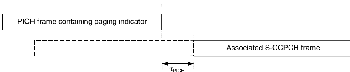
Figure 28: Timing relation between PICH frame and associated S-CCPCH frame
