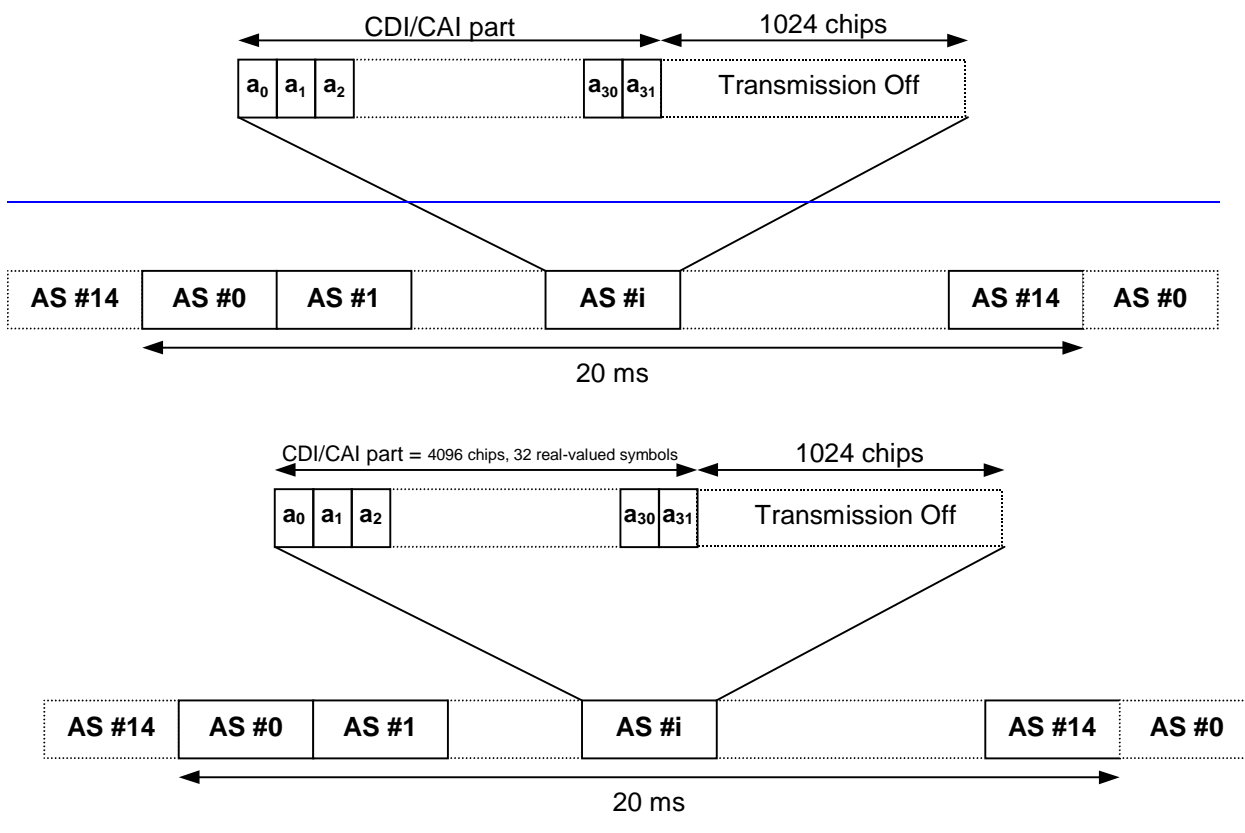
Figure 23: Structure of CD/CA Indicator Channel (CD/CA-ICH)
