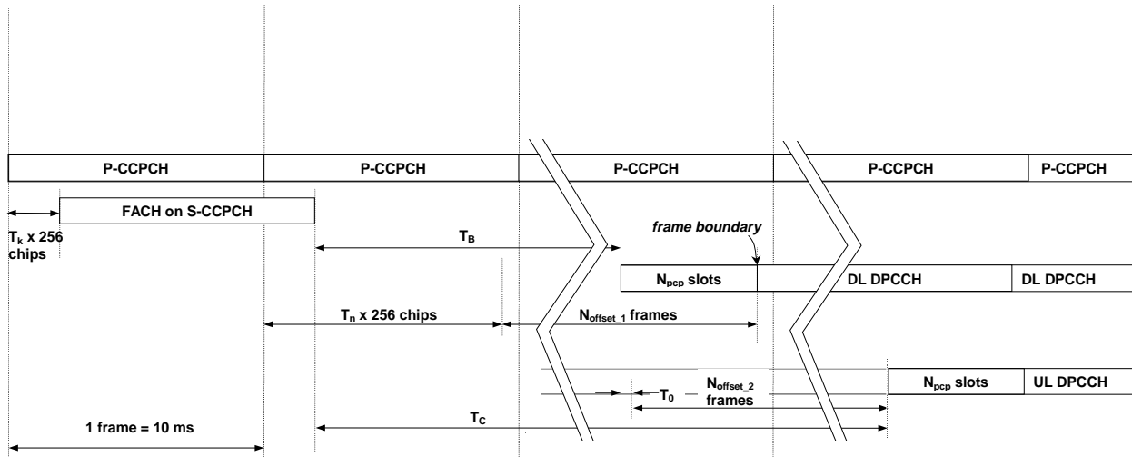
Figure 32: Timing for initialisation of DCH (UE side).
