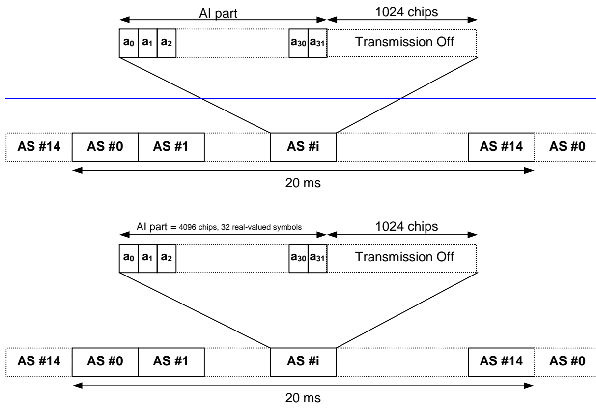
Figure 21: Structure of Acquisition Indicator Channel (AICH)
