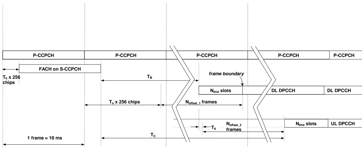
Figure 32: Timing for initialisation of DCH.
