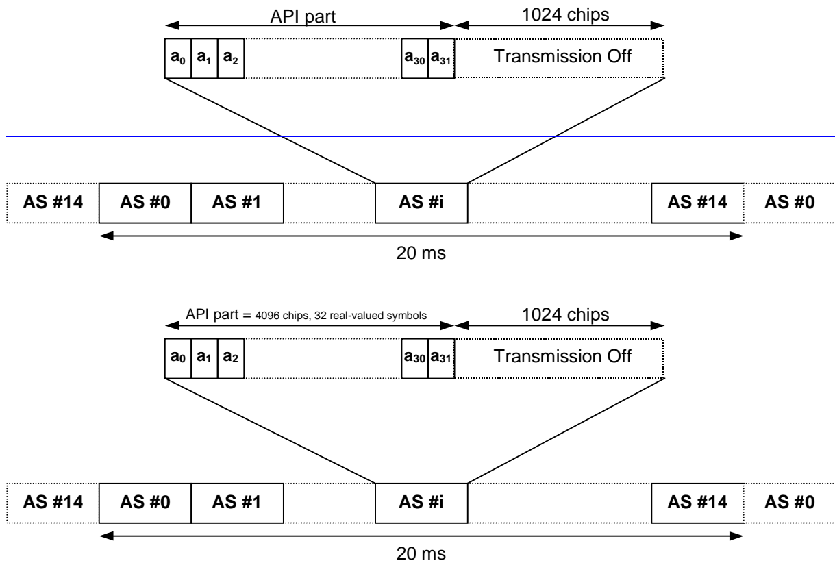
Figure 22: Structure of AP Acquisition Indicator Channel (AP-AICH)
