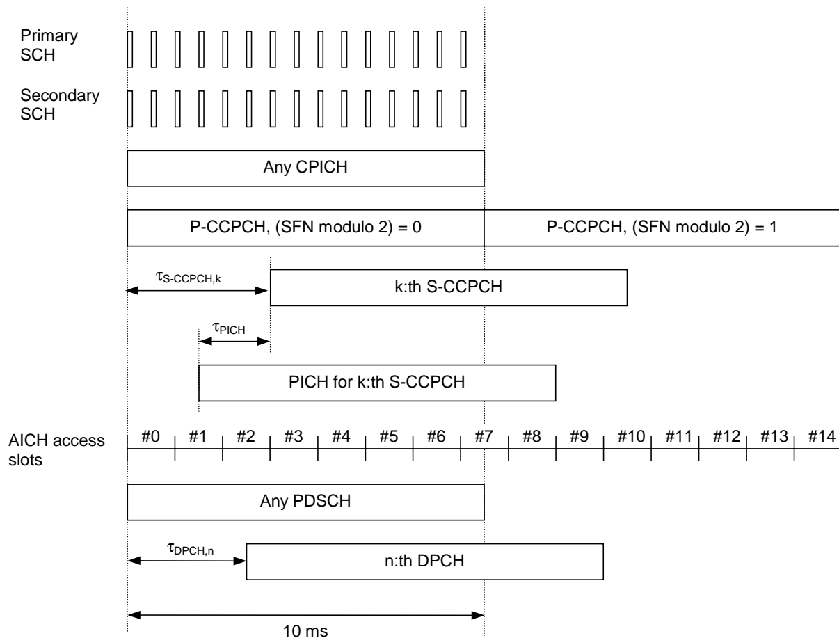
Figure 27: Frame timing and access slot timing of downlink physical channels
