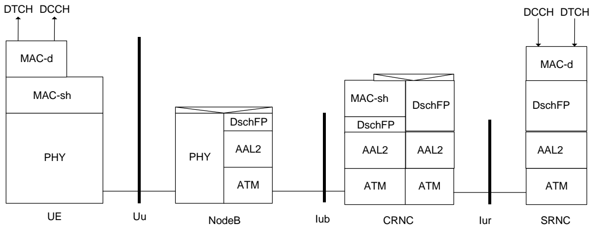
Figure 17. DSCH: Separate Controlling and Serving RNC
