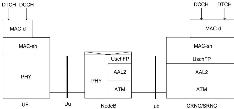
Figure 1. USCH Co-incident Controlling and Serving RNC
