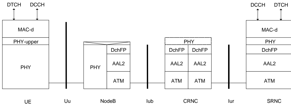
Figure 15. DCH: Separate Controlling and Serving RNC
