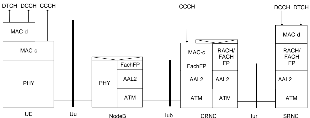
Figure 13. FACH: Separate Controlling and Serving RNC
