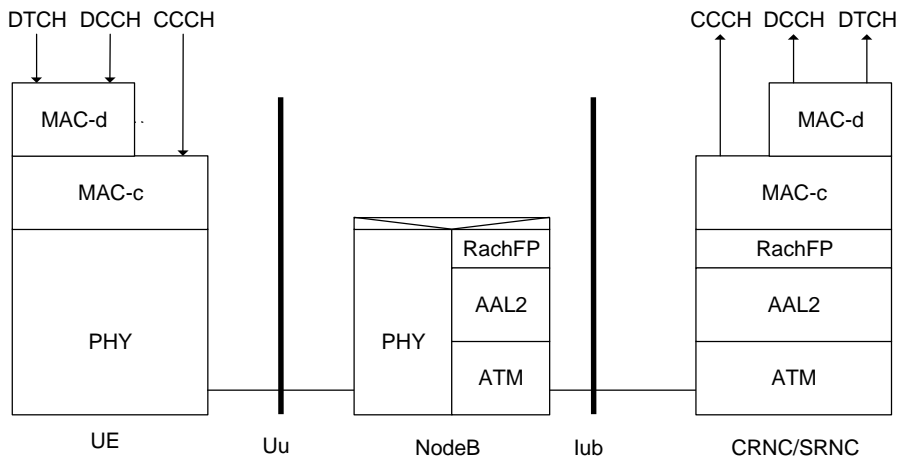
Figure 10. RACH: Coincident Controlling and Serving RNC
