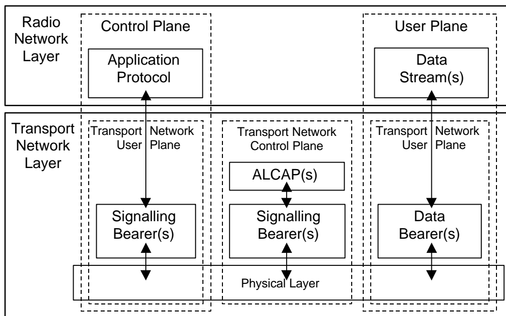
Figure 9. General Protocol Model for UTRAN Interfaces
