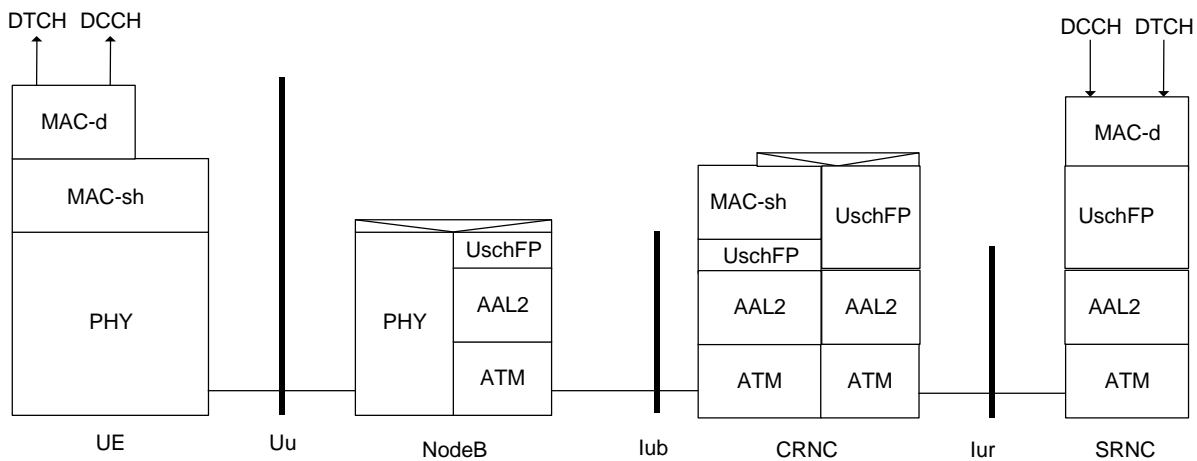
Figure 2. USCH: Separate Controlling and Serving RNC
