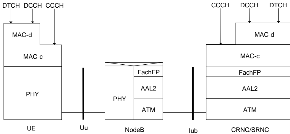
Figure 12. FACH Co-incident Controlling and Serving RNC
