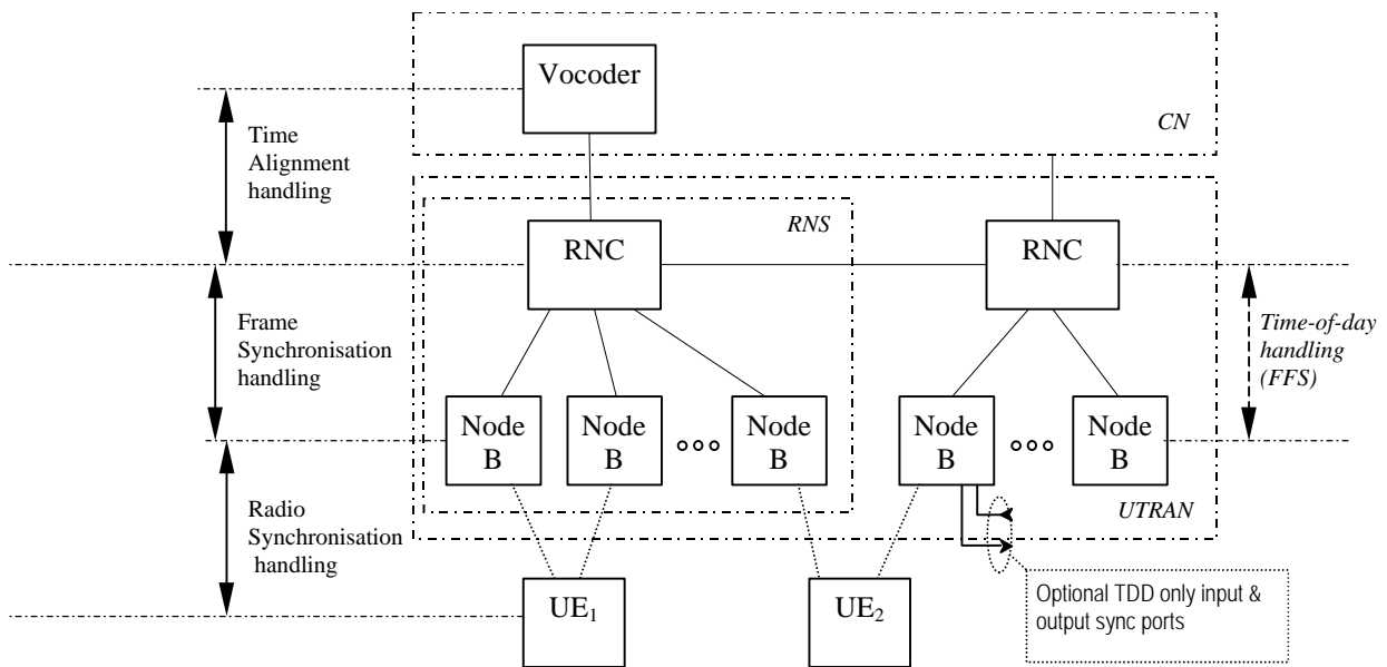
Figure 7. Synchronisation issues model.
