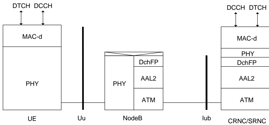
Figure 14. DCH: Co-incident Controlling and Serving RNC
