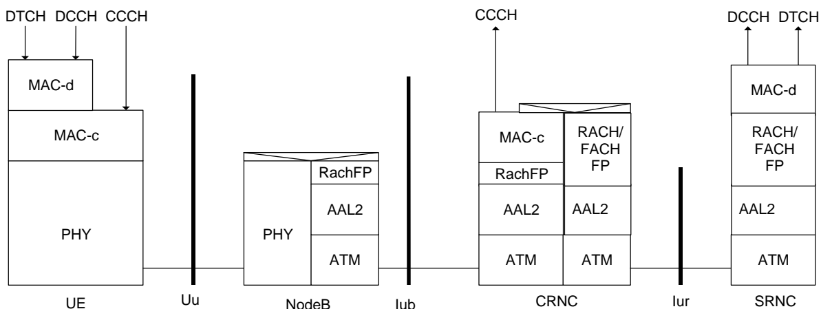
Figure 11. RACH: Separate Controlling and Serving RNC
