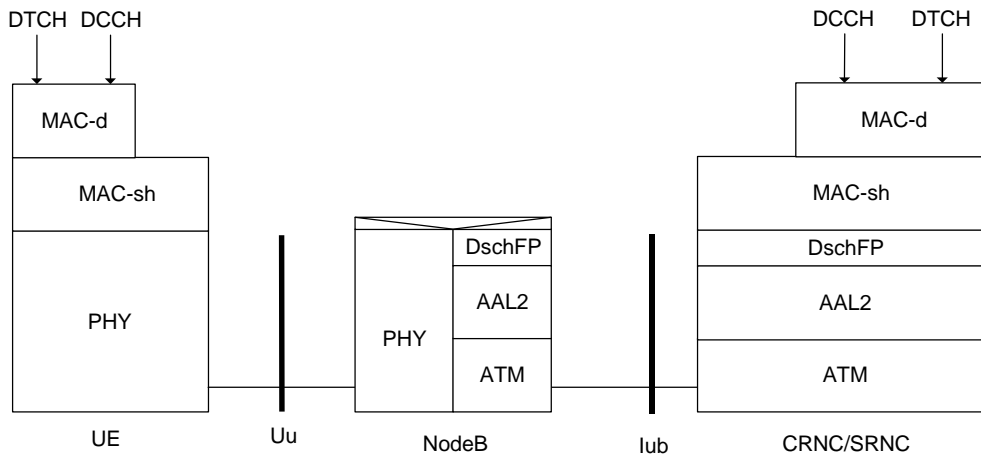
Figure 16. DSCH Co-incident Controlling and Serving RNC
