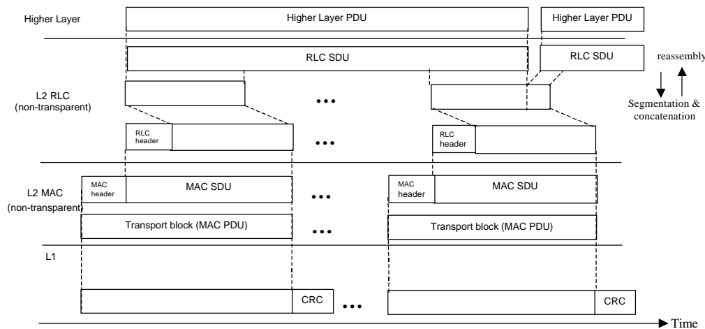
Figure 3. Data flow for a service using a non-transparent RLC and non-transparent MAC, see sections 5.x.2.1.4.1-2 for further definitions of the MAC and RLC services and functionality.
