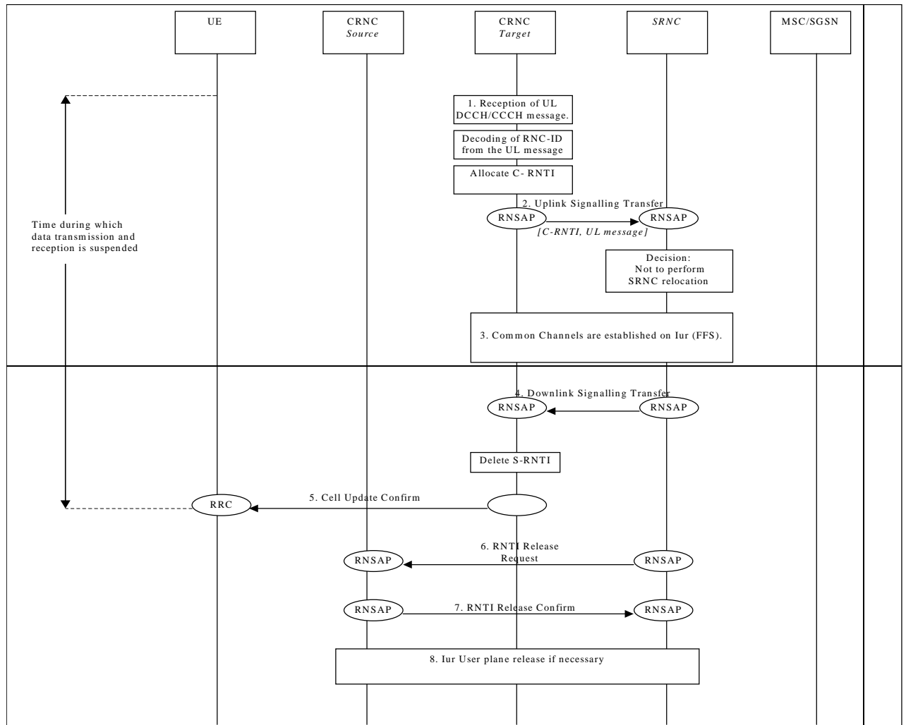
Example of Inter-RNS URA update via Iur
