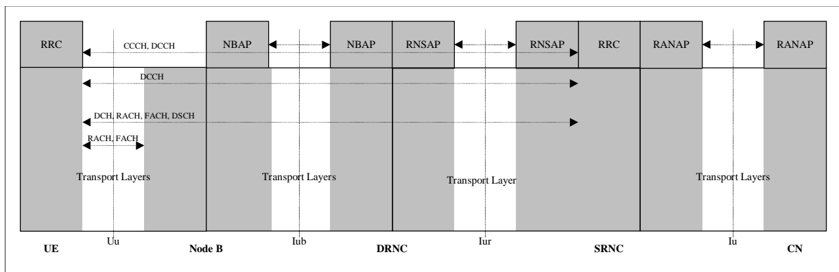
Figure 3: UTRAN and UE control plane protocol architecture (connected mode)
