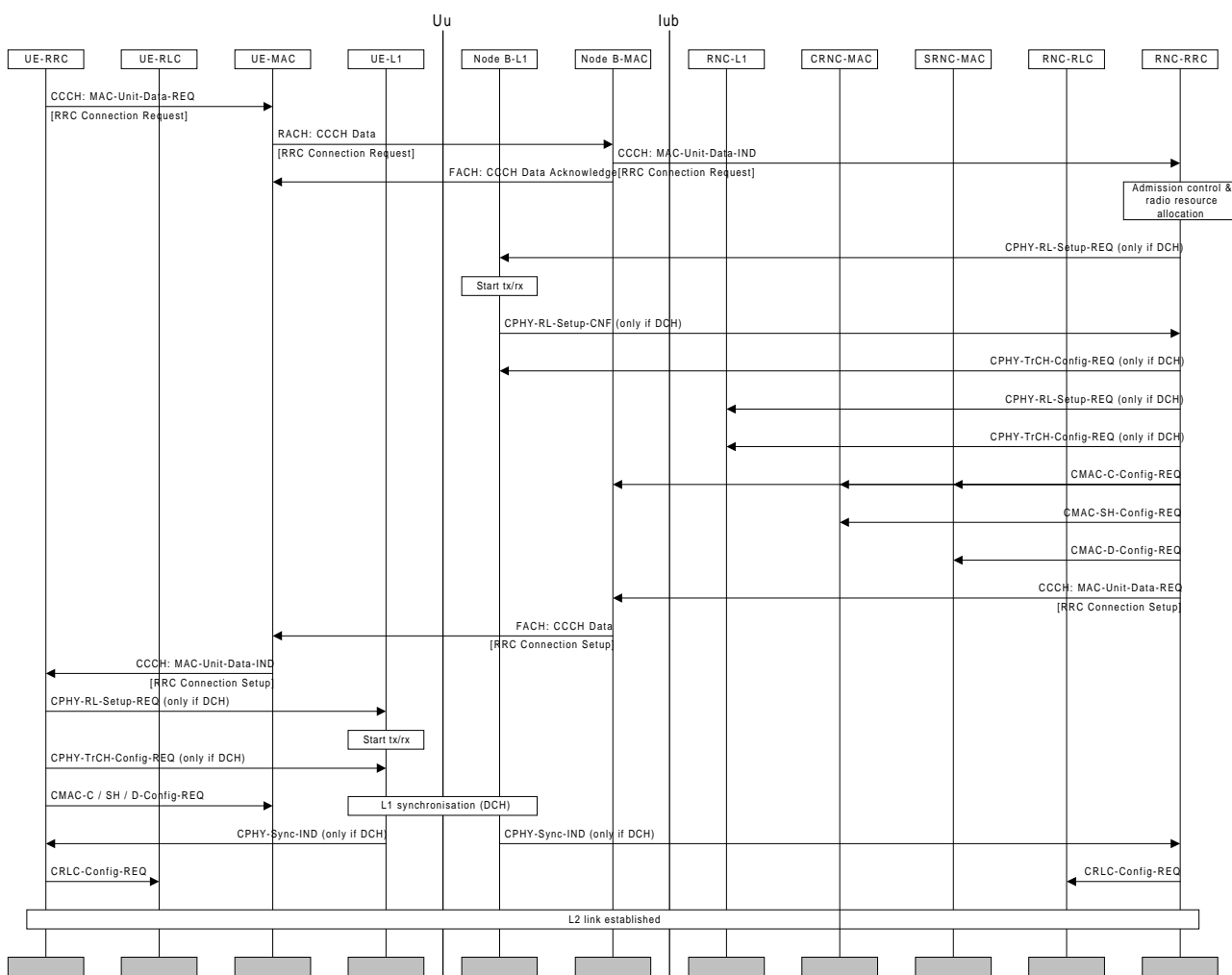
Figure Error! Unknown switch argument.: RRC connection establishment with common channel termination case C
