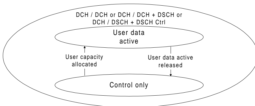
Figure Error! Unknown switch argument.: Substates in DCH / DCH, DCH / DCH + DSCH and DCH / DSCH + DSCH Ctrl substates
