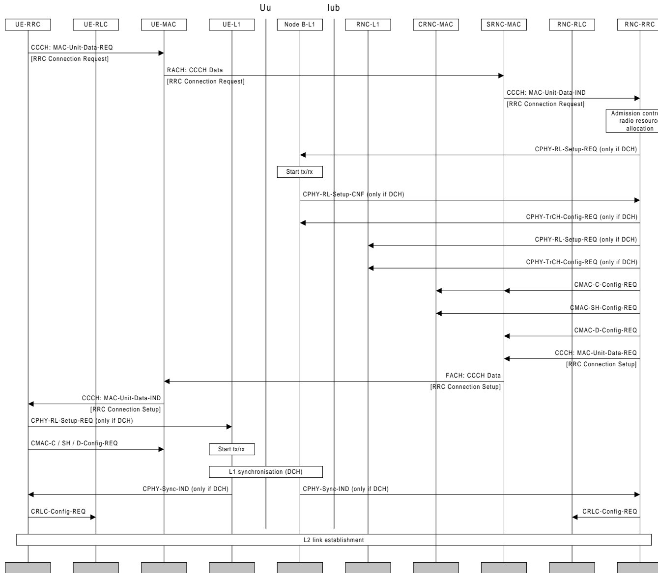
Figure Error! Unknown switch argument.. RRC connection establishment with common channel termination case A
