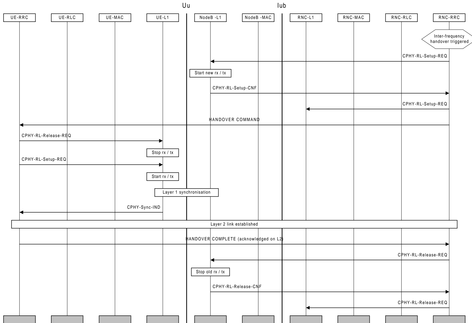
Figure Error! Unknown switch argument.: Hard handover
