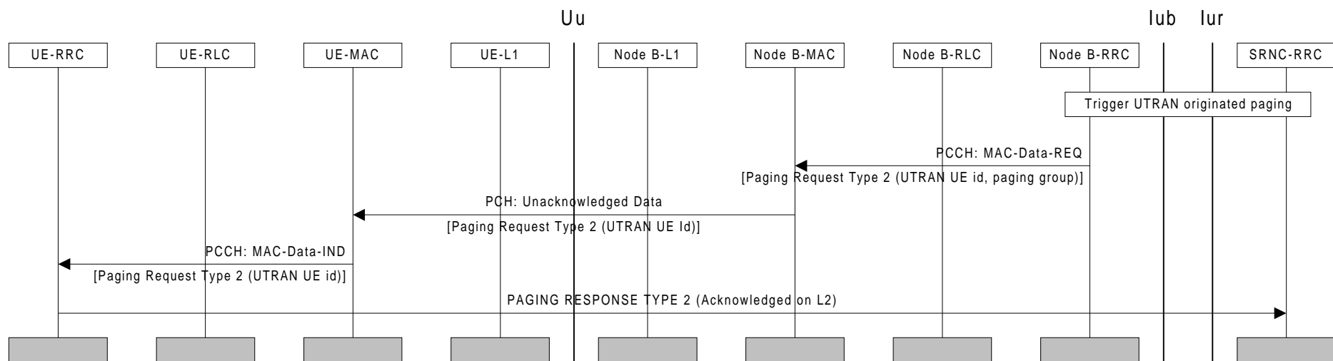
Figure Error! Unknown switch argument.. Example sequence for UTRAN initiated paging request with paging response
