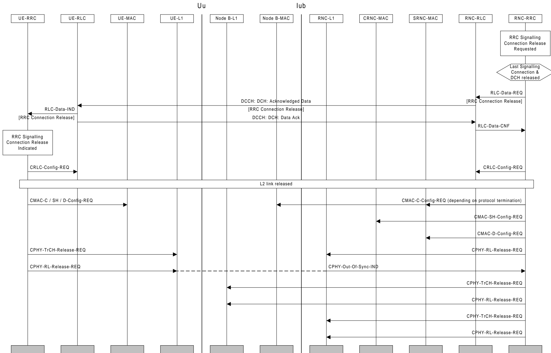
Figure Error! Unknown switch argument.. RRC Connection Release from Dedicated Physical Channel
