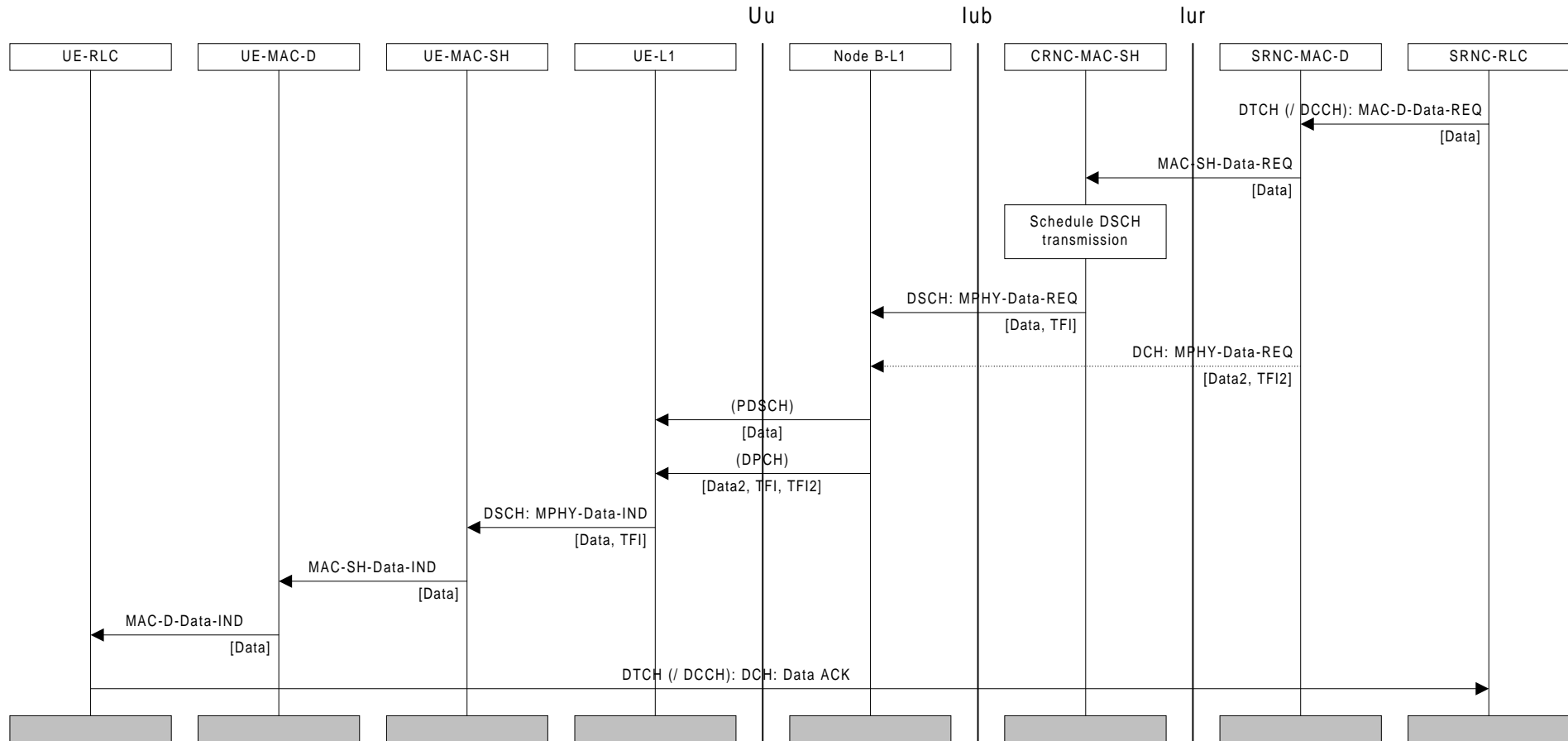
Figure Error! Unknown switch argument.: Example of acknowledged-mode data transmission on DSCH
