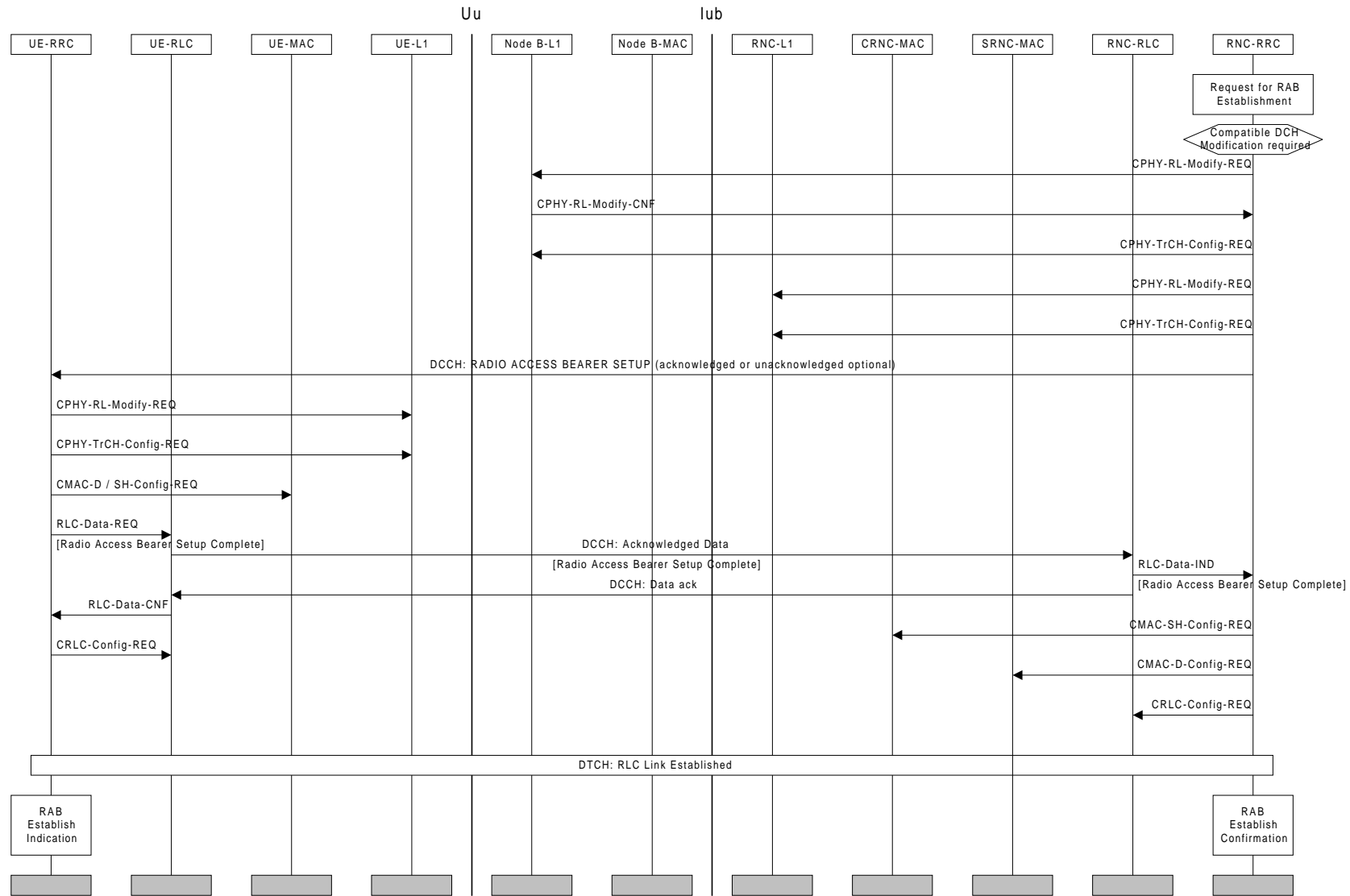
Figure Error! Unknown switch argument.: Radio Access Bearer Establishment with Unsynchronised Dedicated Physical Channel Modification
