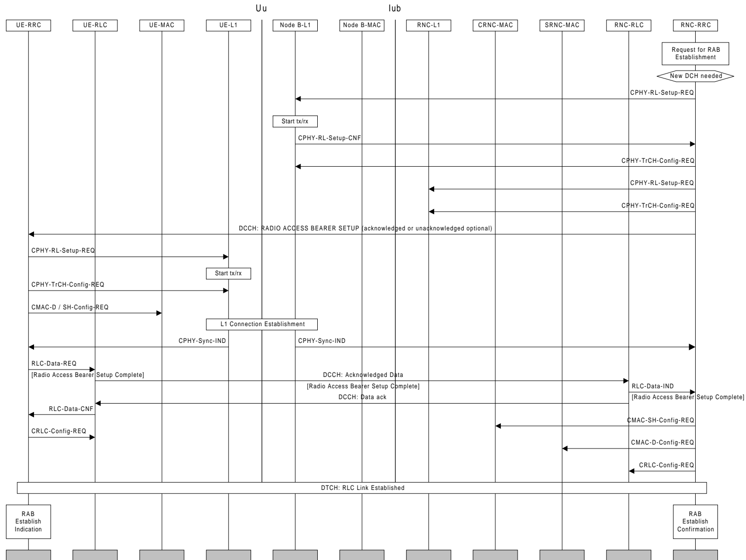
Figure Error! Unknown switch argument.: Radio Access Bearer Establishment with Dedicated Physical Channel Activation
