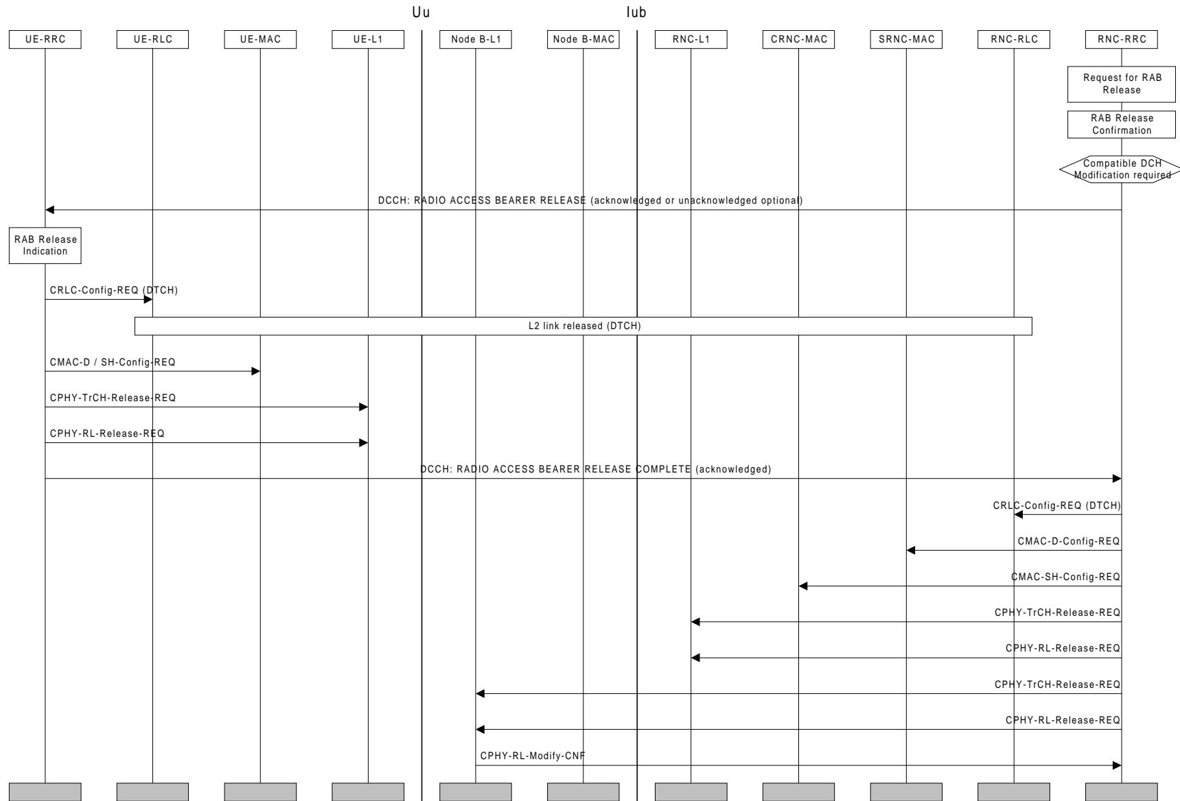
Figure Error! Unknown switch argument.: Radio Access Bearer Release with Unsynchronised Dedicated Physical Channel Modification
