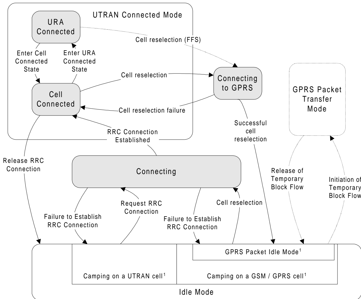
Figure Error! Unknown switch argument.: UE RRC states and State Transitions including GSM/GPRS (IP only)
