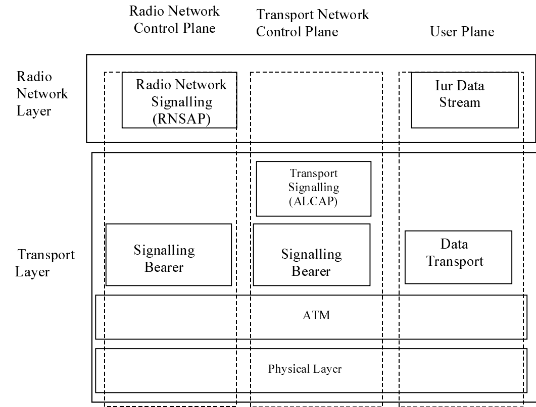
Figure 8-46-1. I ur -Interface Protocol Structure
