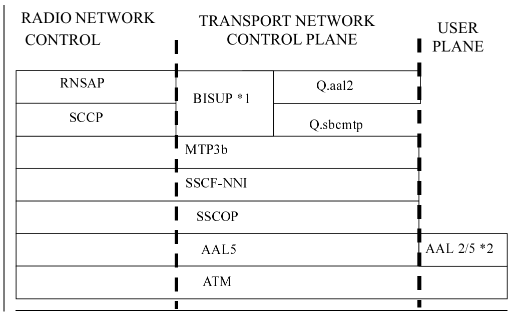
Figure-8-26-2: Iur Interface protocol Structure (TTC version)
