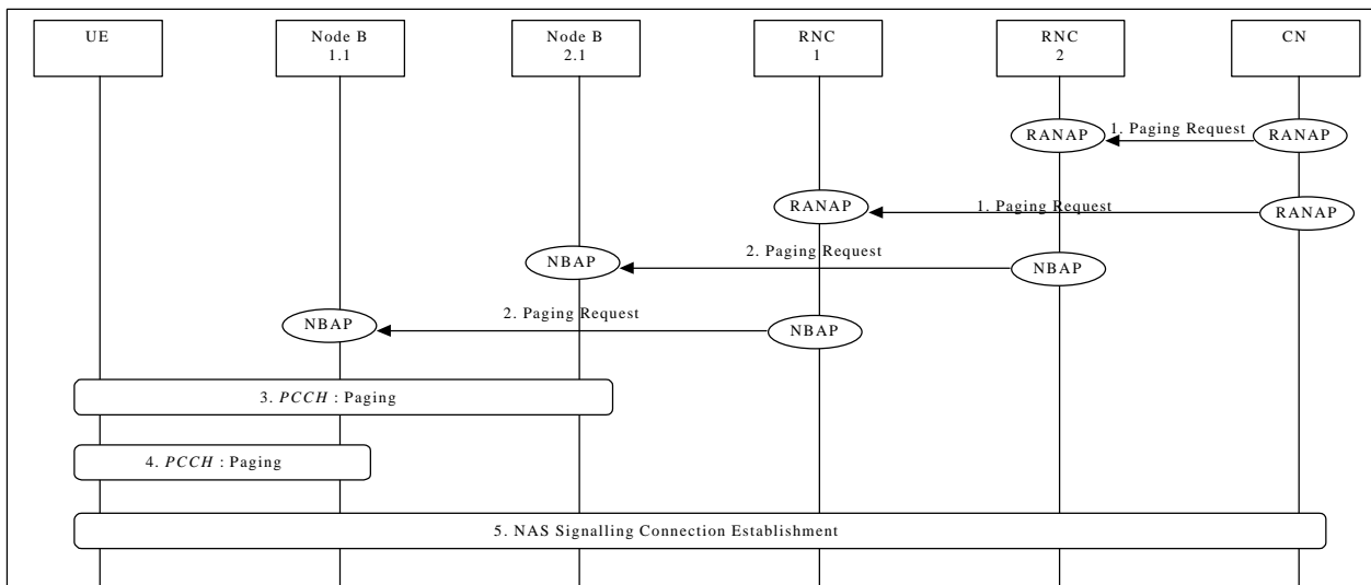
Figure 7: Paging for a UE in RRC Idle Mode
