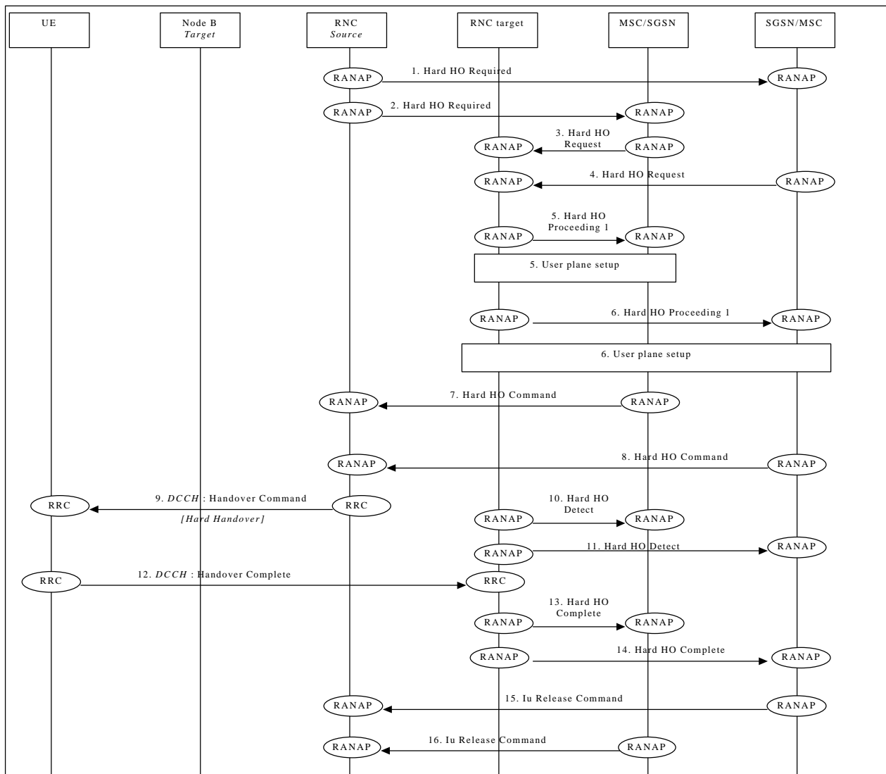
Figure 18: Inter-RNS Hard Handover with switching in the CN (UE connected to two CN nodes)
