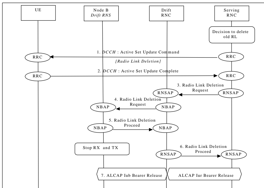
Figure 15: Soft Handover - Radio Link Deletion (Branch Deletion)
