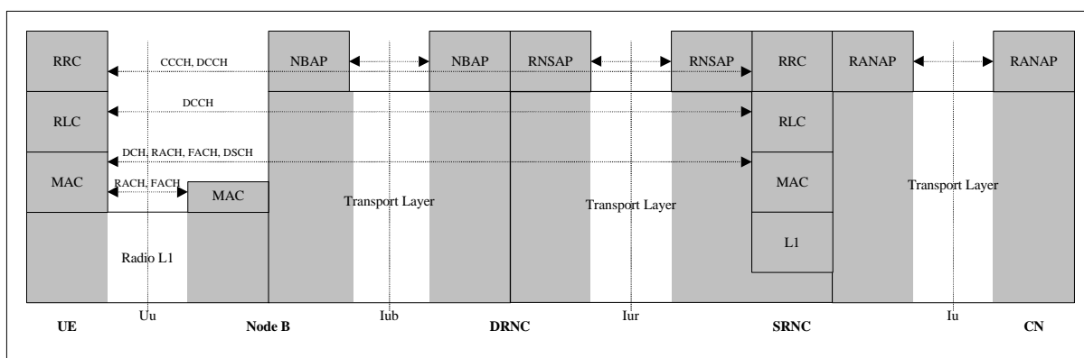
Figure 5: UTRAN and UE control plane protocol architecture (connected mode)
