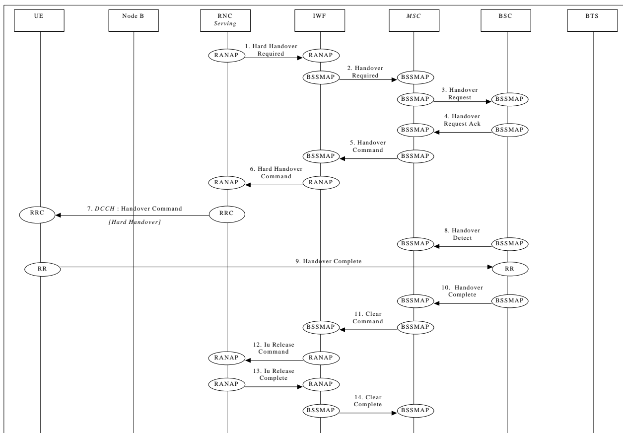
Figure 20: UTRAN ⇒ GSM/BSS handover via IWF
