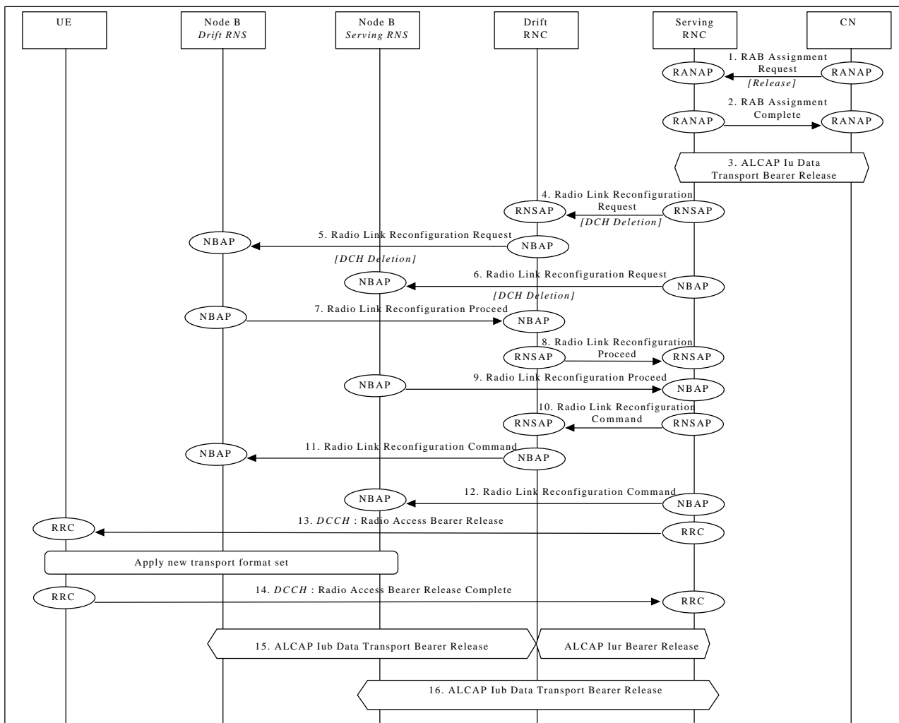
Figure 13: Radio Access Bearer Release - DCH - DCH Release
