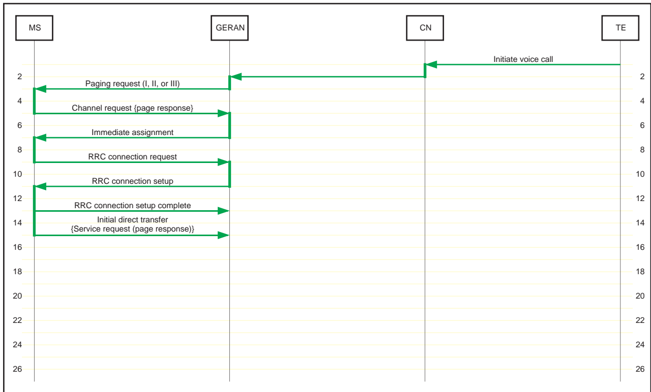
1 Figure 1: Incoming voice call – RRC Idle and CCCH
