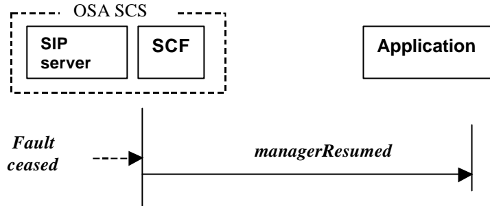
Figure 0-8 Call Flow for managerResumed()
