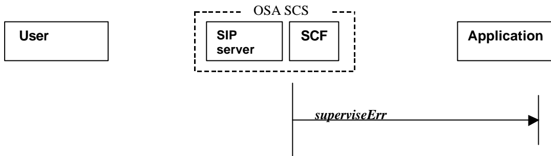
Figure 5-28: Call flow for superviseErr()
