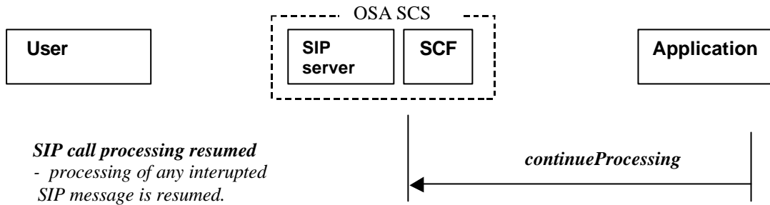
Figure 5-39: Call flow for continueProcessing()
