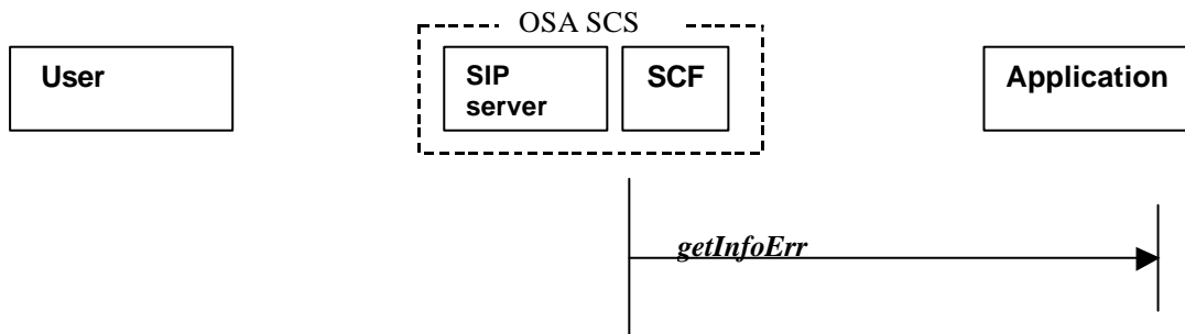
Figure 5-27: Call flow for getInfoErr()
