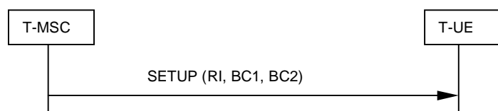
Figure 4.5: SETUP message towards the terminating UE
