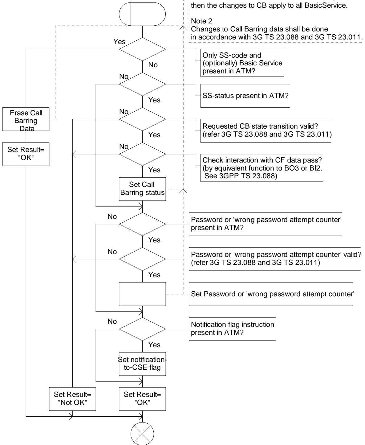
Figure 10.7: Procedure ATM_Modify_CB_Data (sheet 1)
