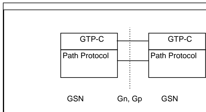
Figure 58: SignallingControl Plane - Protocol Stack
