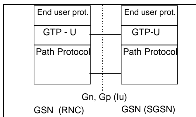
Figure 61: GTP-U - Protocol Stack (GTP-U over the lu in brackets)
