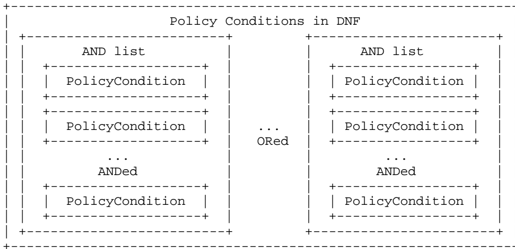
Figure Overview of Policy Conditions in DNF
