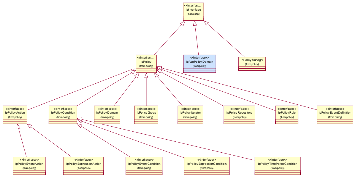
Figure: Policy Classes
