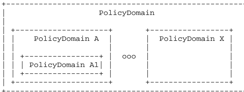
Figure Overview of the PolicyDomain class
