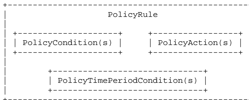
Figure Overview of the PolicyRule Class
