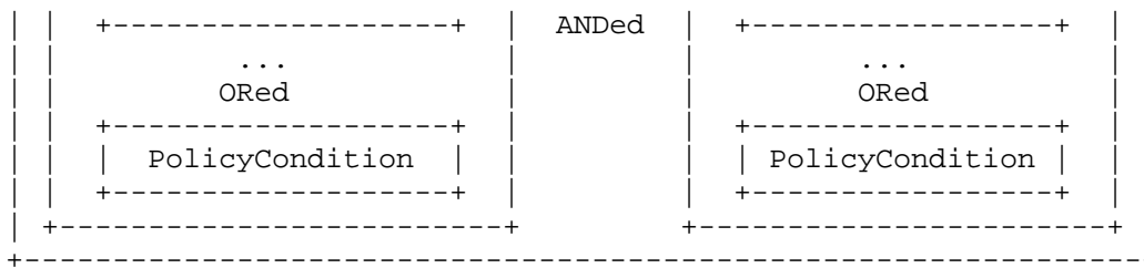
Figure 8. Overview of Policy Conditions in CNF
