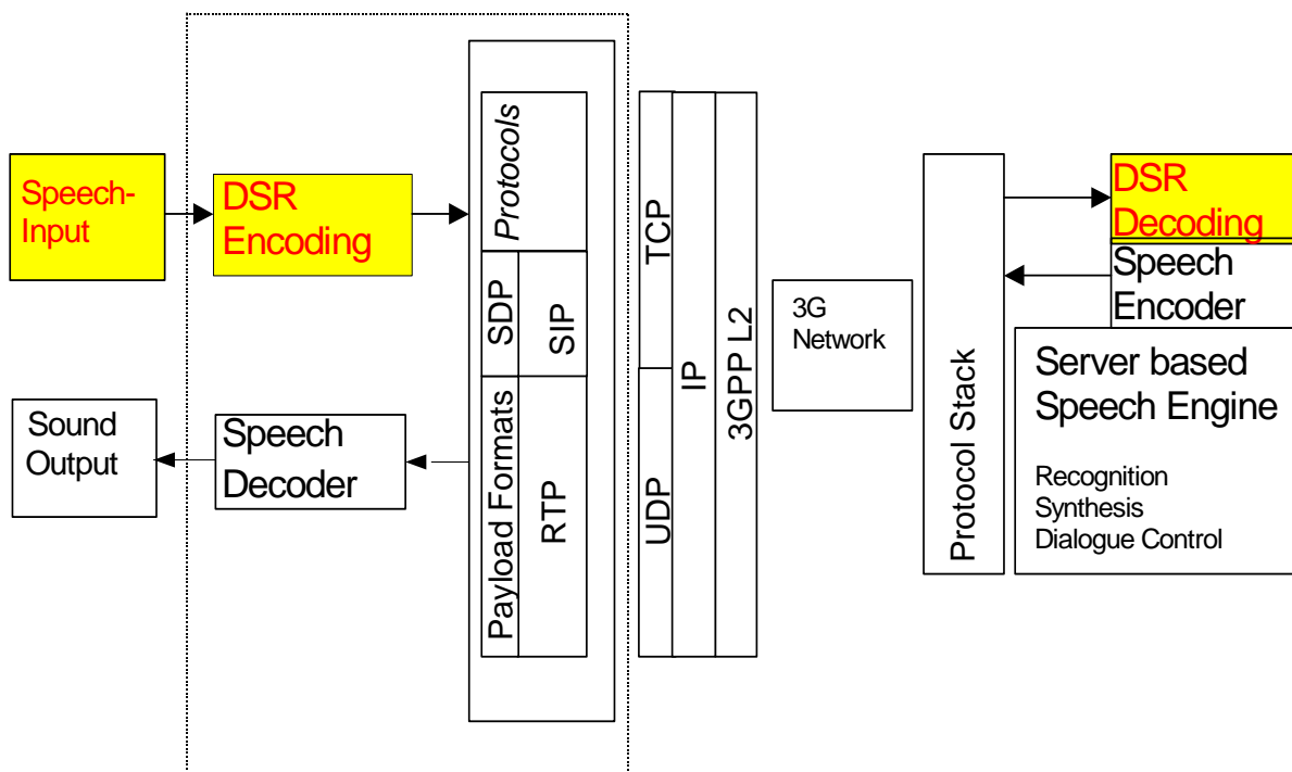
Figure 1: DSR Architecture
